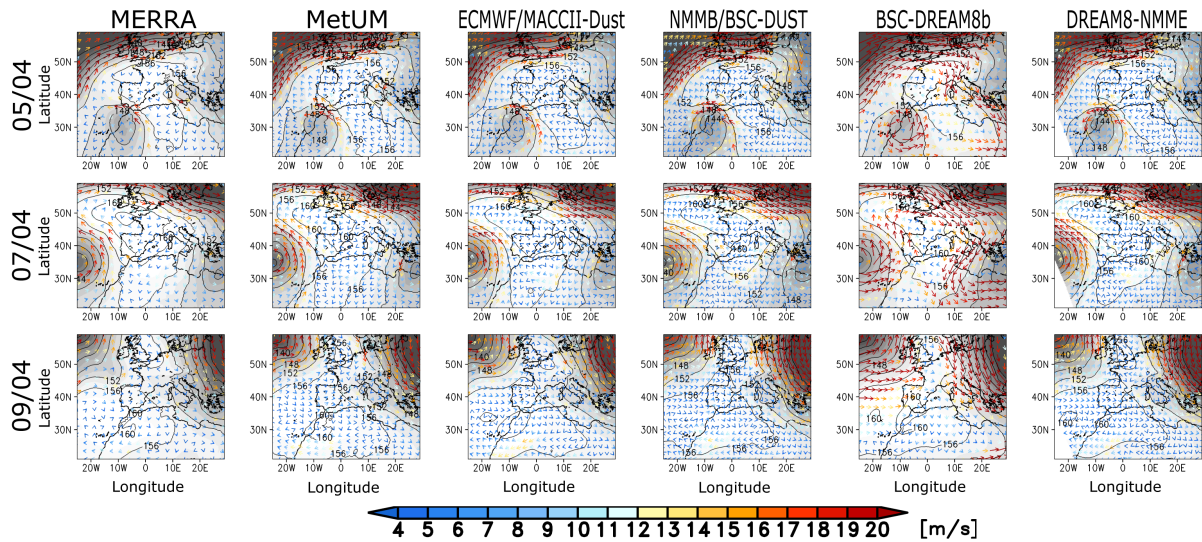
Figure S13: Same as Figure S12 but for 72 hour forecast.
