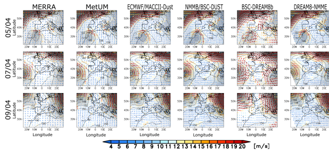
Figure S12: The geopotential height (contours) and wind speed stream lines at 850 hPa on 5 th (first row), 7 th (second row) and 9 th (third row) of April 2011 at 12 UTC from MERRA reanalysis and the 48 hour forecast from MetUM, ECMWF/MACC, NMMB/BSC-DUST, BSC-DREAM8b and DREAM8-NMME (from left to right).
