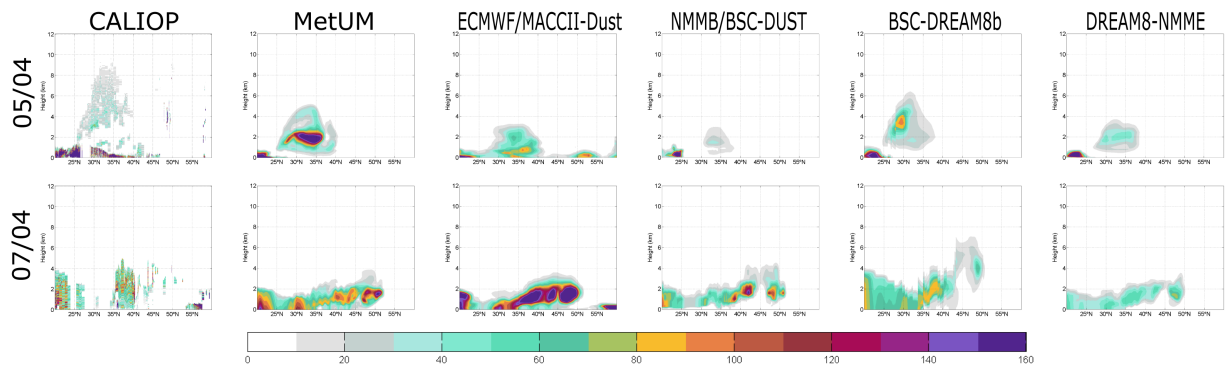
Figure S11: Same as Figure S09 but for 72-hour forecast.
