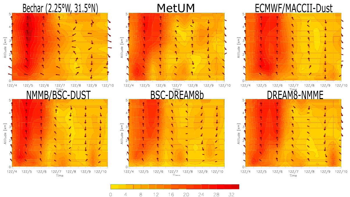
Figure S20: Same as Figure S19 but for 72-hour forecast.
