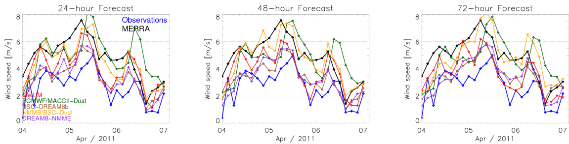
Figure S16: Observed (blue) three-hourly wind speed at 10m in dust source regions and corresponding re-analysis (MERRA, black), global models and regional models for the period 4 th Apr 2011 to 7 th Apr 2011 with (a) 24 hours lead time, (b) 48 hours, and (c) 72 hours. Observations are averaged over the region illustrated in Figure 1.
