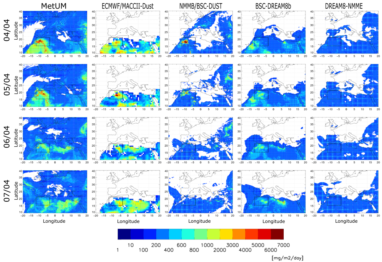
Figure S21: Total accumulated forecasted daily deposition with 48-hour lead time for the models MetUM, ECMWF/MACC, NMMB/BSC-DUST, BSC-DREAM8b and DREAM8-NMME (from left to right).
