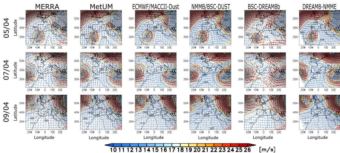
Figure S15: Same as Figure S14 but for 72 hour forecast.
