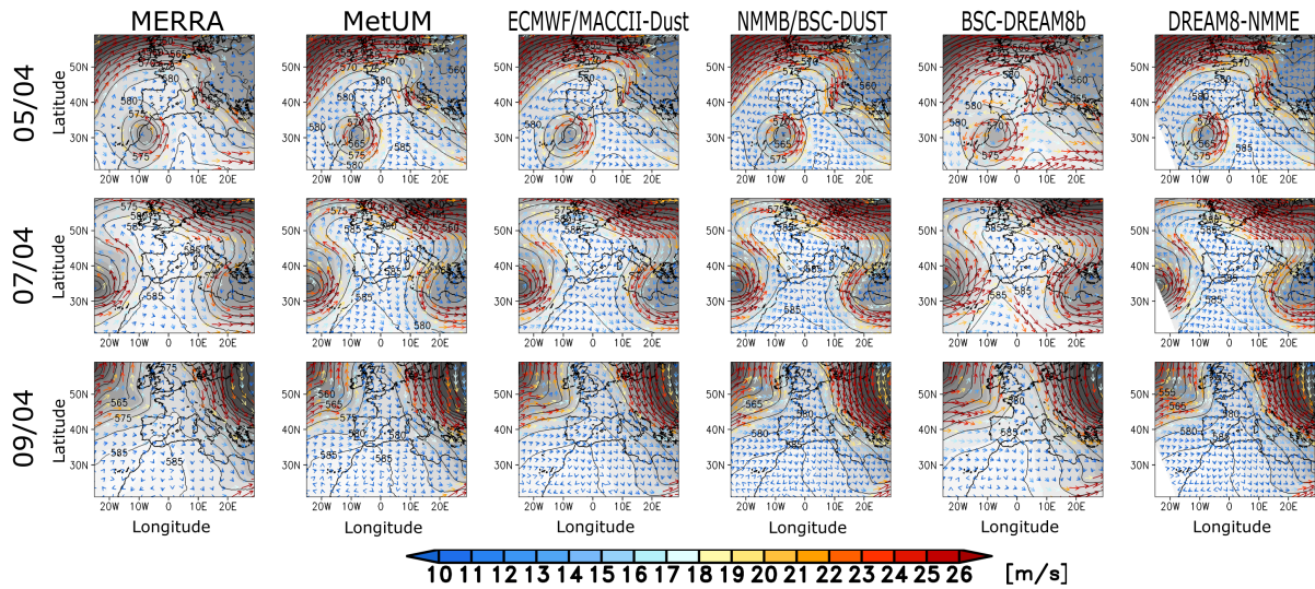
Figure S14: The geopotential height (contours) and wind speed stream lines at 500 hPa on 5 th (first row), 7 th (second row) and 9 th (third row) of April 2011 at 12 UTC from MERRA reanalysis and the 48 hour forecast from MetUM, ECMWF/MACC, NMMB/BSC-DUST, BSC-DREAM8b and DREAM8-NMME (from left to right).
