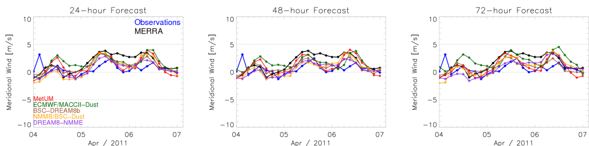
Figure S18: Same as Figure S17 but for meridional wind component.
