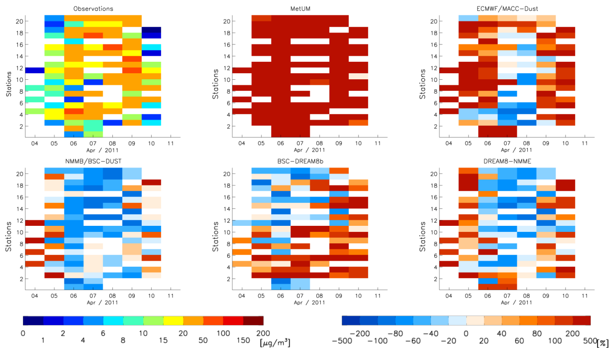
Figure S05: Daily measured surface concentration [ \mu\text{g m}^{-3} ] and normalized bias of corresponding 48 hour forecast surface concentration [%] at stations illustrated in Figure 1. Each row corresponds to one of the stations and the row for each station corresponds to the number presented in Fig. 1. Stations are ordered from south to north and white colour corresponds to days without measurements.
