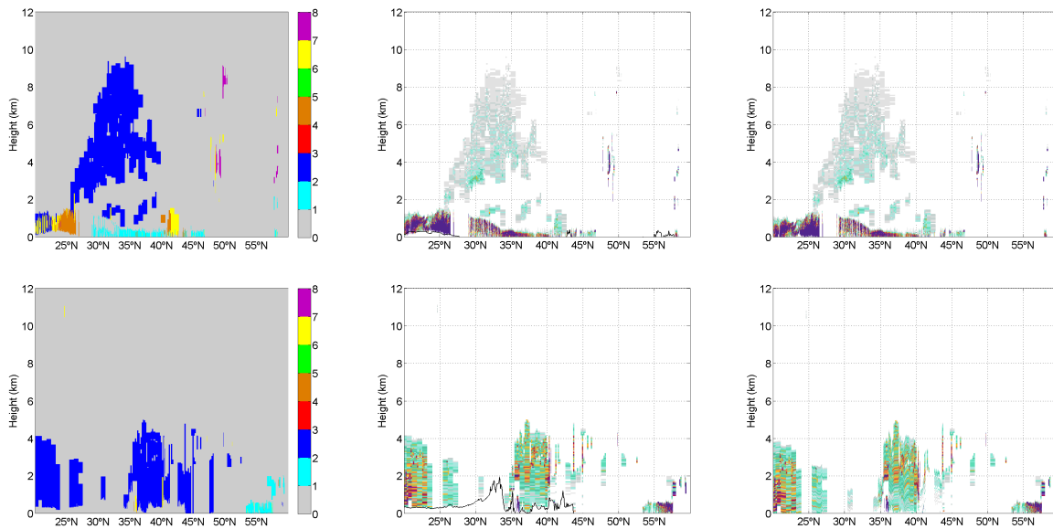
Figure S09: Profiles of CALIOP Vertical Feature Mask product (left panels) and total extinction coefficient at 532 nm (right panels) for 5th April at 2:41UTC (first row) and 7th April at 13:09UTC (second row). Central panels correspond to total extinction coefficient at 532 nm above sea level and right panel correspond to total extinction coefficient at 532 nm above surface level.
