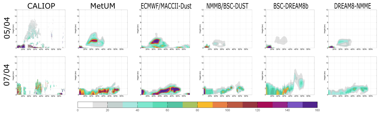
Figure S10: Profiles of measured extinction coefficient at 532 nm from the CALIOP instrument onboard of the CALIPSO satellite (first column) and 48-hour forecasted extinction coefficient profiles at 532 nm from models MetUM TM (second column), ECMWF/MACC (third column), NMMB/BSC-DUST (fourth column), BSC-DREAM8b (fifth column) and DREAM8-NMME (sixth column). Conditions are presented for the 5 th (upper row) and 7 th (lower row) of April. Overpass of the satellite in each case is illustrated in Figure S01.
