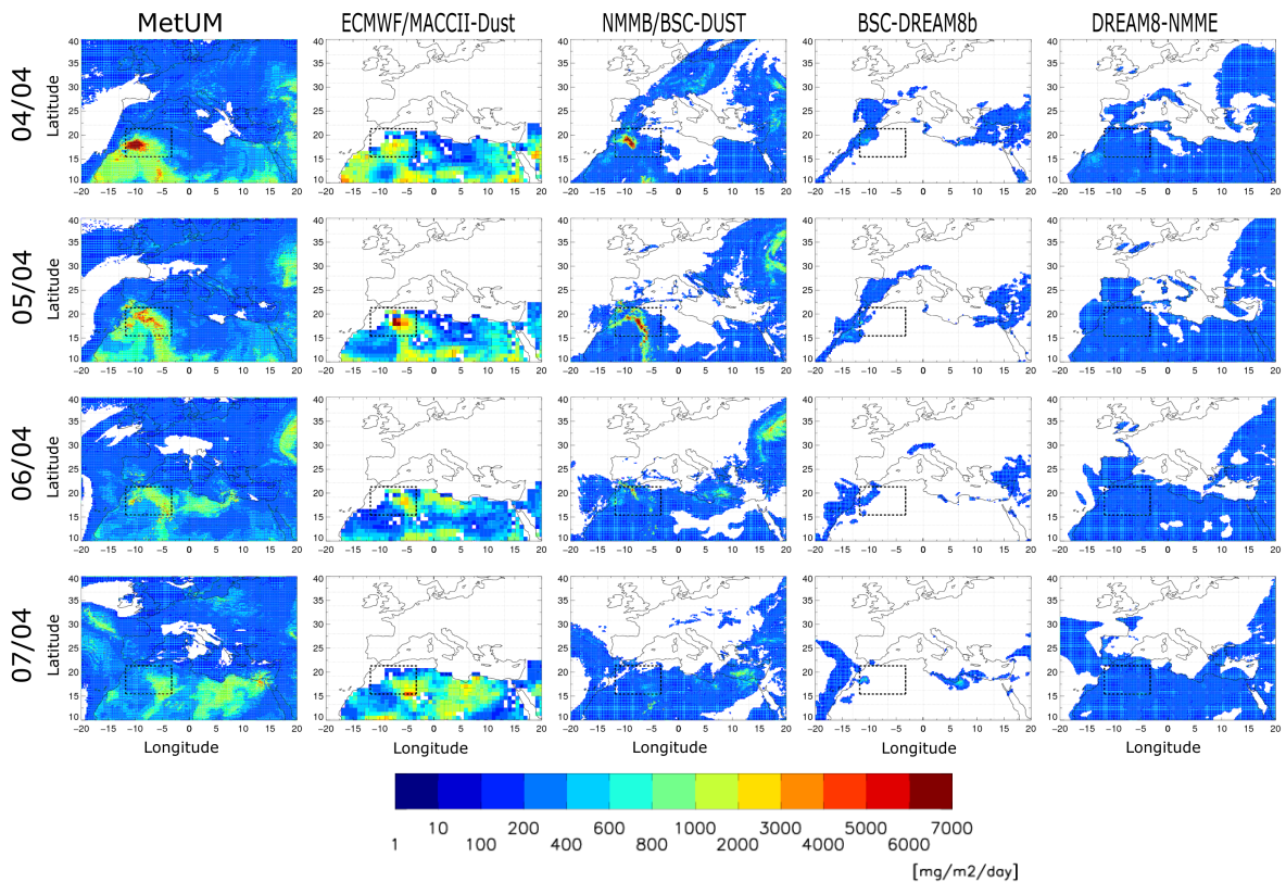
Figure S22: Same as Figure S20 but for 72-hour forecast.
