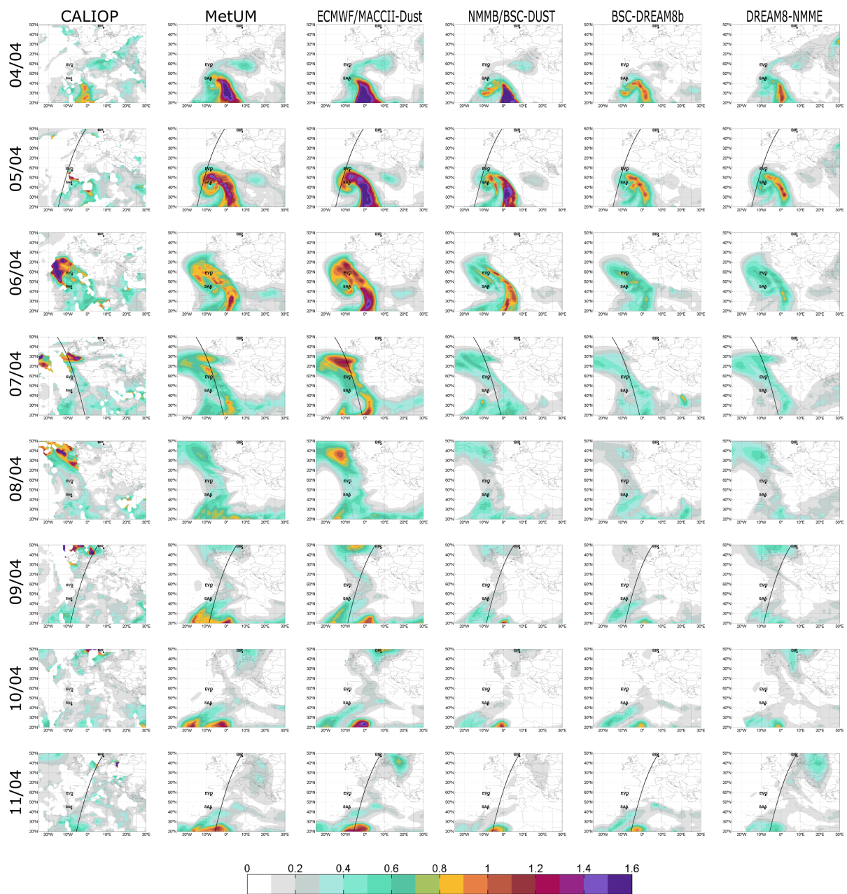
Figure S02: Same as Figure S01 but for 48-hour Forecast.
