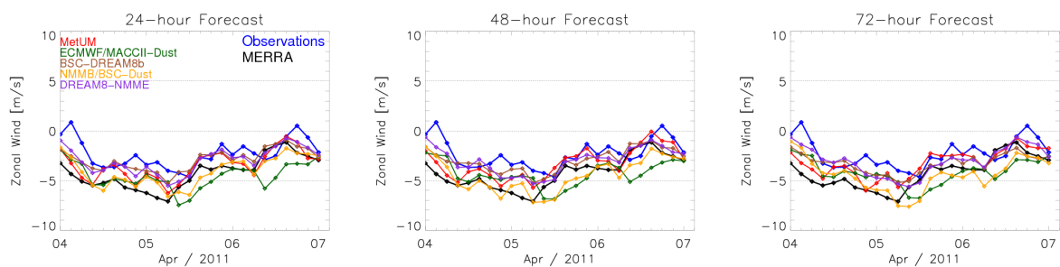
Figure S17: Observed three-hourly zonal wind component at 10m-wind in dust source regions and corresponding re-analysis (MERRA), global models and regional models for the period 4 Apr 2011 to 7 Apr 2011 with (a) 24 hours lead time, (b) 48 hours, and (c) 72 hours. Observations are averaged over the region illustrated in Figure 1.
