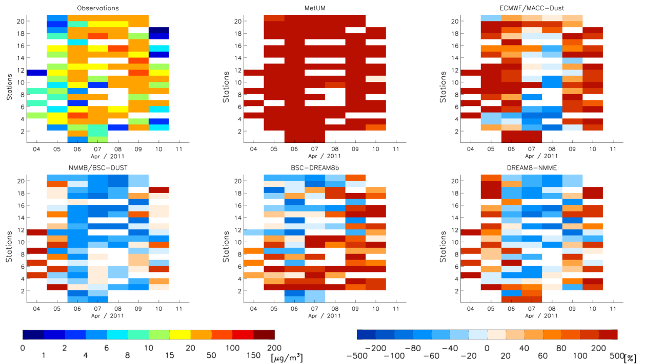
Figure S06: Same as Figure S05 but for 72-hour forecast
