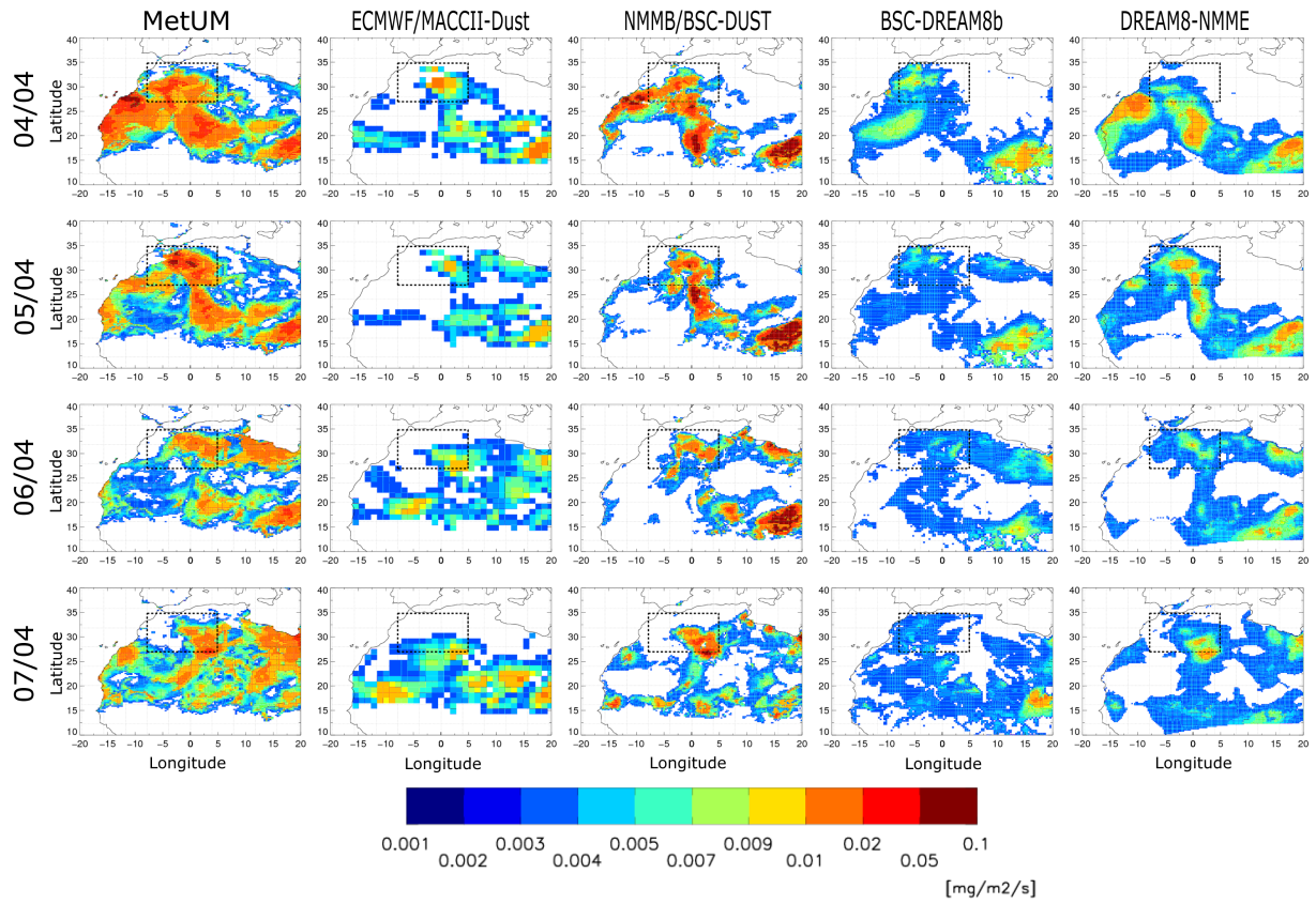
Figure S08: Same as Figure S07 but for 72-hour forecast.
