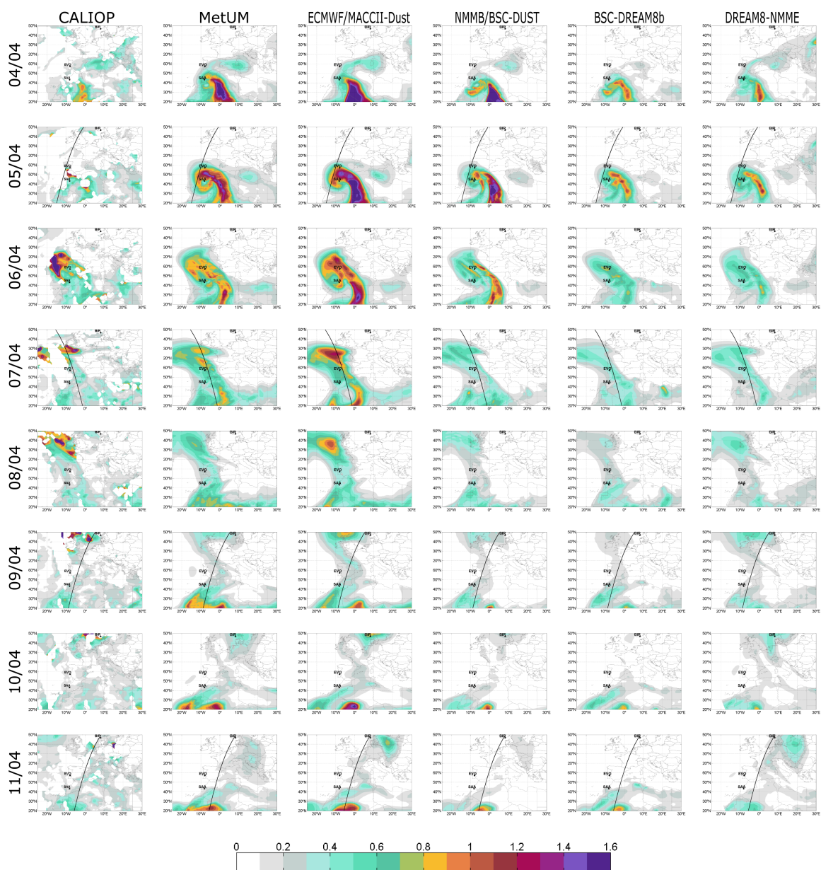
Figure S03: Same as Figure S01 but for 72-hour Forecast.
