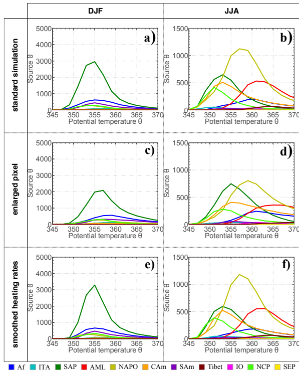
Figure 7. Comparison of the vertical source distribution, for ERA-Interim, for winter (DJF) and summer (JJA) between the standard backward calculation for 2005 (upper two panels)[ 136 ], when the CLAUS pixel size is enlarged by a factor 3 as described in the text (middle two panels), and when the 3-hourly sampling of daily cycle of heating rates is replaced by a time moving average as described in the text (lower two panels).
