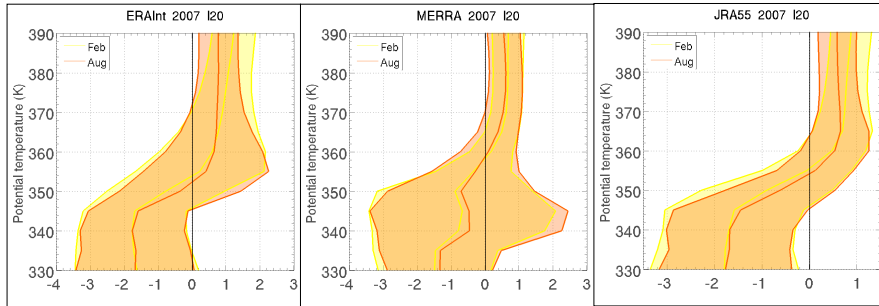
Figure 1. Mean heating rate profiles d\theta/dt and \pm one standard deviation for February 2007 (yellow) and August 2007 (red) averaged over 20^{\circ} S- 20^{\circ} N for the three reanalysis ERA-Interim, MERRA and JRA-55.
