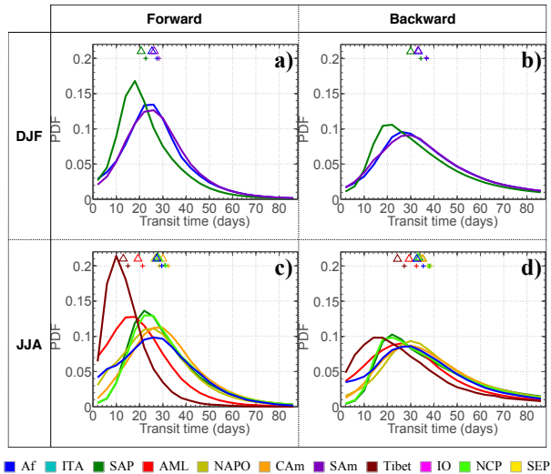
Figure 4. Distribution of the transit times in winter (DJF) and summer (JJA) for forward and backward calculations. The vertical axis is a [ \dots ] 135 probability density function in \text{day}^{-1} . Curves are plotted according to the color code of Fig. 1 but only for the active convective regions during each season. In the upper part of each panel, the triangles and the crosses indicate, respectively, the median and the mean for each curve.
