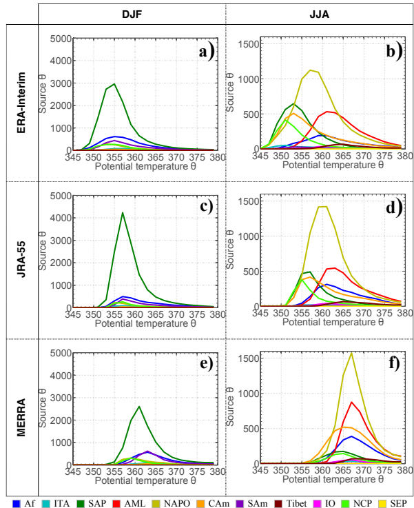
Figure 8. Vertical source distribution for winter (DJF) and summer (JJA) calculated for 2005 with JRA-55 and MERRA reanalysis using the same setup as for ERA-Interim. [ 137 ]Upper two panels, for ERA-Interim, are the same as those shown on the two upper panels of Fig. [ 138 ]7.
