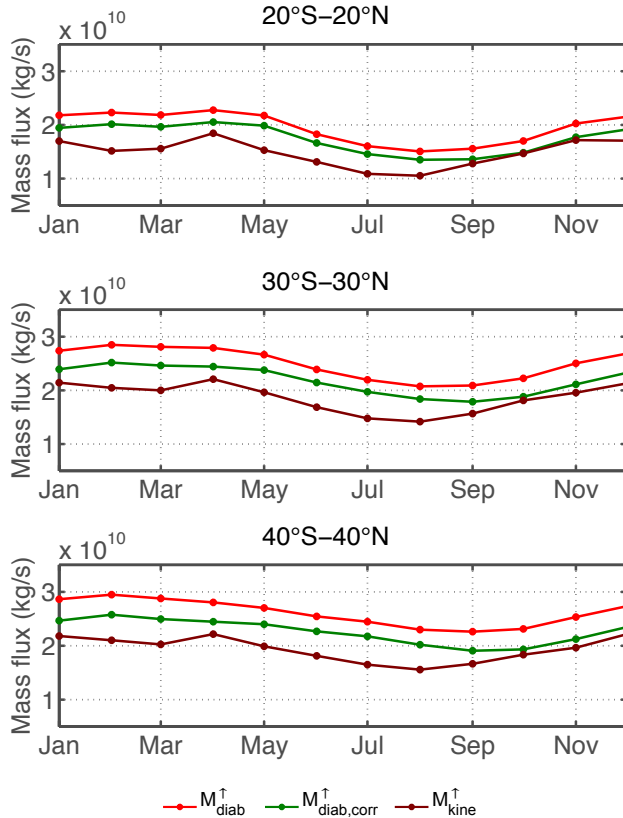
Figure 10. Annual variations of the monthly upward mass flux at the 380 K surface, calculated from the ERA-Interim data. M_{diab}^{\uparrow} and M_{diab,corr}^{\uparrow} : diabatic mass flux calculated from the radiative heating rates of ERA-Interim respectively with and without the mass conservation correction of the radiative heating rates. M_{kine}^{\uparrow} : kinematic mass flux calculated from the residual mean meridional circulation. All quantities are calculated and averaged over the years 2005 to 2008.
