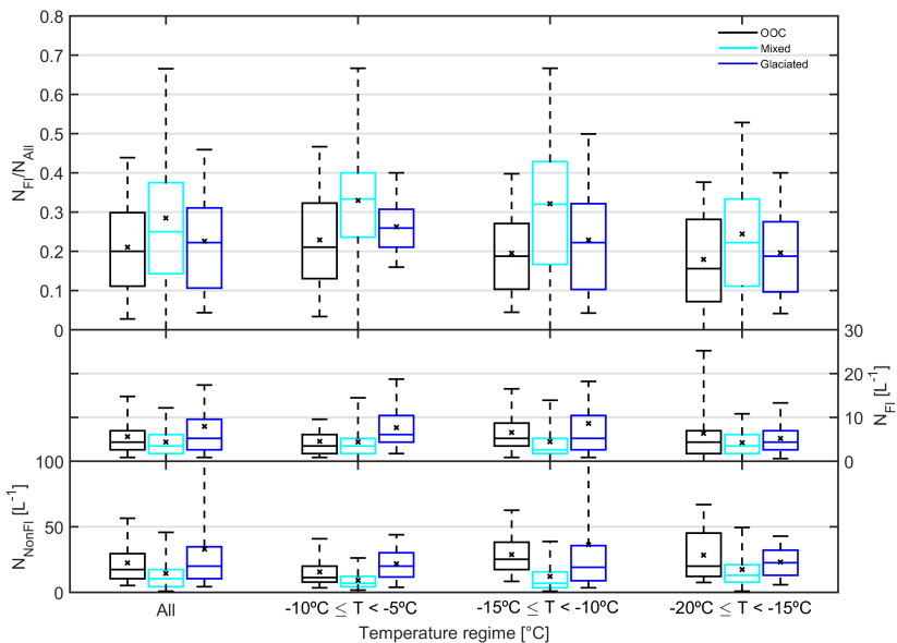
Figure 6. Top panel: fluorescent to total aerosol concentration ratio for out of cloud (black, TWC < 0.01 \text{ g m}^{-3} ), mixed phase (cyan, TWC \geq 0.01 \text{ g m}^{-3} and IMF < 0.9 ) and glaciated (blue, TWC \geq 0.01 \text{ g m}^{-3} and IMF \geq 0.9 ) conditions sampled with the total inlet. Middle and bottom panels: total fluorescent, N_{FI} , and total non-fluorescent, N_{NonFI} , aerosol concentrations. Box and whiskers denote 5th, 25th, 50th, 75th, and 95th percentiles. x marker denotes mean.
