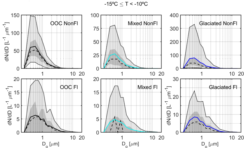
Figure 10. WBS Non-fluorescent (top) and fluorescent particle size distributions (bottom) for (left to right) out of cloud (OOC), mixed phase and glaciated conditions over the temperature range -15^{\circ}\text{C} \leq T < -10^{\circ}\text{C} . Solid line is mean, dashed line is median. 5th-95th percentiles and interquartile range shown with light and dark grey areas respectively.
