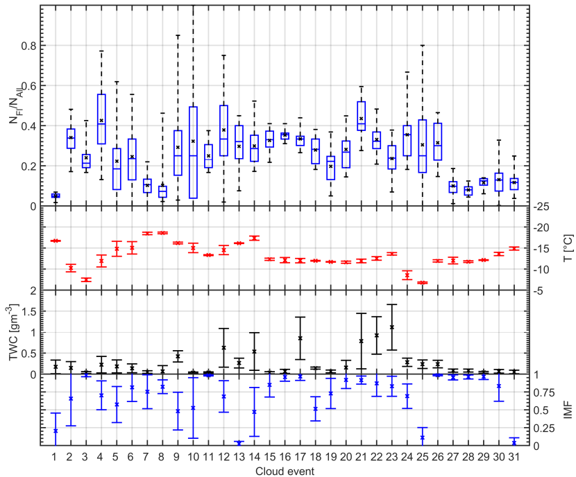
Figure 8. Box and whisker plots of fluorescent to total aerosol concentration ratio for cloud events persisting for at least 30 min in duration with accompanying temperature, total water content and ice mass fraction measurements. Box and whiskers denote 5th, 25th, 50th, 75th, and 95th percentiles. x marker denotes mean.
