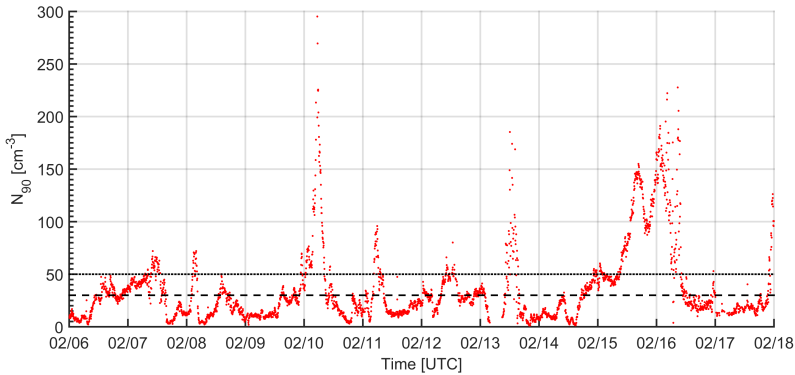
Figure 3. Time series of N_{90} concentration for the analysis period. Dashed line denotes the 30 \text{ cm}^{-3} background concentration described in Herrmann et al. (2015); the dotted line denotes this 50 \text{ cm}^{-3} threshold used to distinguish free tropospheric conditions.
