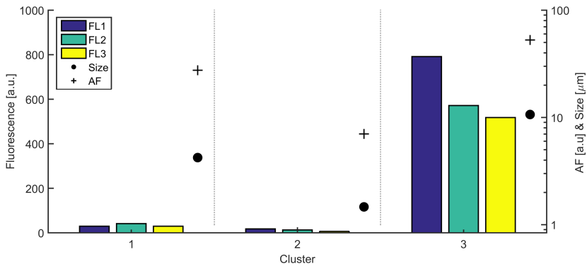
Figure 12. Mean cluster centres for the 3 cluster solution using Ward linkage and Calinski–Harabasz metric. Clusters contribute 25, 70 and 5% respectively to the fluorescent particle population.
