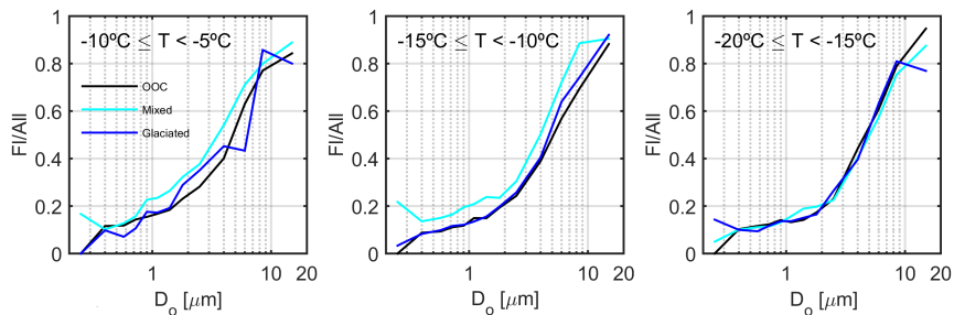
Figure 11. Size dependent fluorescent aerosol fractions for (left to right) out of cloud (black), mixed phase (cyan) and glaciated conditions (blue) over the three different temperature regimes studied.
