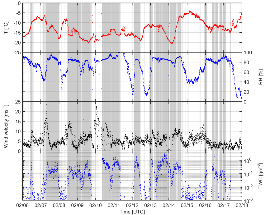
Figure 1. Time series of meteorological data and total water content at the JFJ site for the period 6–18 February. Grey shaded areas denote in cloud periods ( TWC \geq 0.01 \text{ g m}^{-3} ).
