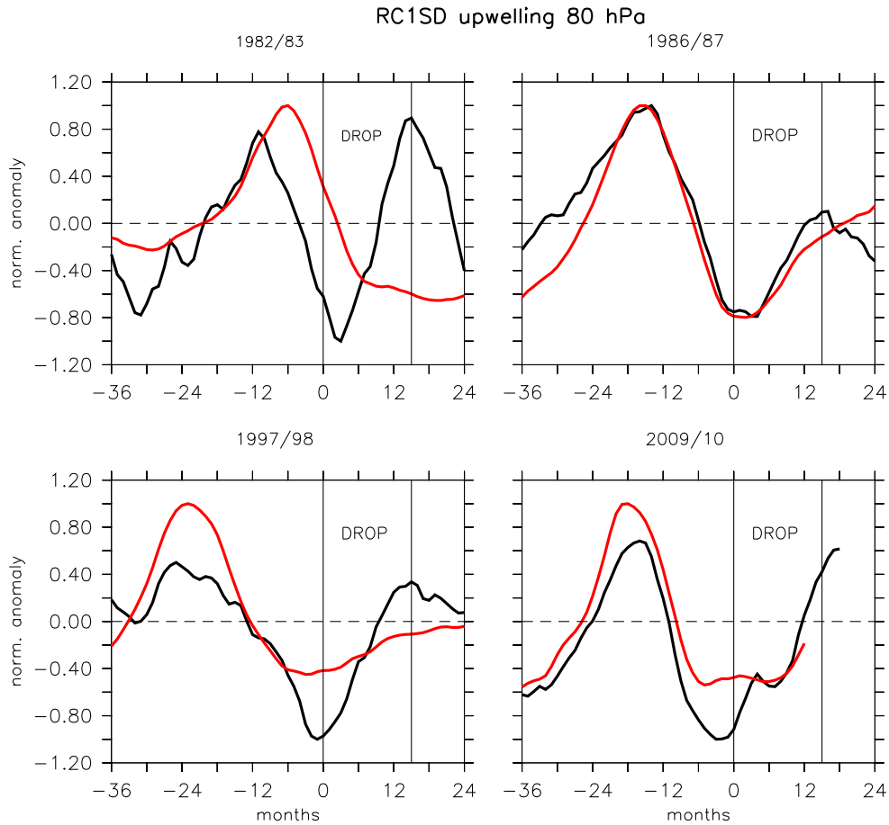
Figure 16. Episode analysis for the normalised upwelling anomaly (black) for ( 10^{\circ} N– 10^{\circ} S) at 80 hPa and the max-normalised SST anomaly for the El Niño index 3.4 region (red). The normalised upwelling anomaly is calculated by division of either the maximum or the absolute value of the minimum. For the SSTs it is defined accordingly. Therefore, the results are dimensionless. All episodes are referenced to the beginning of the temperature drop. The drop onsets are accompanied by a negative upwelling anomaly.
