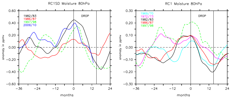
Figure 12. Same as Fig. 11, but for the water vapour anomaly. Note that the vertical axis is smaller in the right figure.
