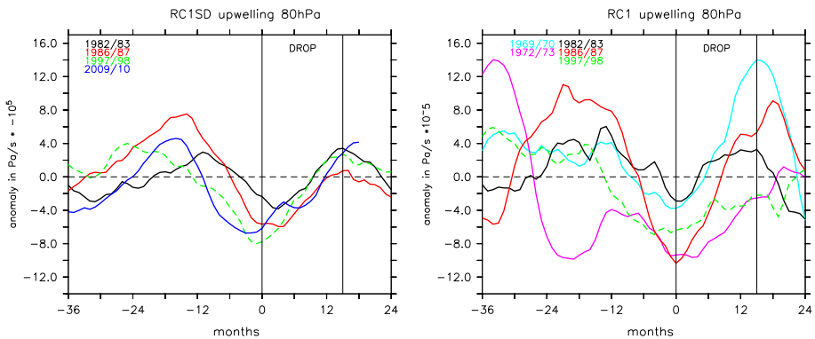
Figure 13. Same as Fig. 11, but for tropical upwelling anomaly.
