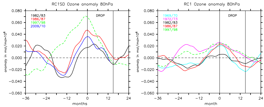
Figure 14. Same as Fig. 11, but for the ozone anomaly.
