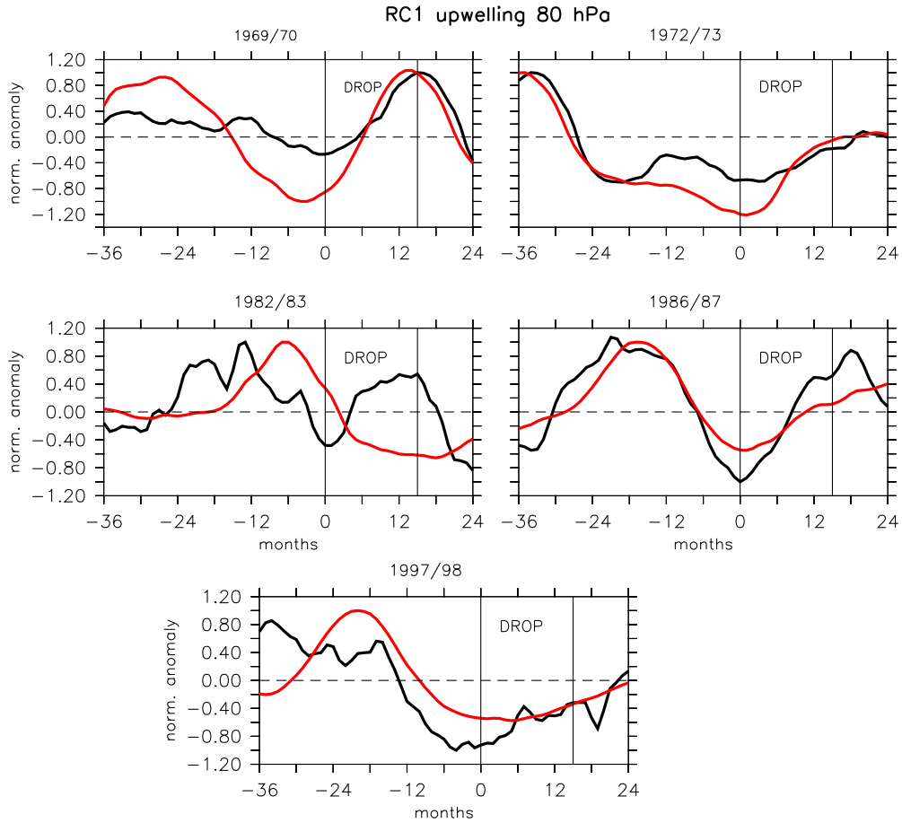
Figure 17. Episode analysis for the normalised upwelling anomaly at 80 hPa (black) for ( 10^{\circ} N– 0^{\circ} S) and the max-normalised SST anomaly for the El Niño index 3.4 region (red). The normalised upwelling anomaly is calculated by division of either the maximum or the absolute value of the minimum. For the SSTs it is defined accordingly. Therefore, the results are dimensionless. All episodes are referenced to the beginning of the temperature drop. The drop onsets are accompanied by a negative upwelling anomaly.
