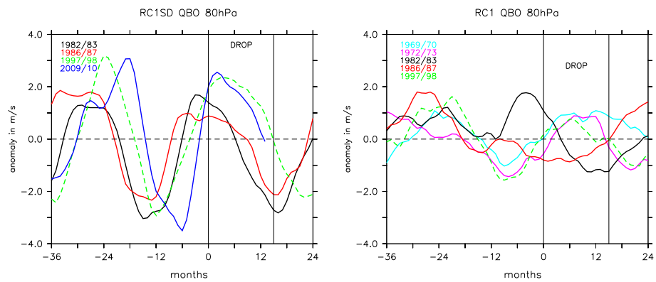
Figure 15. Same as Fig. 11, but for the QBO anomaly. The QBO is represented through the zonal wind anomaly.
