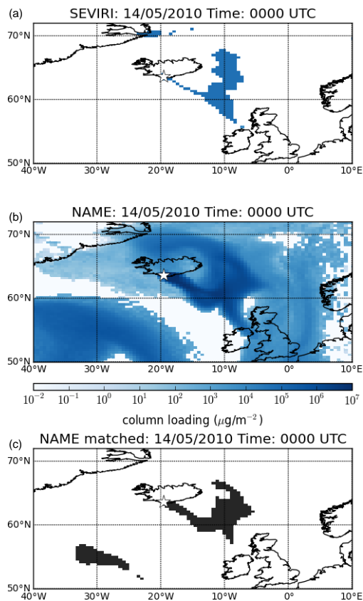
Figure 1. Ash column loading at 00:00 UTC on 14 May 2010 (a) by the satellite (with 5x smoothing), (b) simulated by NAME, (c) NAME simulated ash cloud after pixel matching (i.e. black indicates pixels selected in satellite matching process). Panel (a) uses the colour scale shown in panel (b) .
