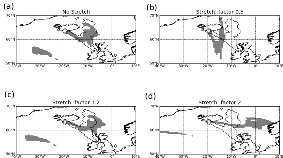
Figure 3. The pixel matched NAME ash cloud (grey shading) compared to the satellite retrieved ash cloud (black outline) with (a) no stretch, (b) stretch factor 0.5, (c) stretch factor 1.2, (d) stretch factor 2.
