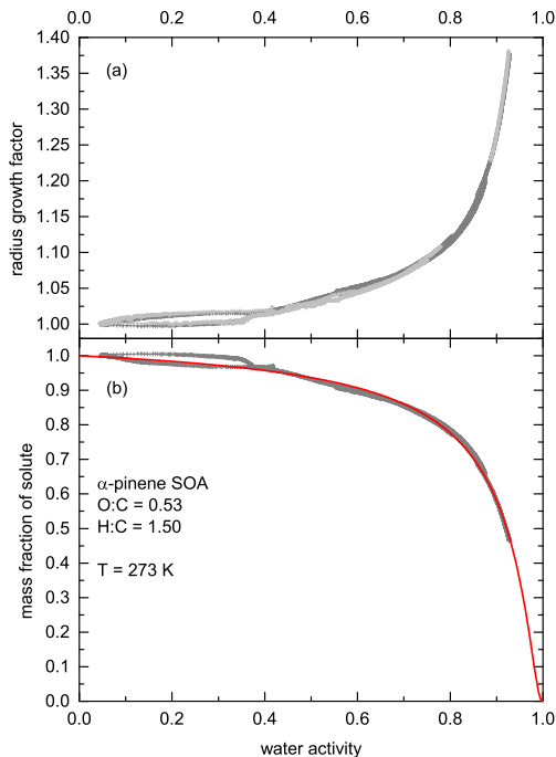
Figure A4. (a) Radius growth factor of a \alpha -pinene SOA particle (O:C=0.53) at 273 K as derived from Mie resonance spectroscopy (light gray crosses) and from mass balance (dark gray crosses) yielding 1.40 \pm 0.05 \text{ g cm}^{-3} for the density of the pure solute. (b) Mass fraction of solute vs. water activity calculated from the data of panel (a). The red line represents the fit according to Eq. (A9). (A fit to a single parameter, \kappa , for describing hygroscopic growth as in Pajunoja et al. (2015) yields a value of 0.081 \pm 0.005 Petters and Kreidenweis, 2007.)
