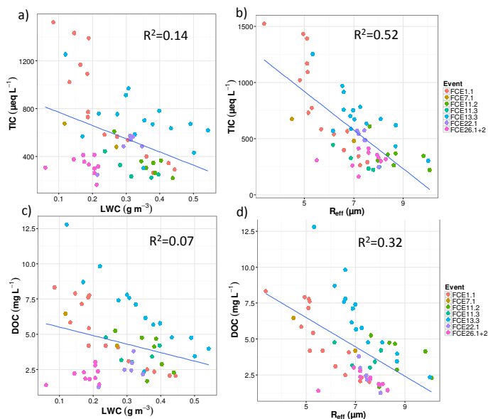
Figure 4. Relationships of total ionic content (upper panels) and dissolved organic carbon (lower panels) vs. liquid water content ( a and c ) and effective droplet radius ( b and d ) for bulk cloud water samples.
