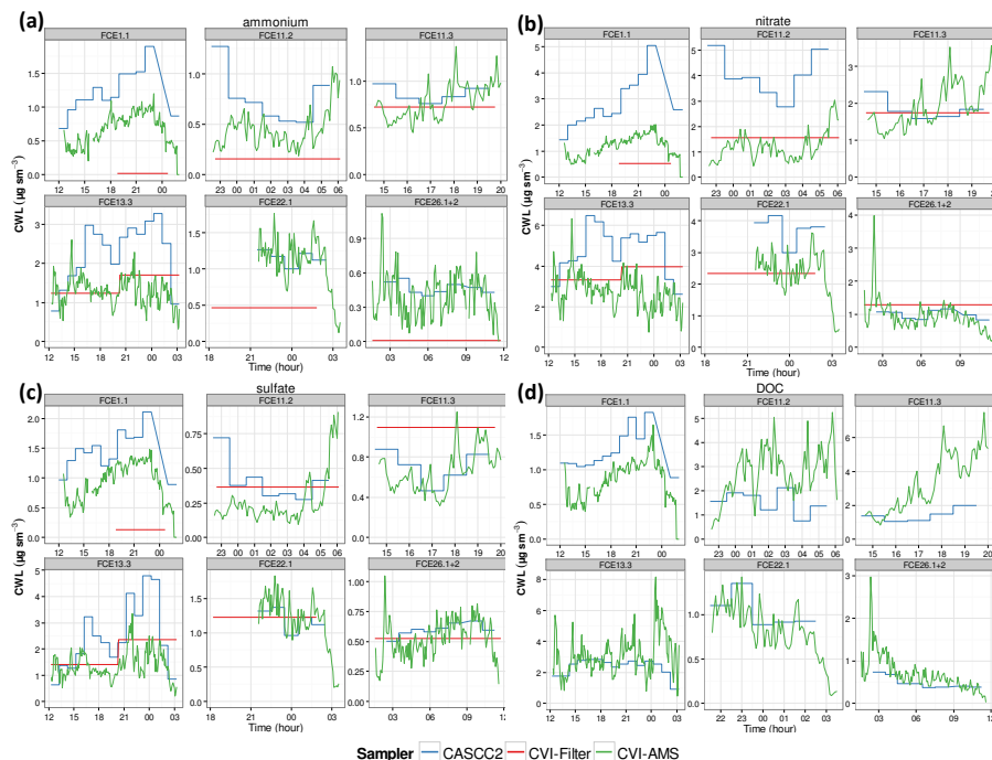
Figure 5. Comparison of cloud water loadings (normalised to standard temperature and pressure) from bulk cloud water collector (blue), quartz filter downstream CVI inlet (red), and AMS downstream CVI (green) for cloud water main constituents (a) ammonium, (b) nitrate, (c) sulfate, and (d) DOC (AMS organics/1.8).
