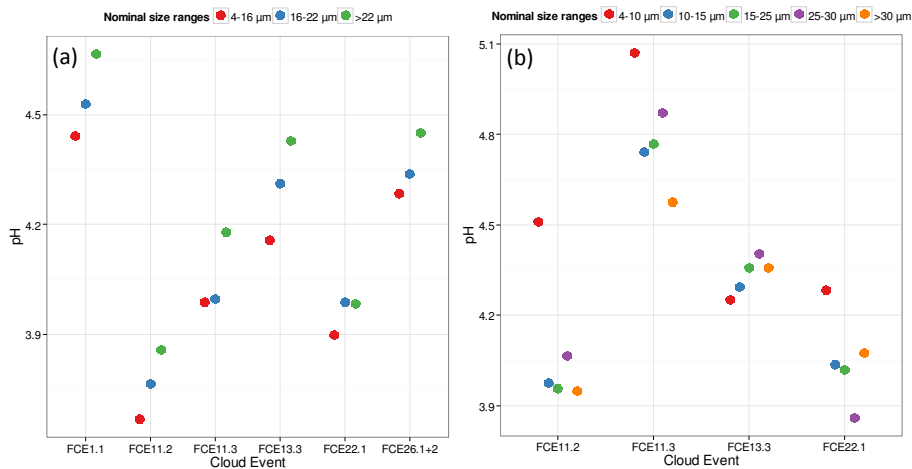
Figure 8. Mean pH values per event, calculated from volume-weighted mean concentrations of H + from (a) 3-stage cloud water collector, and (b) 5-stage collector.
