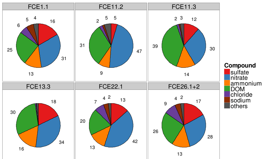
Figure 1. Volume-weighted mean composition of bulk cloud water during main events. Numbers represent percentage from total solute concentration (in \text{mg L}^{-1} ). Trace solutes calcium, magnesium, potassium, \text{H}_2\text{O}_2 (aq), and S(IV) are summarised as “others”. DOM is calculated as \text{DOC} \cdot 1.8 .
