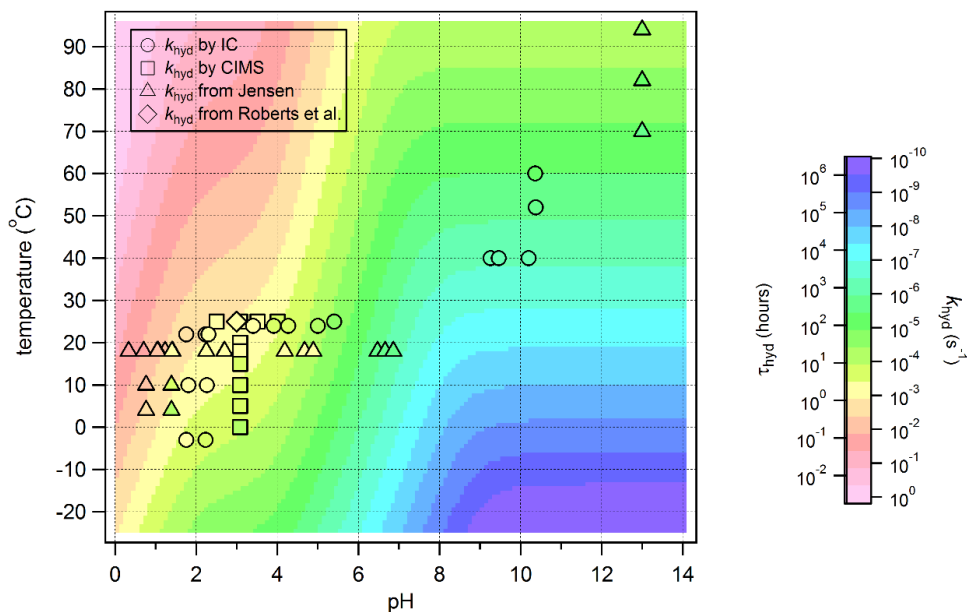
Figure 7. k_{\text{hyd}} as function of temperature and pH generated from Eq. (8) using our obtained values for k_1 , k_2 , and k_3 and for E_{a1} , E_{a2} , and E_{a3} . All available k_{\text{hyd}} measurements for HNCO in the literature and from this work are superimposed and colour coded appropriately. As a guide, the colour scale also represents the lifetime in hours for HNCO in dilute aqueous solutions.
