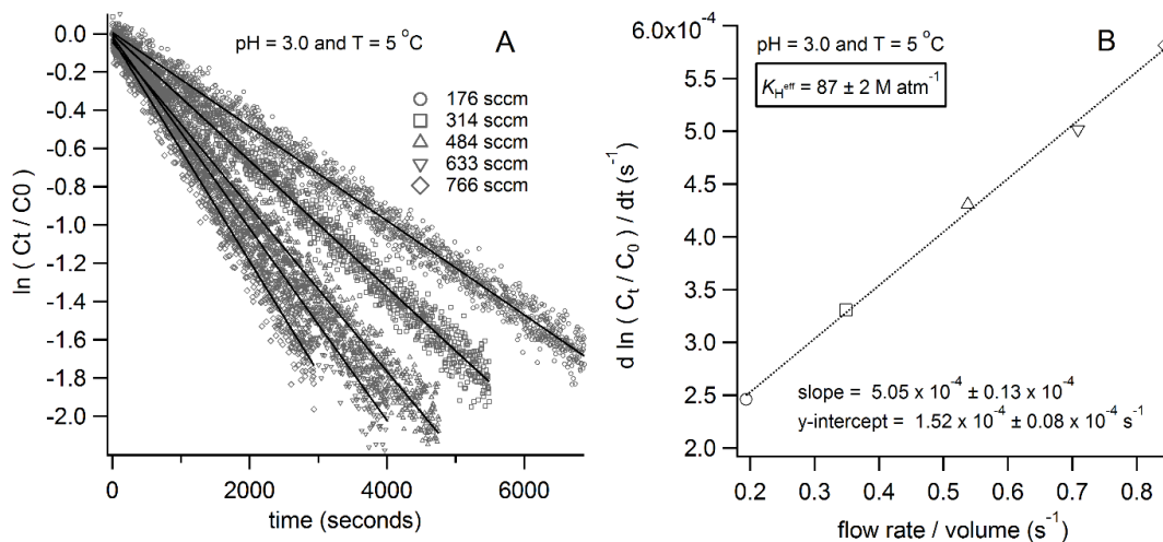
Figure 2. (a) The concentration decay curves as a function of time according to Eq. (4) for each flow rate shown; (b) the slopes of each fit in panel (a) plotted as a function of the ratio of the flow rate to the volume. The symbols in both figures represent the same flow rate shown.
