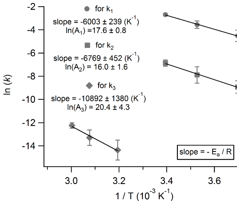
Figure 6. The linear plots of the natural logarithm of each hydrolysis rate coefficient k_1 , k_2 , and k_3 as a function of the inverse of temperature to yield the activation energies of each mechanism.
