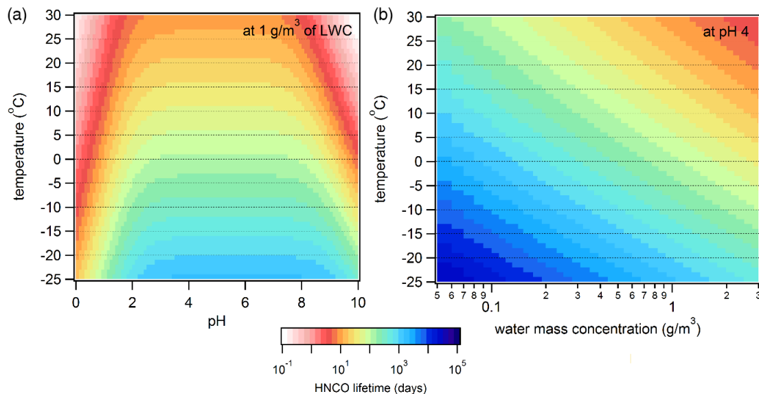
Figure 8. (a) The lifetime of HNCO in days as a function of temperature and pH at 1 g m -3 of LWC and (b) the lifetime of HNCO in days as a function of temperature and LWC at pH 4.
