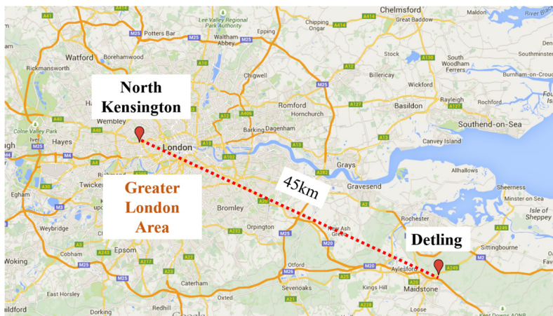
Figure 1. Geographical locations of the sampling sites (i.e., North Kensington and Detling) in this study. The region circled by the M25 motorway is the greater London area. The map is adapted from Google Maps.
