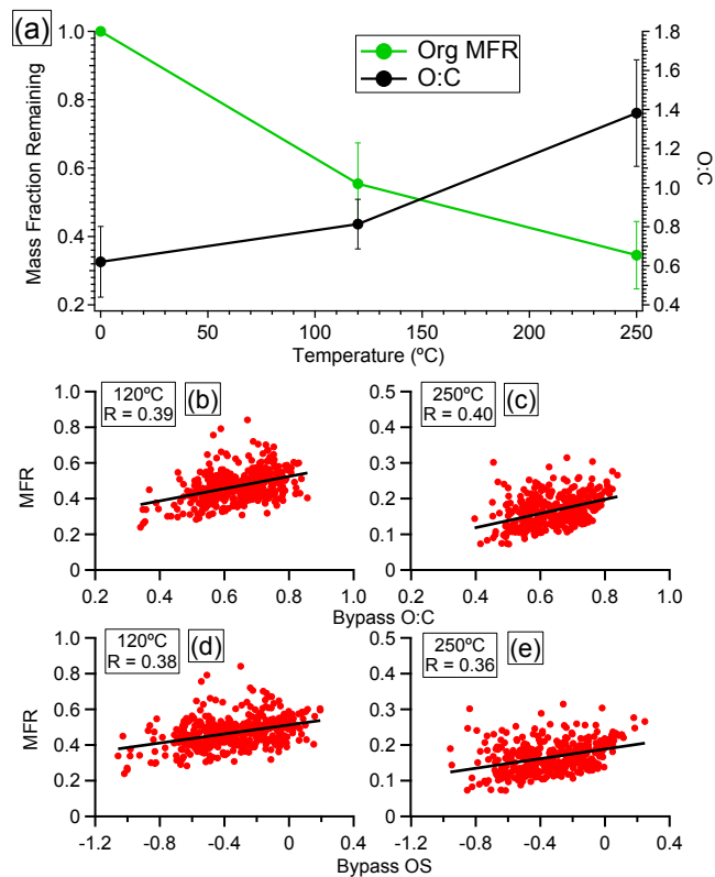
Figure 12. (a) Organic mass fraction remaining (MFR) and O:C as a function of TD temperature; (b) organic MFR at 120°C and 250°C as a function of bypass line organic O:C and oxidation state.
