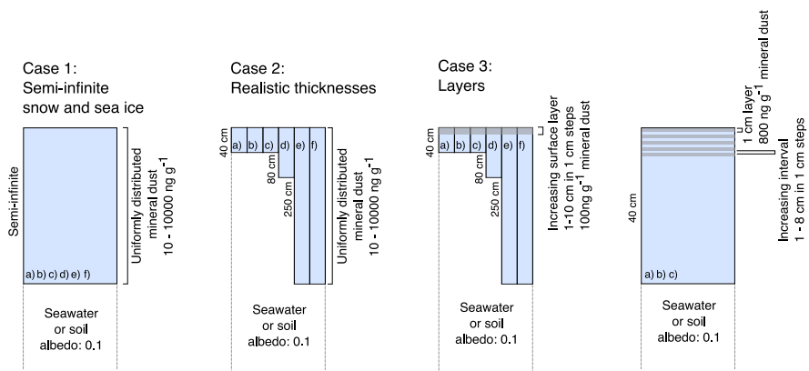
Figure 1: Snow and sea ice configurations modelled for a) cold polar snow, b) coastal windpacked snow, c) melting snow, d) first year sea ice, e) multi year sea ice, f) melting sea ice (not to scale).
