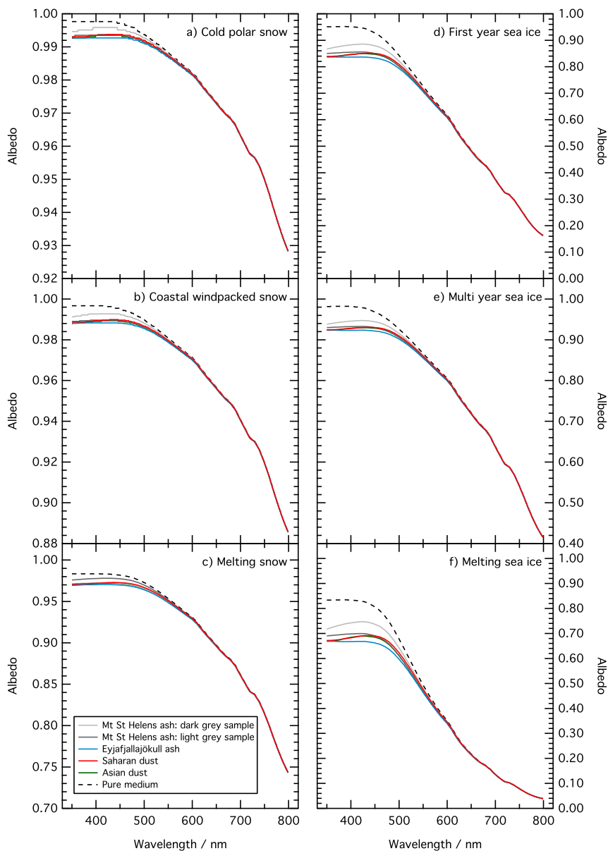
Fig. 4. Wavelength dependant albedo of three semi-infinite snow and sea ice types containing 100 ng g -1 of different mineral aerosol deposits (Mt St Helens ash , Eyjafjallajökull ash, saharan dust and Asian dust). The albedo of a pure medium (containing 1ng g -1 of Asian dust) has been included for comparison. The y-axis has different scales in each panel to cover the large range of values.
