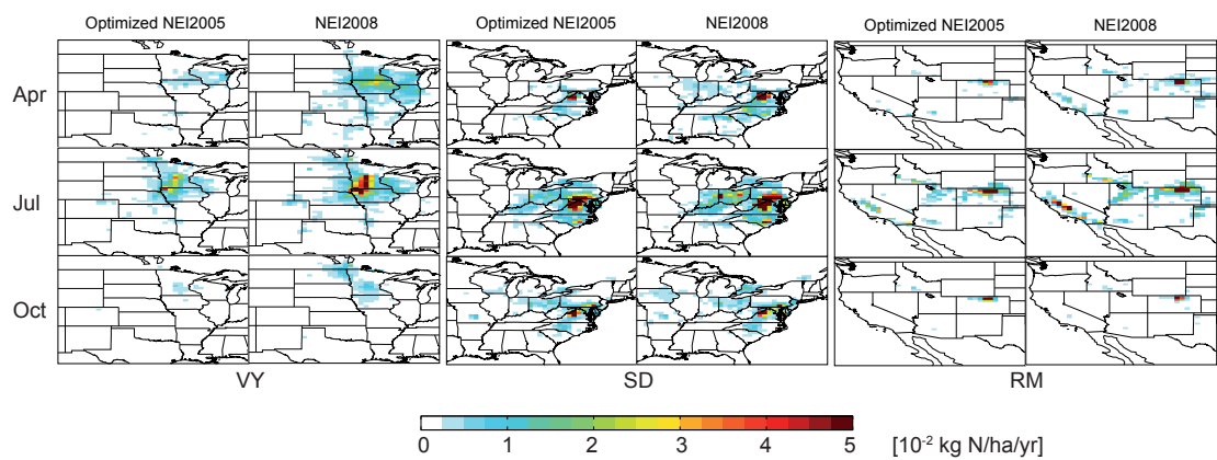
Figure 12. Map of sensitivities of J_p to \text{NH}_3 emissions for 3 selected Class I areas (VY, SD, and RM) for two different \text{NH}_3 emission inventories (optimized NEI2005 and default NEI2008) in each month.
