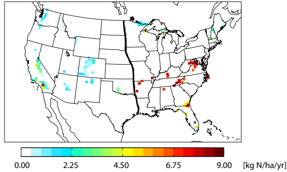
Figure 9. CL exceedance in Class I areas; color indicates magnitude of exceedance. The size of Class I areas are not reflected. Grid cells containing Class I areas are shown as colored regardless of the fraction of Class I areas. Bold line divides Western and Eastern US.
