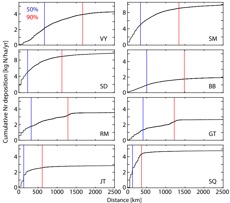
Figure 6. Annual averaged monthly cumulative contribution as a function of distance from the site. Vertical lines are for 50% (blue) and 90% (red) of total Nr deposition. Note that the change in scale of the y -axis for SM and SD.
