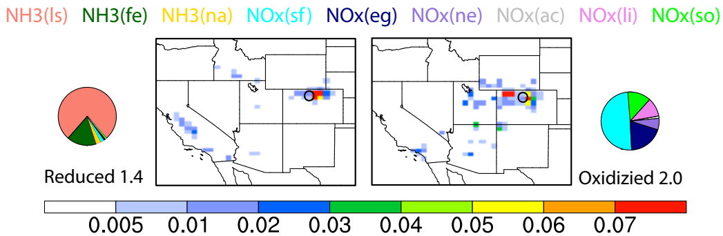
Figure 7. Same as Fig. 5 but for oxidized and reduce Nr deposition in RM. Units for the pie charts and colorbar are kg N/ha/yr. The sum of the oxidized and reduced Nr deposition is smaller than the inset number in Fig. 5 because the number here excludes Nr from "other species."
