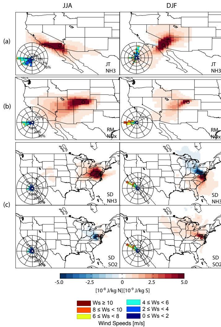
Figure 8. Efficiencies of impacts on Nr deposition showing cost function ( J_p ) change per kg N or kg S emission for the tracer and season indicated in the plot. (a) Joshua Tree (b) Rocky Mountain (c) Shenandoah national parks. Wind-roses for each site show fraction of wind frequencies based on daily surface winds during the season.
