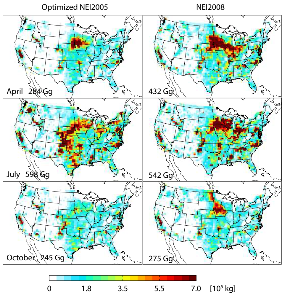
Figure 11. Sum of NH 3 emissions from anthropogenic, natural, biomass burning, and biofuel sources. Inset numbers are contiguous US total NH 3 emissions in each month.
