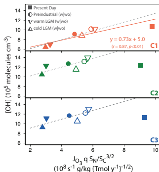
Figure 7. Tropospheric mean mass-weighted OH burden in each simulation as a function of J_{\text{O}_3} q S_{\text{N}} / \left( S_{\text{C}}^{3/2} \right) , where J_{\text{O}_3} is the tropospheric mean mass-weighted ozone photolysis frequency ( \text{s}^{-1} ), q is the tropospheric mean mass-weighted specific humidity ( \text{g kg}^{-1} ), and S_{\text{N}} and S_{\text{C}} are the tropospheric sources of reactive nitrogen ( \text{Tmol N a}^{-1} ) and of reactive carbon ( \text{Tmol C a}^{-1} ), respectively. S_{\text{C}} is calculated as the sum of emissions of CO, NMVOCs, and an implied source of methane equal to its loss rate by OH. Model results for different chemistry schemes are separated into three subsets as follows. Top panel: original isoprene chemistry and original \text{HO}_2 uptake (C1). Middle panel: new isoprene chemistry and original \text{HO}_2 uptake (C2). Bottom panel: new isoprene chemistry and new \text{HO}_2 uptake (C3). Different symbols denote different climate scenarios (present day, preindustrial, warm LGM, cold LGM). Filled symbols represent simulations in which the \text{CO}_2 -sensitivity of plant isoprene emission is considered (w); unfilled symbols are those without (wo). All present-day simulations were performed with \text{CO}_2 -sensitivity turned on. The orange line shows a reduced major axis regression fit for the C1 subset, with the regression equation and correlation coefficient ( r = 0.87 , p < 0.01 ) inset. We do not find a statistically significant correlation between OH and J_{\text{O}_3} q S_{\text{N}} / \left( S_{\text{C}}^{3/2} \right) for the C2 ( r = 0.36 ) and C3 ( r = 0.34 ) subsets. When the present-day values are excluded and a multiple regression model is fitted to the remaining ensemble, we find that the three different chemistry schemes possess the same values for the slopes of the linear correlation but different values for the intercepts, as shown by the dashed grey lines (see text for details).
