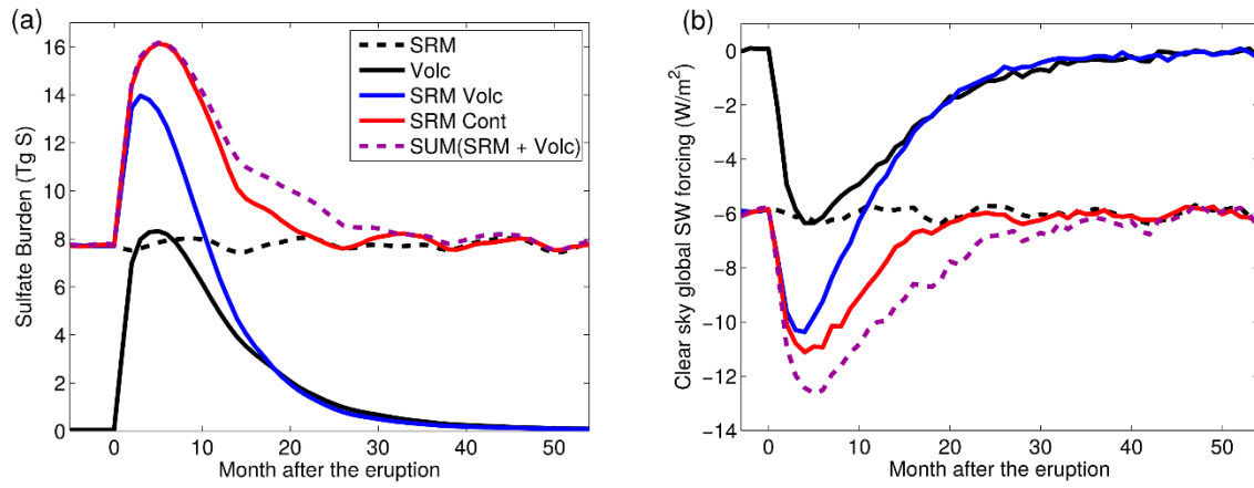
Figure 2. a) Stratospheric sulfate burden and b) global mean clear sky shortwave radiative forcing at the surface in the different scenarios. In addition, the dashed purple line represents the sum of SRM and Volc runs, and is shown for comparison.
