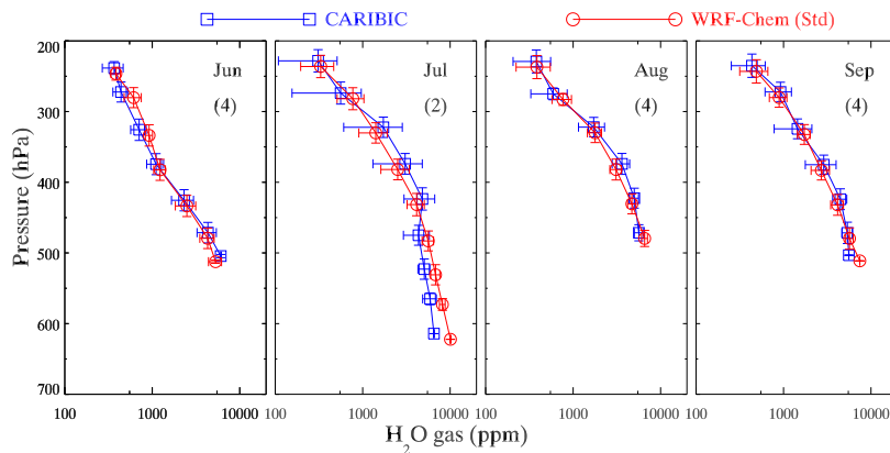
Figure 4. New Figure added Comparison of monthly average \text{H}_2\text{O} gas (ppm) from standard WRF-Chem simulations (Std) with the CARIBIC observations during June, July, August and September 2008. Numbers in brackets denote the number of observational profiles in the respective month. Model output has been spatially and temporally interpolated along the CARIBIC flight tracks. Note the logarithmic scale on X axis.
