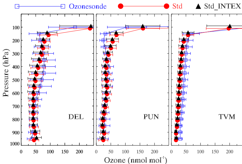
Figure 5. New Figure added Comparison of average ozone mixing ratios during the summer monsoon (June-September) from Std and Std_INTEX WRF-Chem simulations (Std) with the ozonesonde observational climatology during 2006-2009 period over Delhi (DEL), Pune (PUN) and Thiruvananthapuram (TVM).
