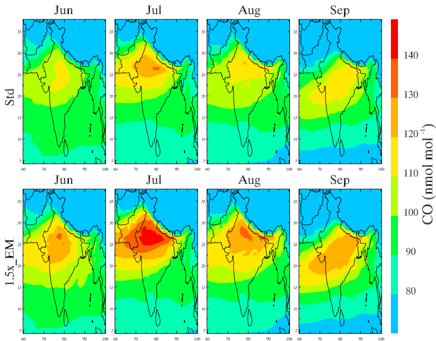
Figure 9. New Figure Added Comparison of monthly average horizontal distribution of CO in the upper troposphere (116 hPa to 211 hPa) over India from the Std simulation (top panel) and 1.5\times\_EM simulation (bottom panel) during June, July, August and September 2008.
