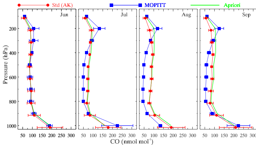
Figure 6. Added apriori profile Comparison of monthly average CO from WRF-Chem simulations (Std) with the MOPITT retrievals over Chennai during the four months of the summer monsoon period of the year 2008. The MOPITT averaging kernel and the a priori profile have been applied to the WRF-Chem output, denoted by Std (AK). MOPITT a priori profile is also shown for comparison.
