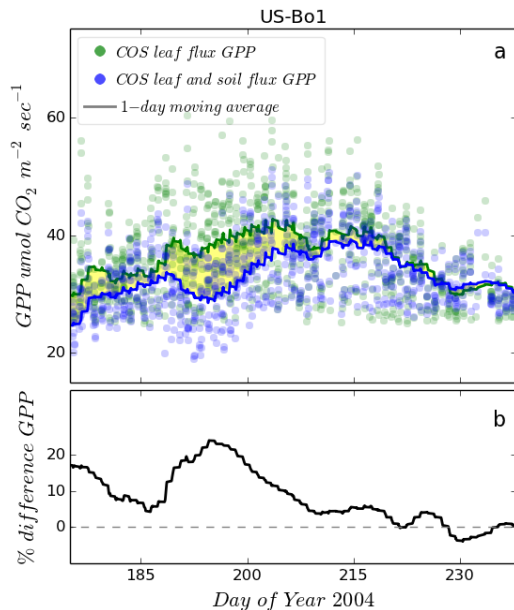
Figure 14. Comparing theoretical GPP estimates based on gross COS leaf fluxes vs. net ecosystem COS fluxes. (a) Theoretical GPP estimates based on leaf COS uptake, GPP estimates based on net ecosystem COS fluxes calculated by Eqs. (1) and (3), and their moving averages for a 24 h window. The yellow shaded region highlights the difference between COS-GPP proxy when no soil correction is included and the reported GPP. (b) The percentage difference between the 1 day moving average of reported GPP and the calculated COS flux-GPP estimates with modeled soil COS exchange included.
