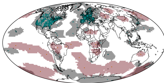
Figure 11. Map of surface ozone observational coverage as in Fig. 2 (blue dots indicate current measurement sites and grey areas their footprints) with the twenty additional sites and footprints from Figs. 9 and 10 added as red dots and pink areas to illustrate the global coverage if ozone measurements were made at these sites.
