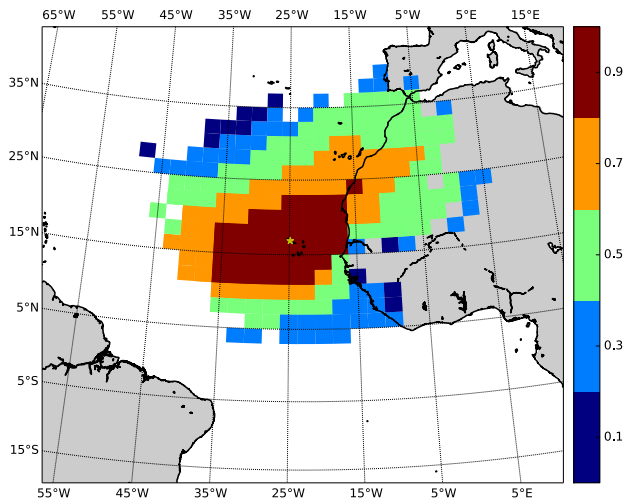
Figure 1. Example of the site footprint for the Cape Verde Observatory ( blue marker yellow star ; 16° 51' 49" N, 24° 52' 2" W ) derived using thresholds of R = 0.1 to 0.9 in the spatial correlation of monthly anomalies in surface ozone from the GEOS-Chem model.
