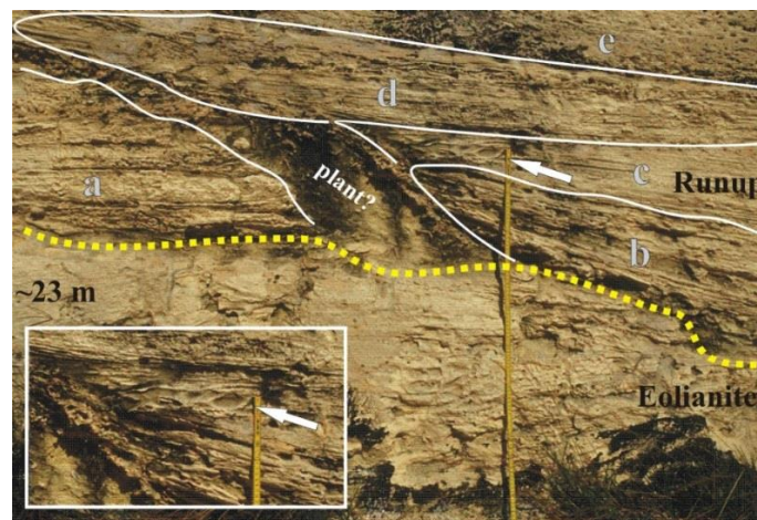
Fig. 23. Photograph of runup deposits in a road cutting above +23 m (1 m scale in photo) on Old Land Road, Great Exuma Island, situated deep in Exuma Sound ~200 km south of north Eleuthera. The older built-up eolianite forms the lower half of the image; the upper half has multiple "packages" of planar, fenestrae-filled beach sets. The upper progression of sedimentary packages (labelled a-e) clearly shows an onlapping, rising sequence of beds, indicating increasing wave energy and degree of runup. Further, the individual laminae of scour structures (arrows and inset image) display the same onlapping, upward climbing succession. It would be impossible to achieve such bedding if rain-saturated sediments were sloughing downhill on low angle slopes under the influence of gravity, especially near the crest of a ridge.
