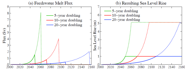
Fig. 5. (a) total fresh water flux added in North Atlantic and Southern Oceans, (b) resulting sea level rise. Solid lines for 1 m sea level rise, dotted for 5 m. One Sverdrup (Sv) is 10^6 \text{ m}^3/\text{s} , which is \sim 3 \times 10^4 \text{ Gt/year} .
