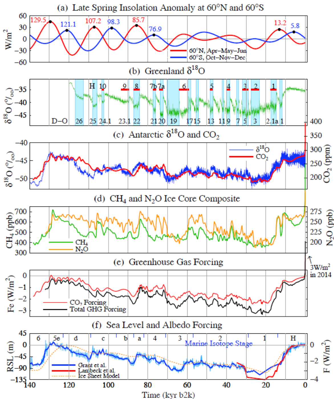
Fig. 27. (a) Late spring insolation anomalies relative to the mean for the past million years, (b) \delta^{18}O_{ice} of composite Greenland ice cores (Rasmussen et al., 2014) with Heinrich events of Guillevic et al. (2014), (c, d) \delta^{18}O_{ice} of EDML Antarctic ice core (Ruth et al., 2007), multi-ice core CO_2 , CH_4 , and N_2O based on spline fit with 1000-year cut-off (Schilt et al., 2010), scales are such that CO_2 and \delta^{18}O means coincide and standard deviations have the same magnitude, (e) GHG forcings from equations in Table 1 of Hansen et al. (2000), but with the CO_2 , CH_4 , and N_2O forcings multiplied by factors 1.024, 1.60, and 1.074, respectively, to account for each forcing's "efficacy" (Hansen et al., 2005a), with CH_4 including factor 1.4 to account for indirect effect on ozone and stratospheric water vapor, (f) sea level data from Grant et al. (2012) and Lambeck et al. (2014) and ice sheet model results from de Boer et al. (2010). Marine isotope stage boundaries from Lisiecki and Raymo (2005). (b-e) are on AICC2012 time scale (Bazin et al., 2013),
