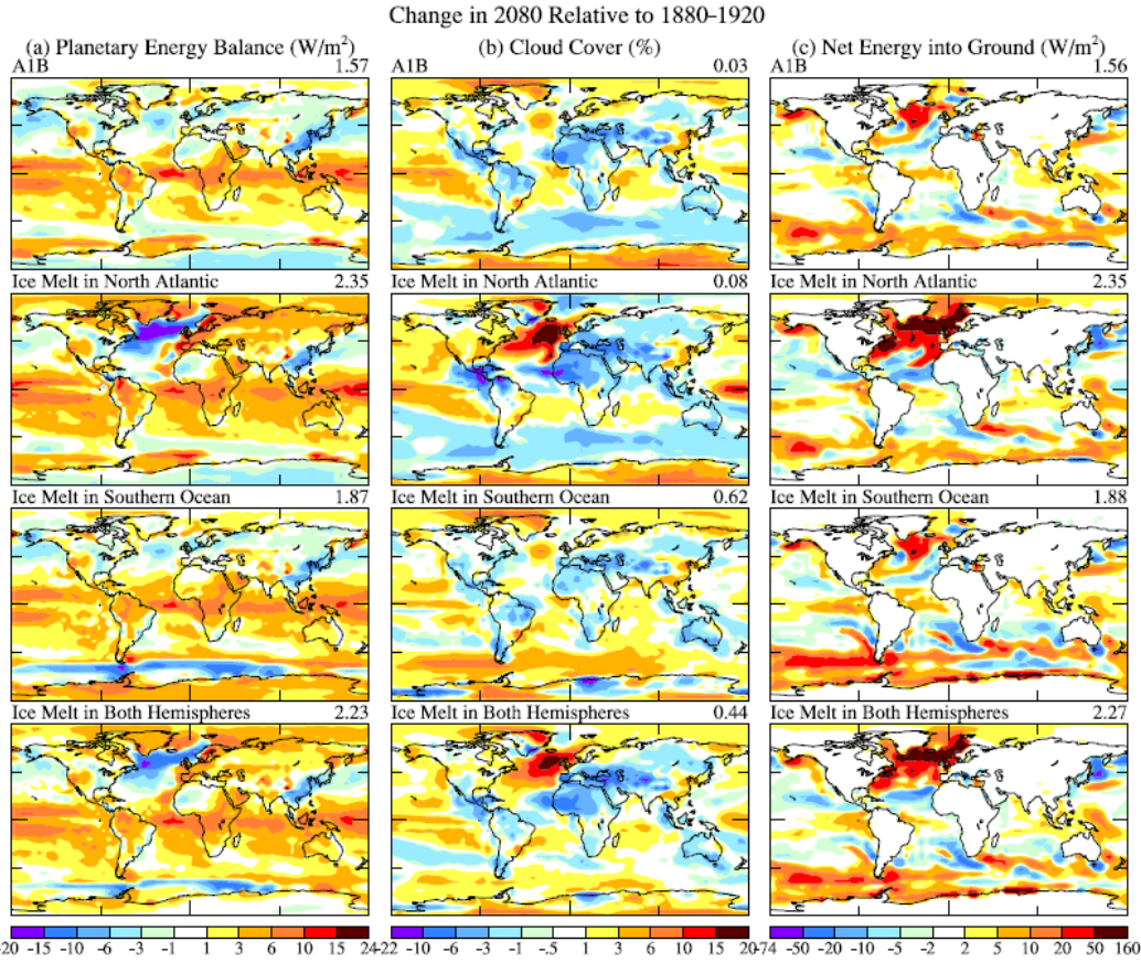
Fig. 8. Change in 2080 (mean of 2078-2082), relative to 1880-1920, of annual mean (a) planetary energy balance ( \text{W/m}^2 ), (b) cloud cover (%), and (c) net energy into ground ( \text{W/m}^2 ) for same scenarios as Fig. 6.
