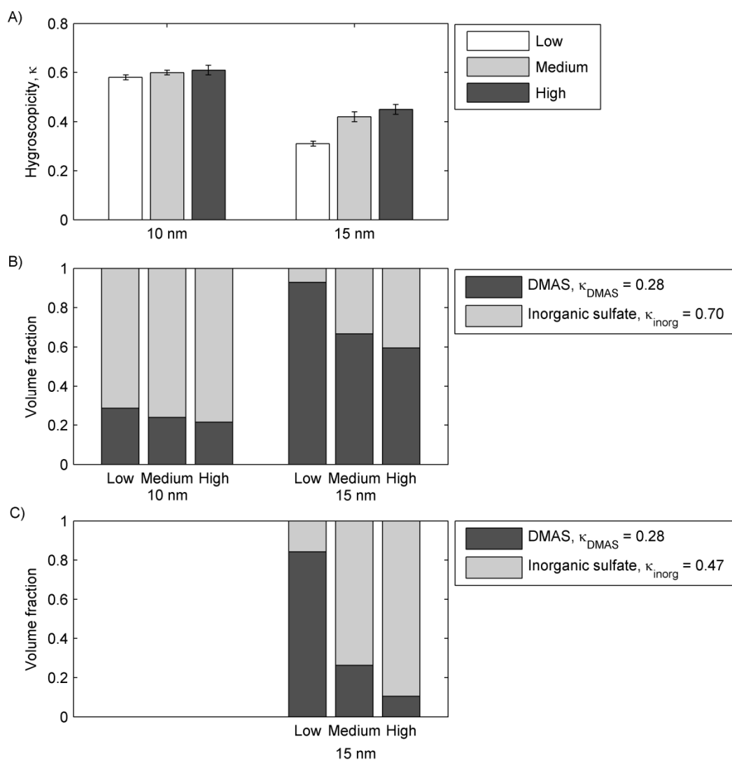
Fig. 3. (A) Comparison of hygroscopicity of 10 and 15 nm particles produced from sulfuric acid and dimethylamine; (B-C) Estimated volume fractions in the particles depending on UV aperture (Exp. B-D) assuming the inorganic fraction was (B) sulfuric acid and had a hygroscopicity \kappa = 0.70 and (C) ammonium sulfate and had a hygroscopicity \kappa = 0.47 . The concentrations of sulfuric acid were 5.1 \times 10^6 , 7.6 \times 10^6 , and 12.3 \times 10^6 molecules \text{cm}^{-3} for low, medium, and high, respectively.
