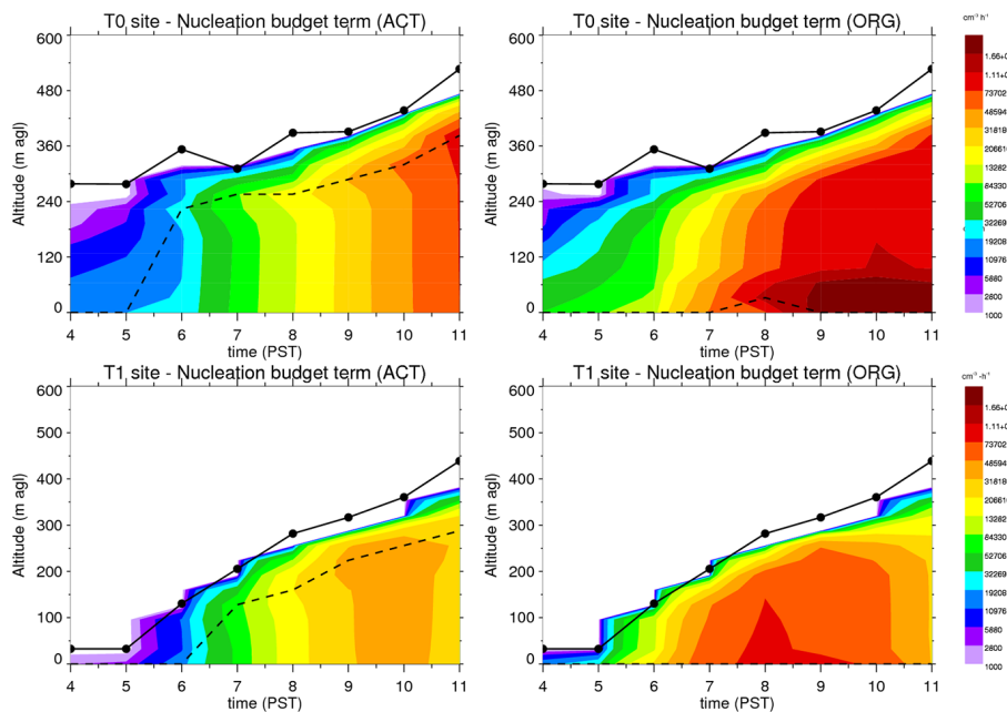
Figure 5. Particle production from the ACT and ORG parameterizations at the T0 and T1 sites on 8 June 2010 together with modeled BL height (circled line). The dashed line shows the altitude of maximum predicted number of small particles.
