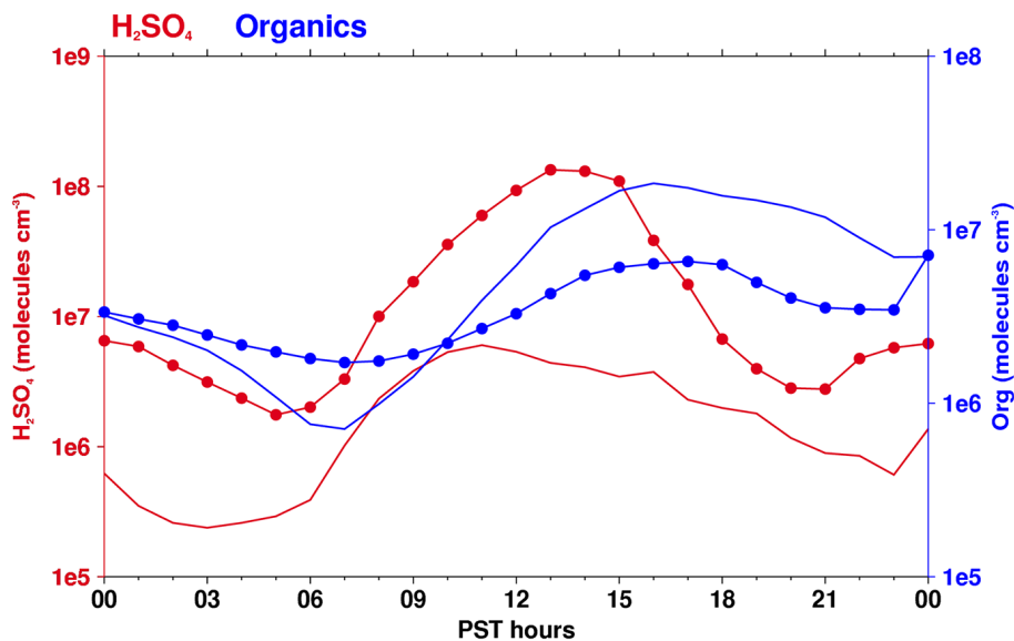
Figure 11. Modeled \text{H}_2\text{SO}_4 (red line), and organic gas concentrations (blue line) at the T0 site on 8 June 2010 (circled line) and 12 June 2010 (solid line).
