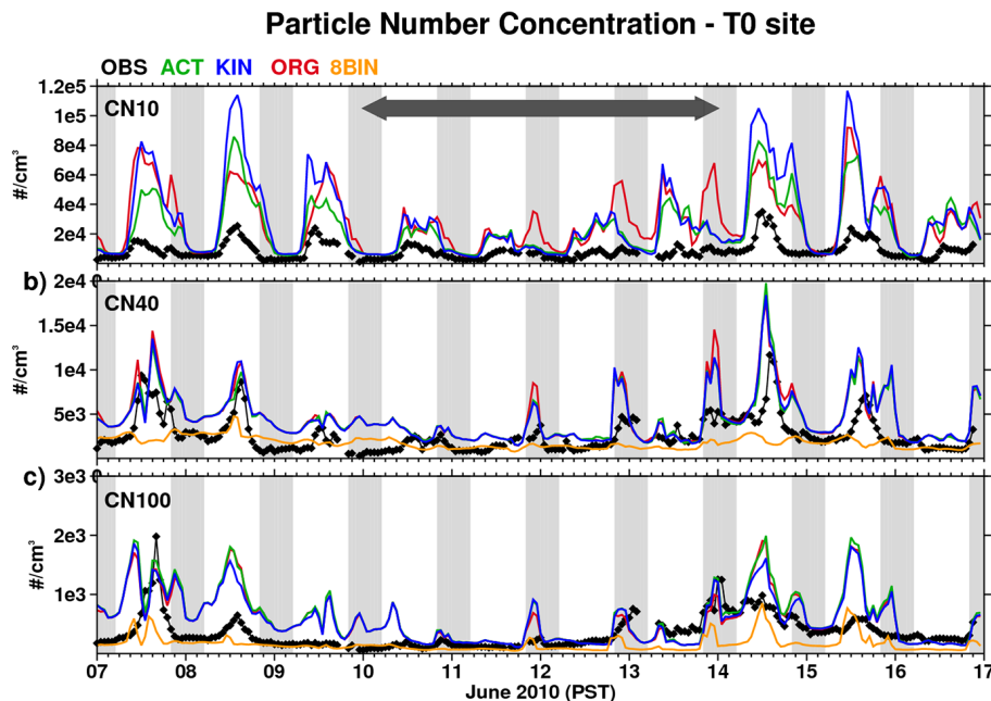
Figure 1. Observed and simulated time series of particle number concentration at the T0 site for (a) CN 10 ; (b) CN 40 ; (c) CN 100 . Gray shading indicates nighttime and the arrow denotes the period of northerly synoptic flow associated with the passage of a trough over California. All times are local Pacific Standard Time (PST).
