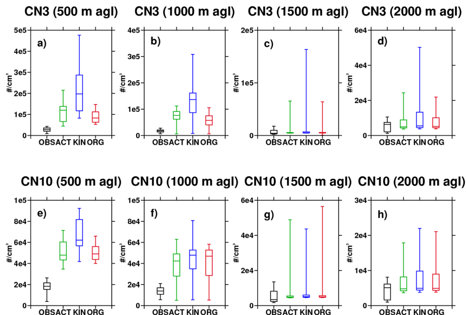
Figure 18. Boxplot for observed and simulated CN_3 and CN_{10} at the surface to 500 m altitude (a and e); 500–1000 m altitude (b and f) 1000–1500 m altitude (c and g); and 1500–2000 m altitude (d and h) for the 8 June 2010 afternoon G-1 flight. Observations are in black, ACT simulation values are in green, KIN in blue, and ORG in red. The line in the middle of each box is the median, while the boxes represent the 25th and 75th percentiles, and “whiskers” the 5th and 95th percentiles.
