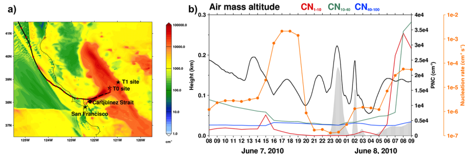
Figure 7. (a) Nucleation budget term ( \text{cm}^{-3} \text{h}^{-1} ) averaged over first five model layers from 05:00 to 09:00 PST 8 June 2010 from the ACT simulation, together with a backward trajectory from 08:00 PST on 7 June to 09:00 PST on 8 June 2010; the red dots denote the hourly locations of the air mass prior to its arrival at the T0; (b) Altitude of the air mass (black line) together with particle number concentration in 1–10 nm diameter range (red line), 10–40 nm range (green line), 40–100 nm range (blue line) and nucleation rate (orange circled line); the gray area denotes the terrain height.
