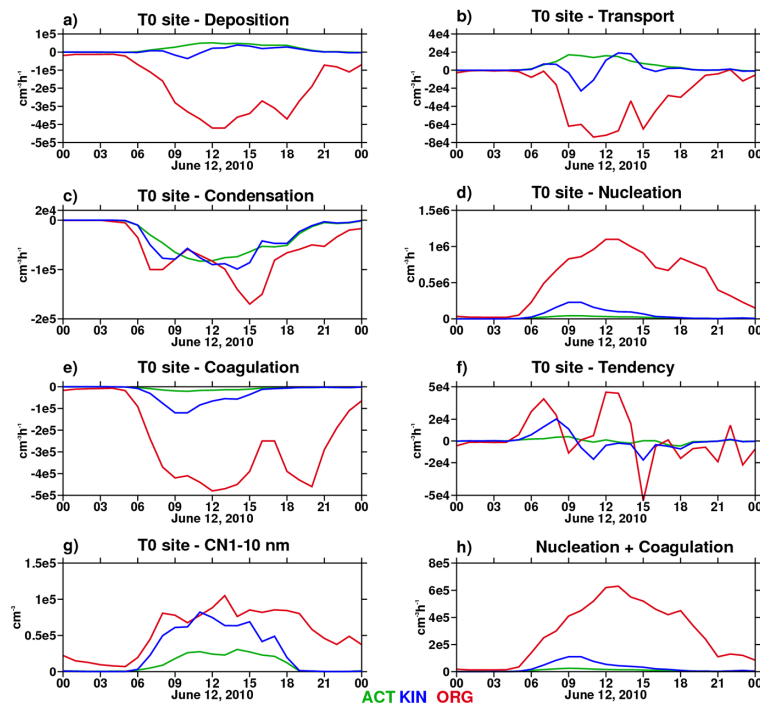
Figure 15. Budget diagnostic terms for 1–10 nm particles at the T0 site on 12 June: (a) deposition; (b) transport; (c) condensation; (d) nucleation; (e) coagulation; (f) total tendency; (g) particle number concentration in 1 to 10 nm range; and (h) tendency of particles coming from nucleation and coagulation processes.
