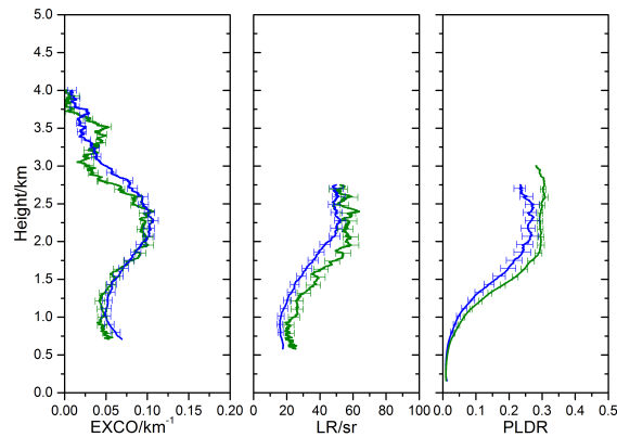
Figure 5. Profiles of the particle extinction coefficient (EXCO) and the lidar ratio (LR), and of the particle linear depolarization ratio (PLDR) of the pure dust layer at 355 nm (blue) and 532 nm (green) on 20 June 2013, 23:30–24:00 UTC. The error bars indicate the systematic errors.
