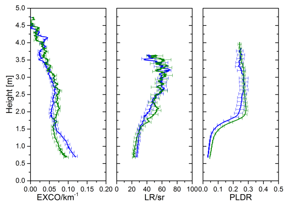
Figure 7. Same as Fig. 5 but for 27 June 2013, 00:00–02:00 UTC.
