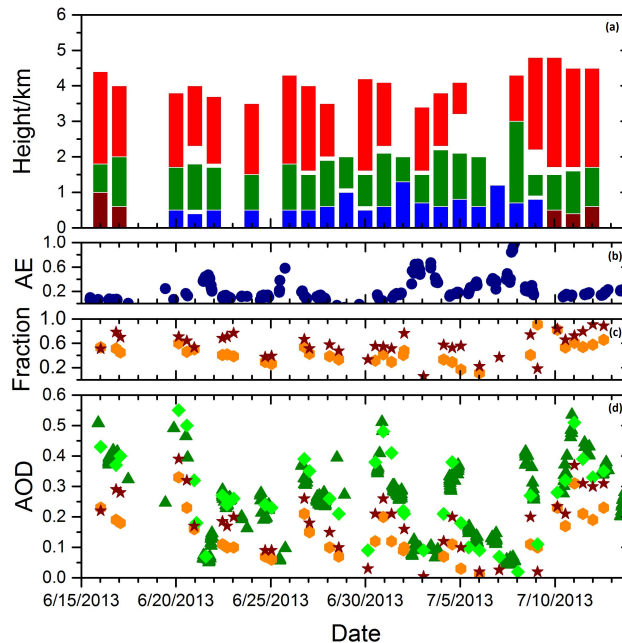
Figure 1. Time series of (a) aerosol layering during SALTRACE derived from POLIS lidar measurements during the evening measurement sessions (red indicates Saharan dust dominated aerosol layers, green indicates intermediate or mixed aerosol layers, blue indicates marine dominated aerosol layers and brown indicates mixtures of Saharan dust and marine aerosols), (b) Angström exponents between 440 and 870 nm (blue dots) from CIMEL sun-photometer measurements, (c) the fraction of pure dust optical depth (orange) and total dust optical depth (brown stars) to the total AOD, and (d) aerosol optical depth (AOD) at 500 nm derived from CIMEL sun-photometer measurements (dark green) and at 532 nm derived from POLIS lidar measurements (light green) and optical depth of the pure dust layer (orange) and of the whole dust contribution in the atmospheric column (brown stars) at 532 nm derived from POLIS lidar measurement.
