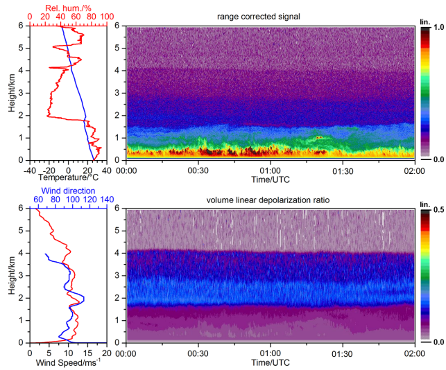
Figure 6. Same as Fig. 4 but for 27 June 2013, 00:00–02:00 UTC. The radiosonde was launched on 27 June at 00:24 UTC.
