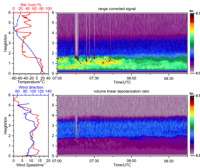
Figure 8. Same as Fig. 4 but for 01 July 2013, 07:00–08:45 UTC. The radiosonde was launched on 01 July at 00:00 UTC.
