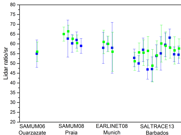
Figure 13. Mean values of the lidar ratio of Saharan dust at 355 nm (blue) and 532 nm (green) derived for fresh Saharan dust (mean campaign value) during SAMUM-1 in Ouarzazate, Morocco in 2006 (SAMUM06) (Tesche et al., 2009b), for mid-range transported Saharan dust on 5 days during SAMUM-2 at Cape Verde in 2008 (SAMUM08) (Groß et al., 2011b), for long-range transported dust over Central Europe on 3 days at Munich, Germany in 2008 (EARLINET08) (Wiegner et al., 2011), and for long-range transported Saharan dust over the Caribbean on 10 days during SALTRACE at Barbados in 2013 (SALTRACE13). The error bars denote the systematic errors.
