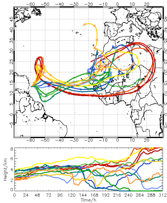
Figure 2. 312 h backward trajectories calculated with the Hybrid Single Particle Lagrangian Integrated Trajectory (HYSPPLIT) model (Draxler and Rolph, 2012) and GDAS meteorological data for the pure dust layers on 20 June 2013, 23:00 UTC (reddish), 27 June 2013, 01:00 UTC (blueish), 01 July 2013, 08:00 UTC (greenish), and 11 July, 23:00 UTC (yellowish). The stars along the trajectories indicate 24 h time steps. The height range of the pure dust layers is indicated in Table 1.
