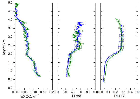
Figure 9. Same as Fig. 5 but for 01 July 2013, 07:00–08:45 UTC.
