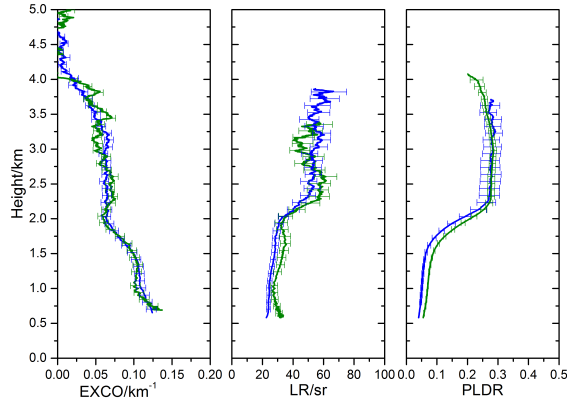
Figure 11. Same as Fig. 5 but for 11 July 2013, 23:00–24:00 UTC.
