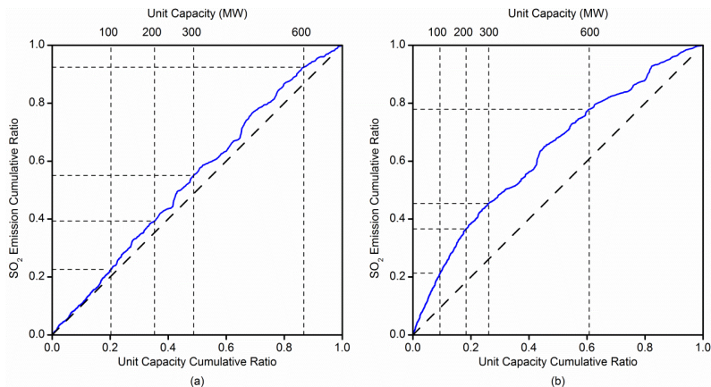
Figure 7. Cumulative ratio of SO 2 emissions by unit capacity for the years (a) 2005 and (b) 2010. The units are sorted according to ascending capacity along the x axis.
