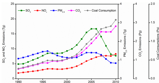
Figure 4. Coal consumptions and emissions of SO 2 , NO x , PM 2.5 and CO 2 of coal-fired power plants in China from 1990 to 2010.
