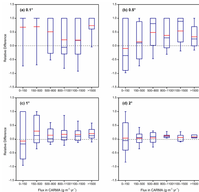
Figure 14. Comparisons of CO 2 emissions between CARMA and CPED for various spatial resolutions (from 0.1 to 2°) in 2009. The box plots show the binned relative differences (a - b)/(a + b) , where a is the CARMA estimate, and b is the CPED estimate. The blue horizontal line is the median of the relative differences, the red horizontal line is the mean of the relative differences, the box denotes the 25 and 75 % percentiles, and the whiskers denote the 10 and 90 % percentiles. A perfect agreement would correspond to a median and mean equal to zero.
