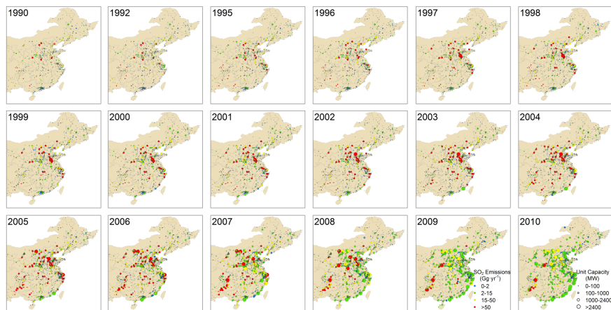
Figure 9. Evolution of \text{SO}_2 emissions from coal-fired power plants in China, 1990–2010. Units: \text{Gg yr}^{-1} .
