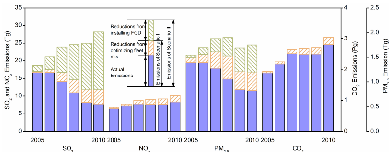
Figure 8. Reductions in SO 2 , NO x , PM 2.5 and CO 2 emissions from major emission control measures during the 11th five-year period (2005–2010). The solid blue bar denotes our estimates of inter-annual power plant emissions. The green and yellow bars illustrate the reduction in emissions due to FGD installations and optimization of the generation unit fleet mix, respectively.
