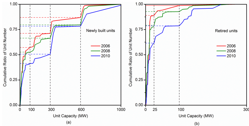
Figure 2. Cumulative ratio of unit number for (a) newly constructed and (b) retired electric generating units for 2006, 2008 and 2010. The units are sorted according to ascending capacity along the x axis.
