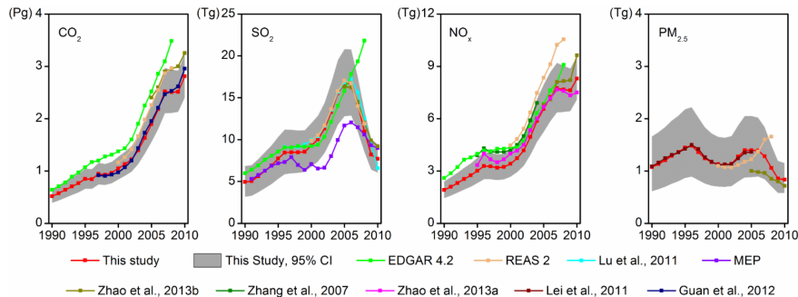
Figure 12. Comparisons of SO 2 , NO x , PM 2.5 and CO 2 emissions from China's coal-fired power plants during 1990 and 2010.
