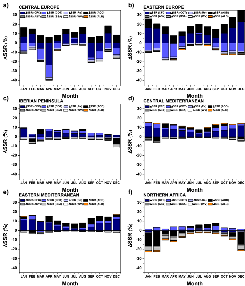
Figure 10. ΔSSR (%) caused by CFC, COT, Re, AOD, ASY, SSA, WV and ALB for (a) CE, (b) EE, (c) IP, (d) CM, (e) EM and (f) NA.
