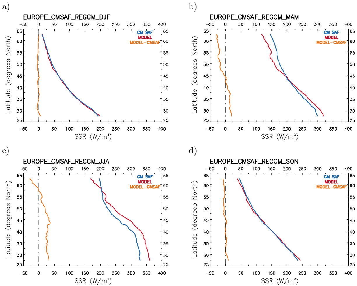
Figure S4. Latitudinal variability of RegCM4 SSR (red), CM SAF SSR (blue) and their difference (orange) over Europe for (a) winter (DJF), (b) spring (MAM), (c) summer (JJA) and (d) autumn (SON) from MFG MVIRI observations.
