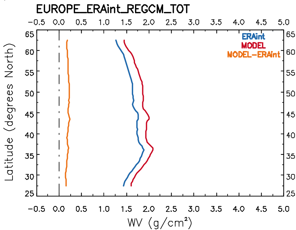
Figure S17. (a) NMB patterns of RegCM4-ERA-Interim WV and (b) Latitudinal variability of RegCM4 WV (red), ERA-Interim WV (blue) and their difference (orange) over Europe.
