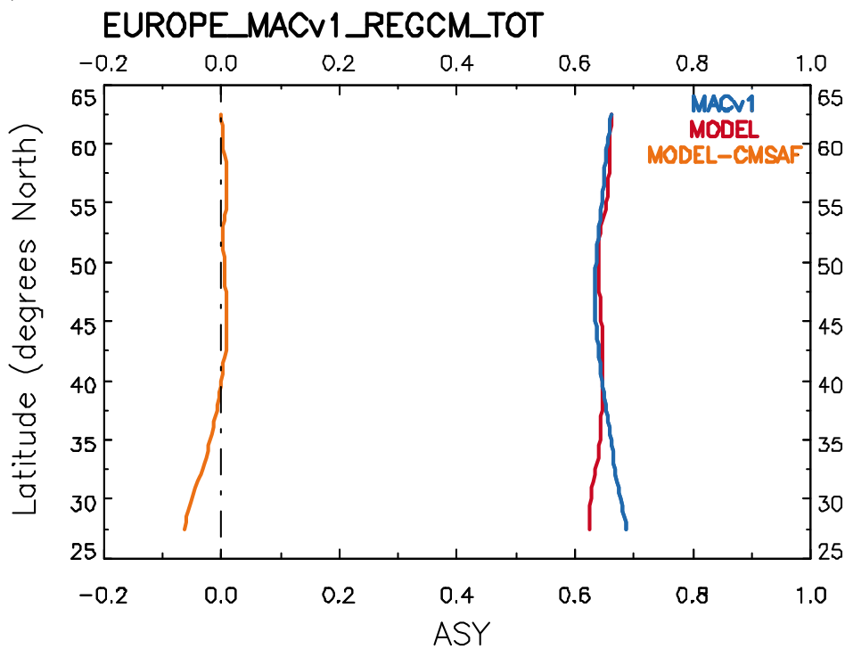
Figure S13. (a) NMB patterns of RegCM4-MACv1 ASY and (b) Latitudinal variability of RegCM4 ASY (red), MACv1 ASY (blue) and their difference (orange) over Europe.
