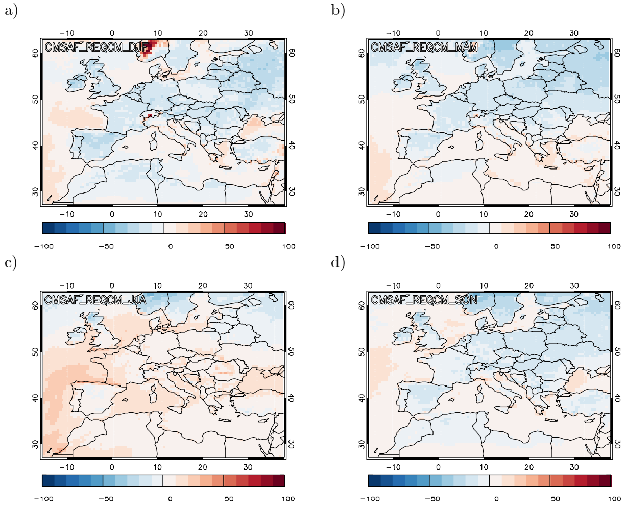
Figure S3. Seasonal Normalized mean bias (NMB) patterns of RegCM4-CM SAF SSR over Europe for (a) winter (DJF), (b) spring (MAM), (c) summer (JJA) and (d) autumn (SON) from MFG MVIRI observations.
