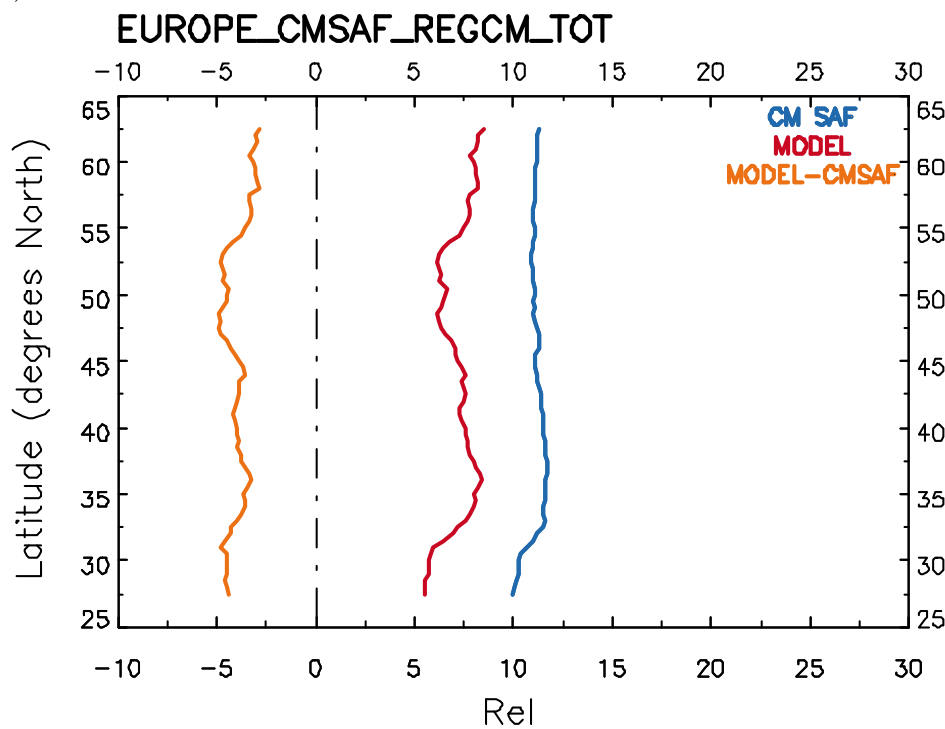
Figure S6. (a) NMB patterns of RegCM4-CM SAF Rel and (b) Latitudinal variability of RegCM4 Rel (red), CM SAF Rel (blue) and their difference (orange) over Europe from MSG SEVIRI observations.
