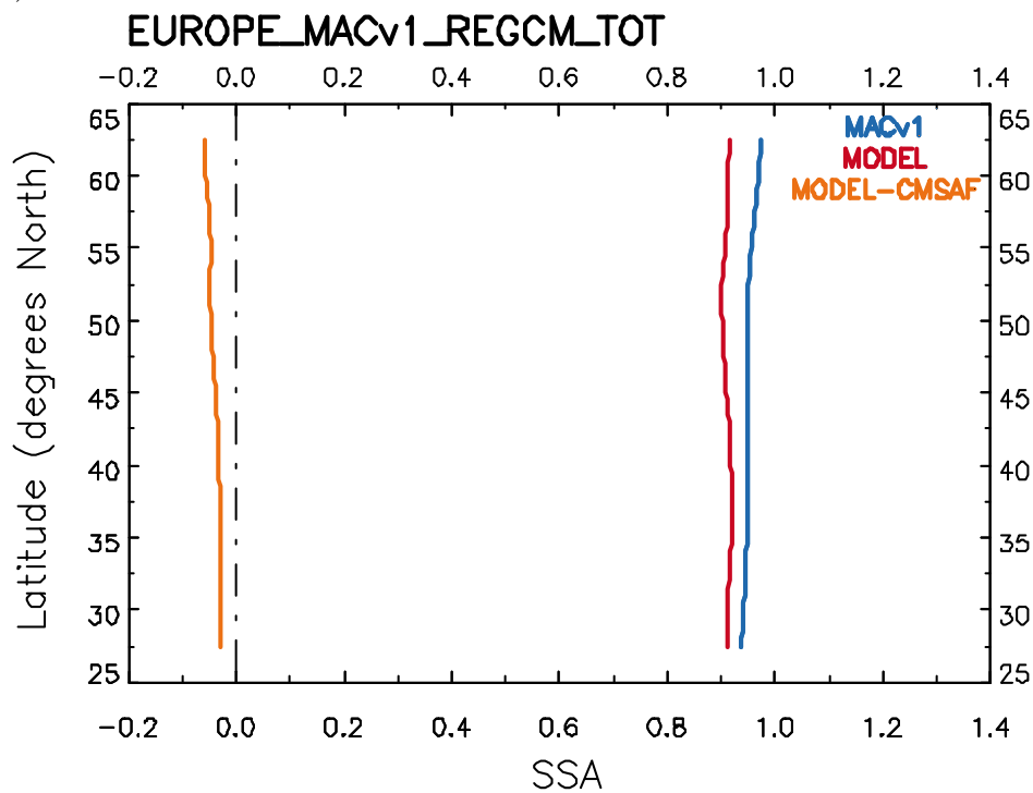
Figure S15. (a) NMB patterns of RegCM4-MACv1 SSA and (b) Latitudinal variability of RegCM4 SSA (red), MACv1 SSA (blue) and their difference (orange) over Europe.
