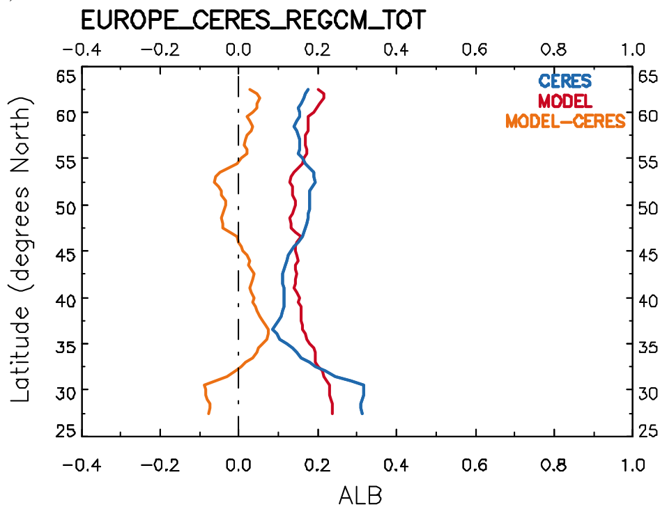
Figure S19. (a) NMB patterns of RegCM4-CERES ALB and (b) Latitudinal variability of RegCM4 ALB (red), CERES ALB (blue) and their difference (orange) over Europe.
