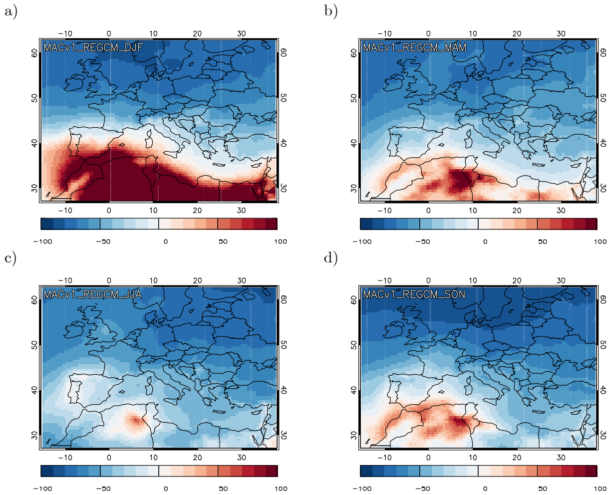
Figure S10. Seasonal Normalized mean bias (NMB) patterns of RegCM4-MACv1 AOD 550 over Europe for (a) winter (DJF), (b) spring (MAM), (c) summer (JJA) and (d) autumn (SON).
