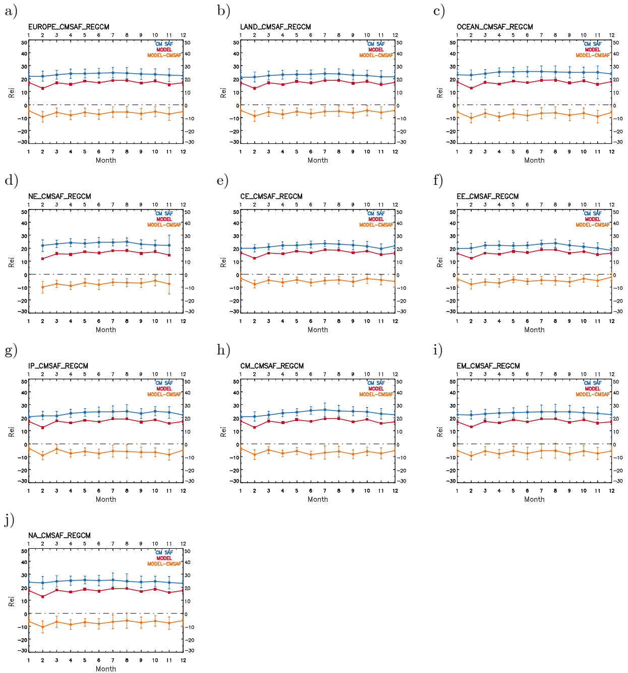
Figure S9. Seasonal variability of RegCM4 Re i (red), CM SAF Re i (blue) and their difference (orange) over (a) the whole Europe, (b) Land, (c) Ocean, (d) NE, (e) CE, (f) EE, (g) IP, (h) CM, (i) EM, (j) NA from MSG SEVIRI observations.
