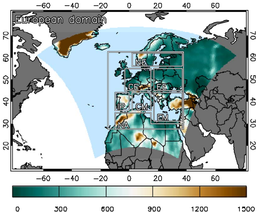
Figure S1. Topography of the RegCM4 simulation domain with the European box region and the 7 sub-regions used for the generalization of the results: Northern Europe (NE), Central Europe (CE), Eastern Europe (EE), Iberian Peninsula (IP), Central Mediterranean (CM), Eastern Mediterranean (EM) and Northern Africa (NA).
