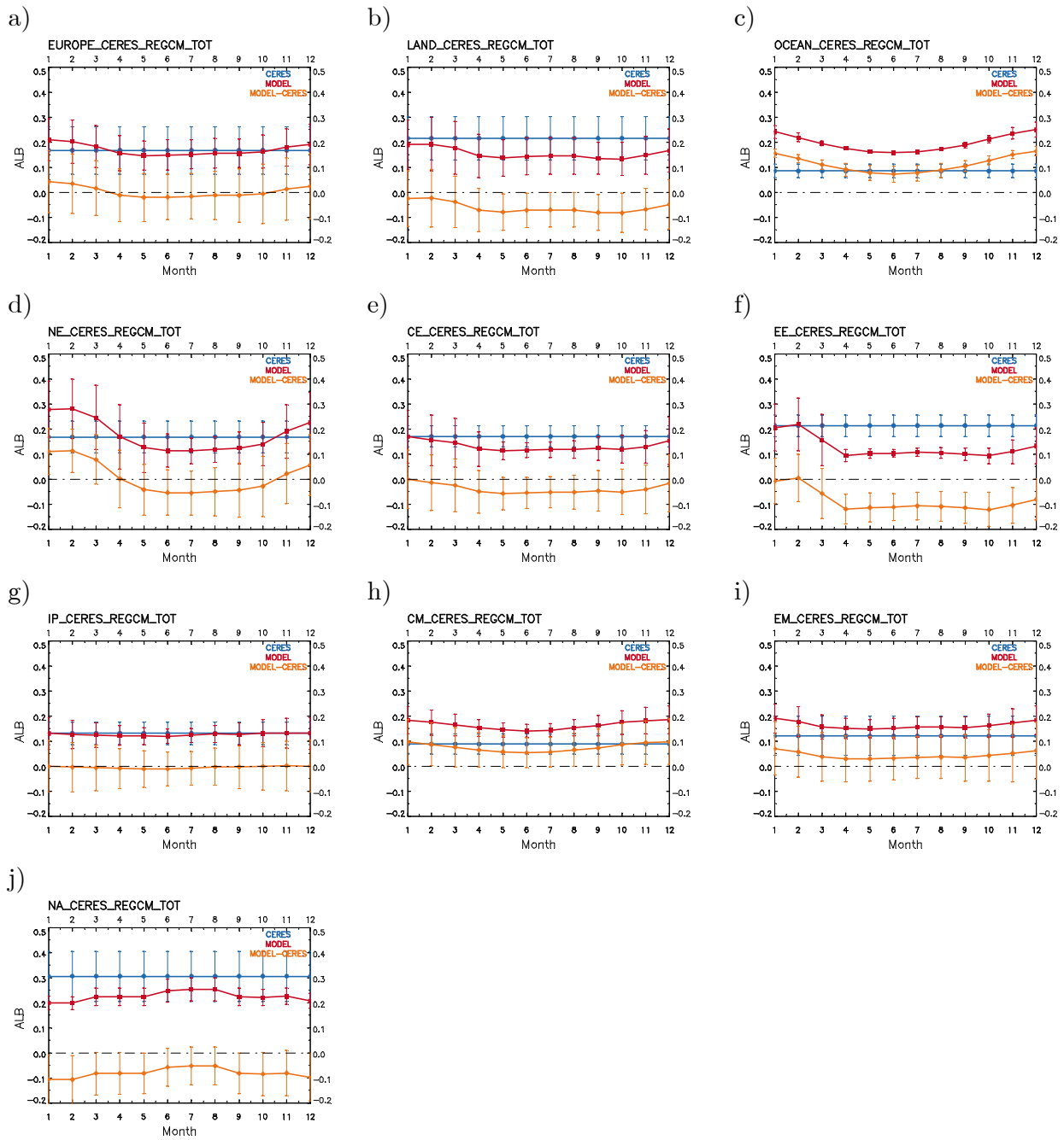
Figure S20. Seasonal variability of RegCM4 ALB (red), CERES ALB (blue) and their difference (orange) over (a) the whole Europe, (b) Land, (c) Ocean, (d) NE, (e) CE, (f) EE, (g) IP, (h) CM, (i) EM, (j) NA.
