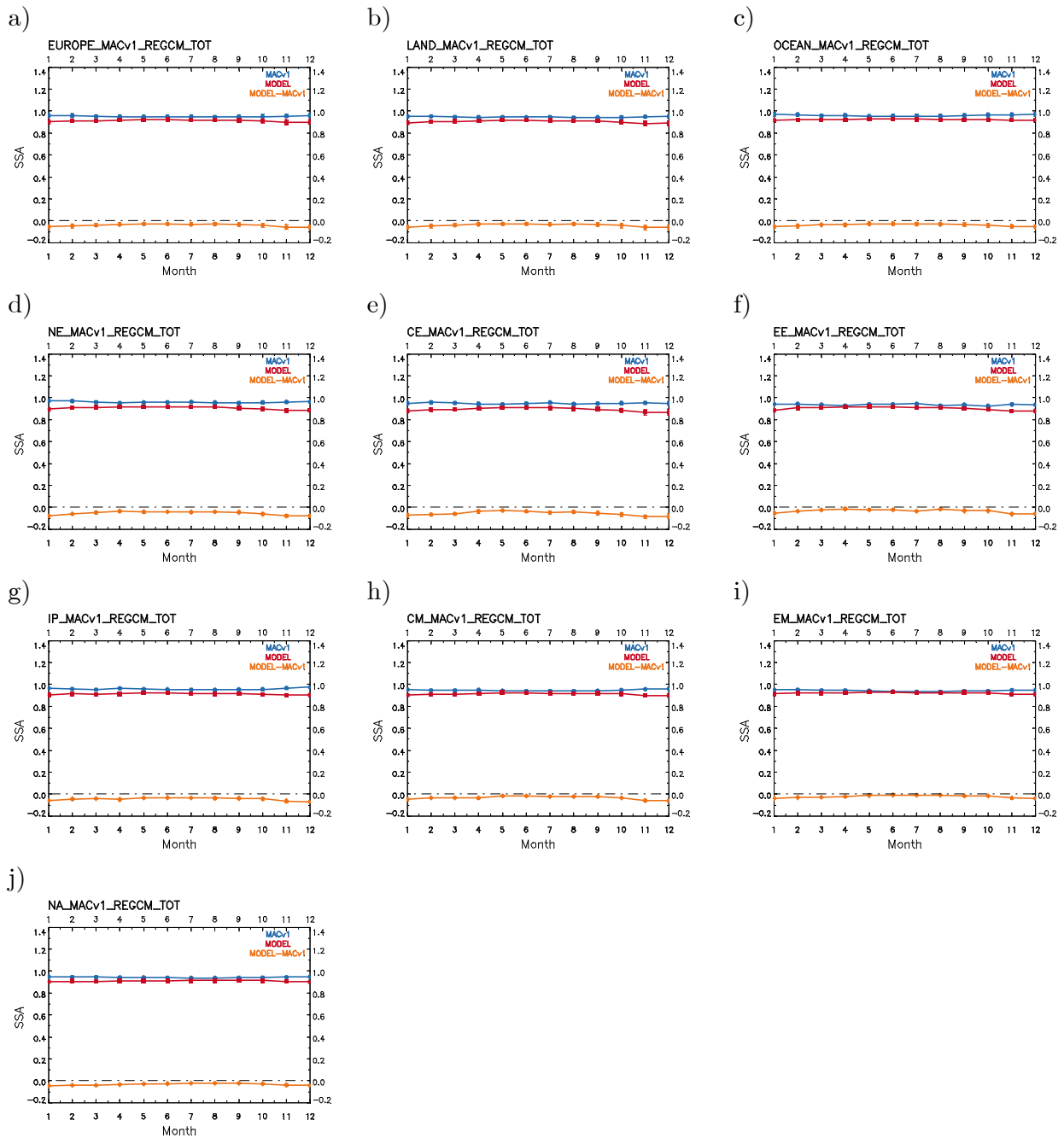
Figure S16. Seasonal variability of RegCM4 SSA (red), MACv1 SSA (blue) and their difference (orange) over (a) the whole Europe, (b) Land, (c) Ocean, (d) NE, (e) CE, (f) EE, (g) IP, (h) CM, (i) EM, (j) NA.
