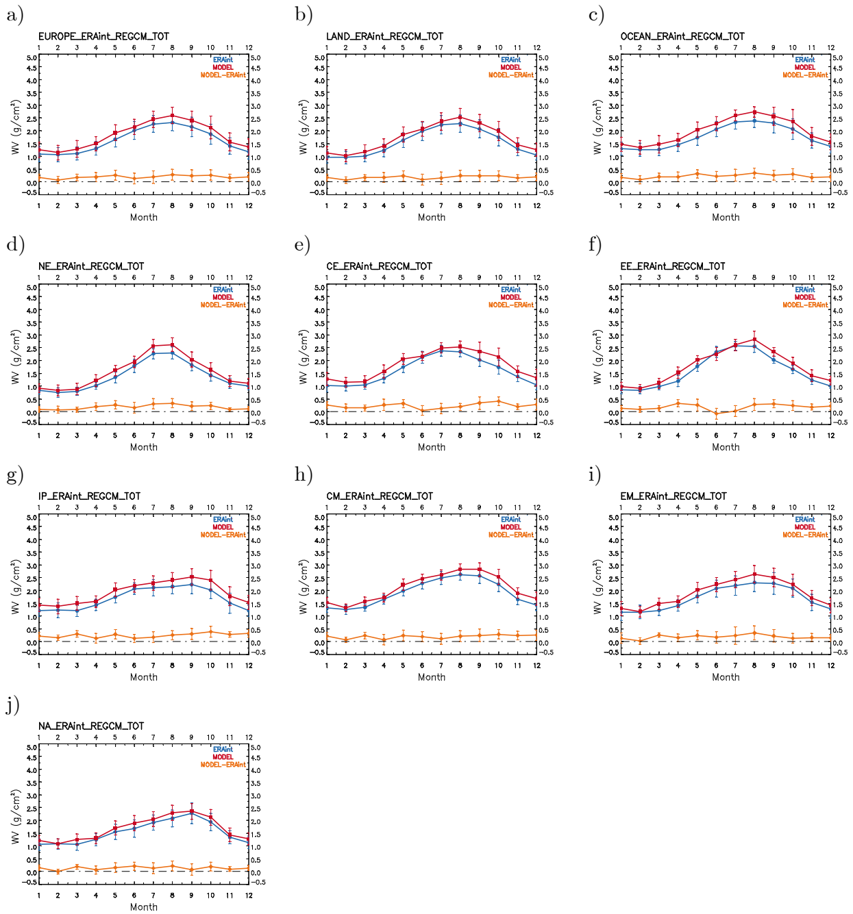
Figure S18. Seasonal variability of RegCM4 WV (red), ERA-Interim WV (blue) and their difference (orange) over (a) the whole Europe, (b) Land, (c) Ocean, (d) NE, (e) CE, (f) EE, (g) IP, (h) CM, (i) EM, (j) NA.
