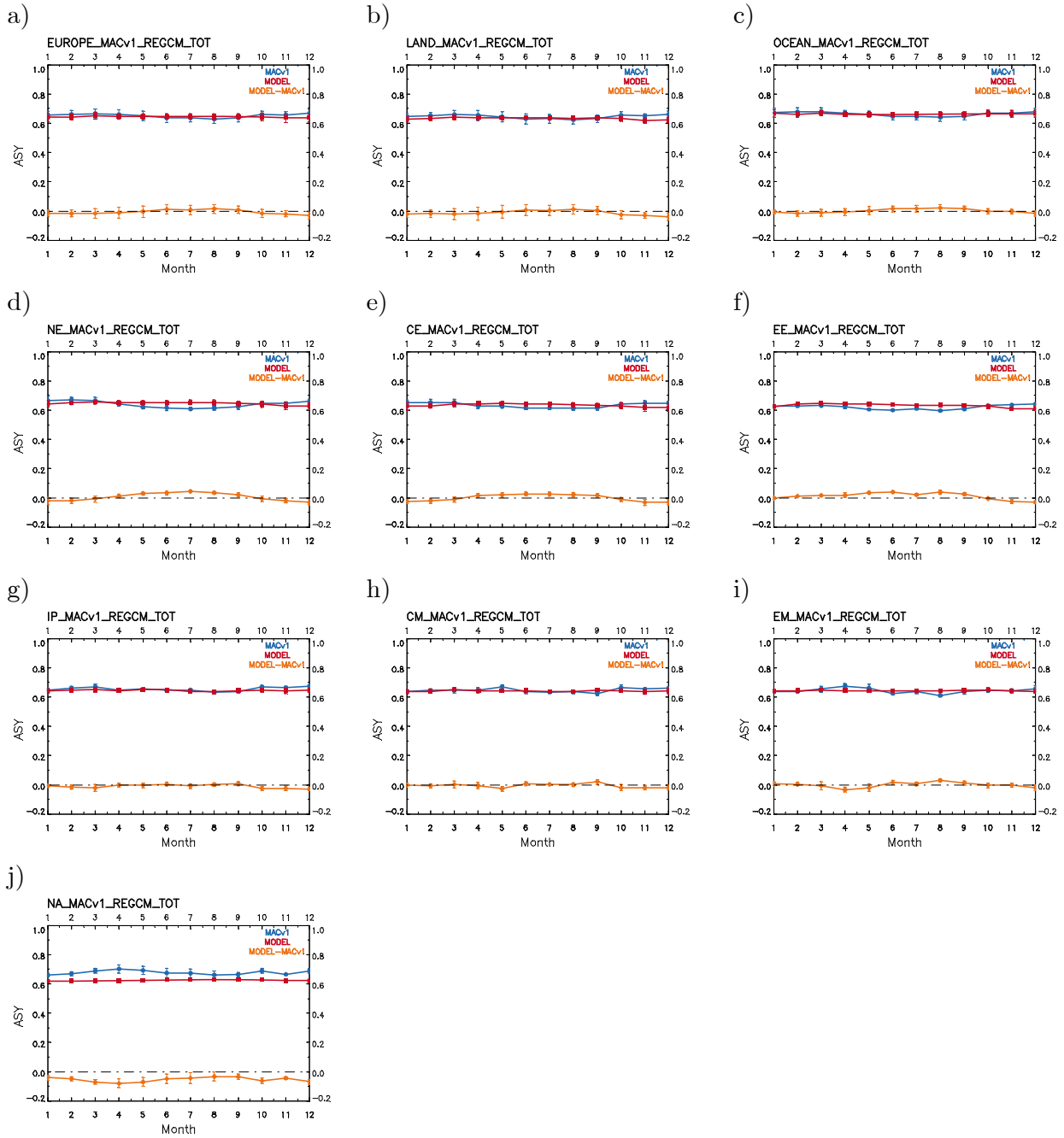
Figure S14. Seasonal variability of RegCM4 ASY (red), MACv1 ASY (blue) and their difference (orange) over (a) the whole Europe, (b) Land, (c) Ocean, (d) NE, (e) CE, (f) EE, (g) IP, (h) CM, (i) EM, (j) NA.
