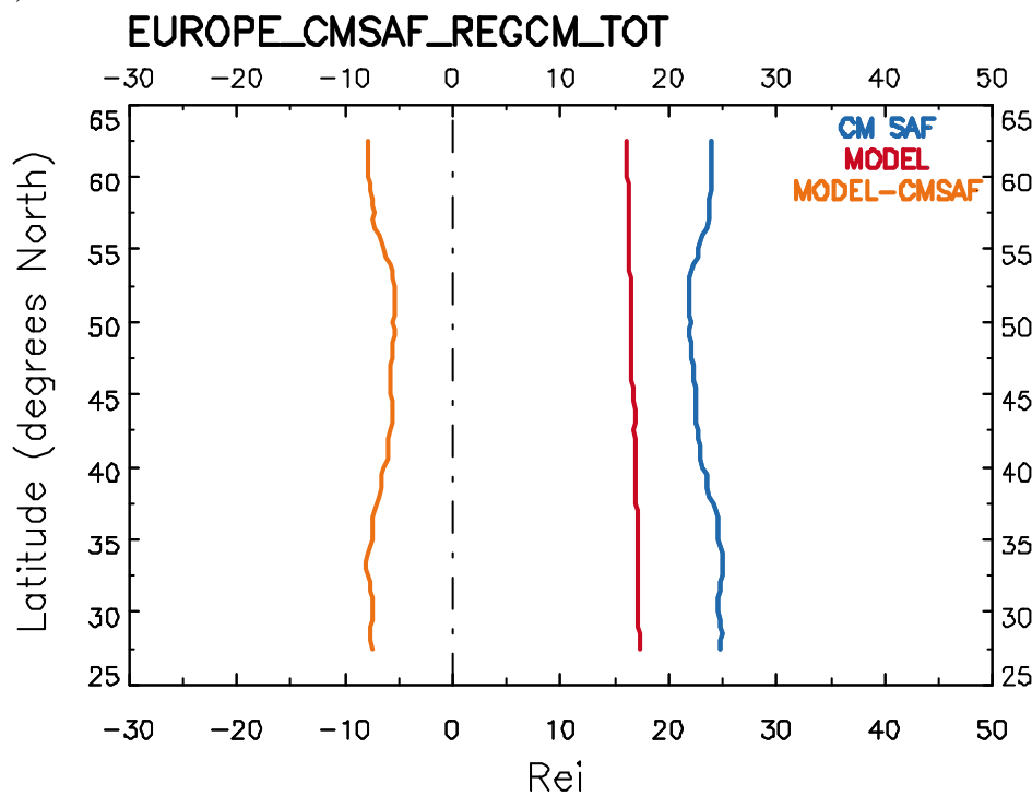
Figure S8. (a) NMB patterns of RegCM4-CM SAF Rei and (b) Latitudinal variability of RegCM4 Rei (red), CM SAF Rei (blue) and their difference (orange) over Europe from MSG SEVIRI observations.
