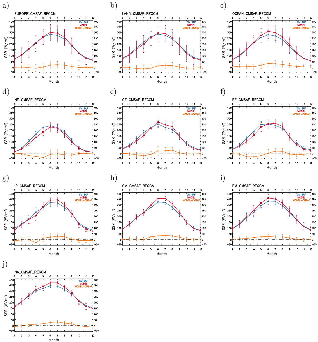
Figure S5. Seasonal variability of RegCM4 SSR (red), CM SAF SSR (blue) and their difference (orange) over (a) the whole Europe, (b) Land, (c) Ocean, (d) NE, (e) CE, (f) EE, (g) IP, (h) CM, (i) EM, (j) NA from MFG MVIRI observations.
