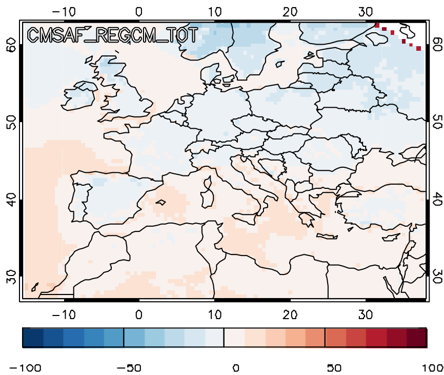
Figure S2. Normalized mean bias (NMB) patterns of RegCM4-CM SAF SSR over Europe from (a) MFG MVIRI (2000-2005) and (b) MSG SEVIRI (2006-2009) observations.
