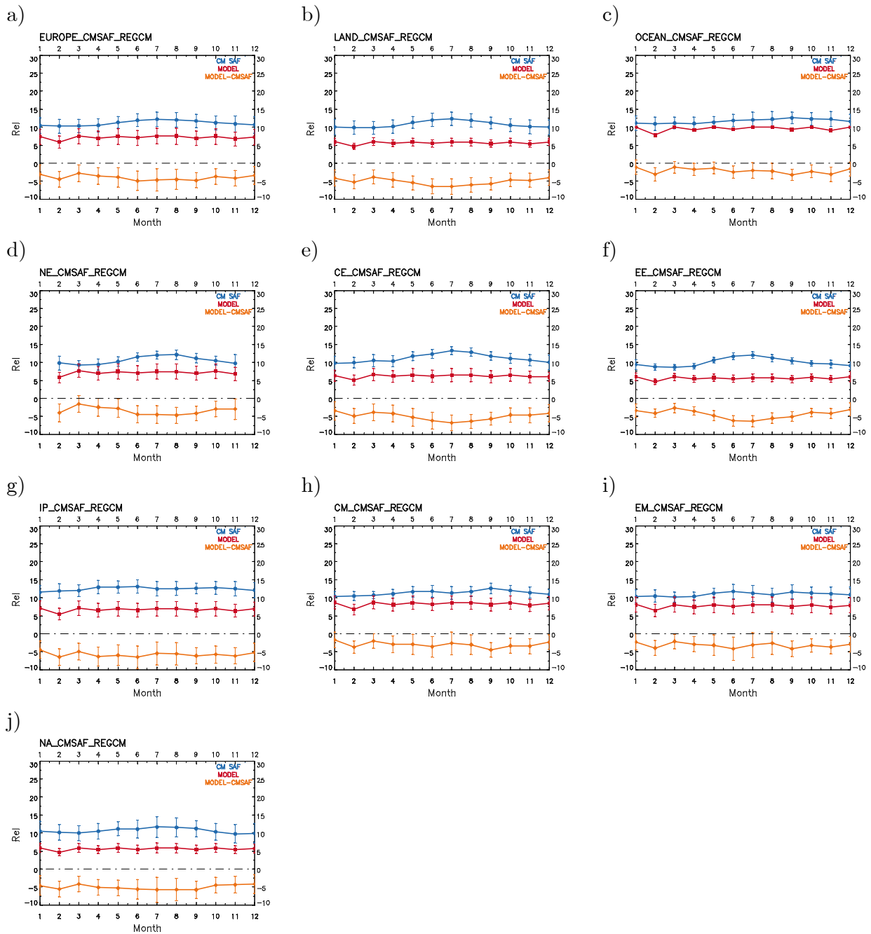
Figure S7. Seasonal variability of RegCM4 Rel (red), CM SAF Rel (blue) and their difference (orange) over (a) the whole Europe, (b) Land, (c) Ocean, (d) NE, (e) CE, (f) EE, (g) IP, (h) CM, (i) EM, (j) NA from MSG SEVIRI observations.
