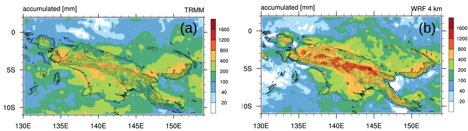
Figure 2. Accumulated rainfall (mm) and daily mean rainfall rate ( \phi ) for the New Guinea region between 02–28 February 2010 from TRMM (a, c) (a) and the 4 km WRF simulation (b, d) (b). Data from WRF have been coarse-grained to match the data resolution of the TRMM 3B42 gridded product.
