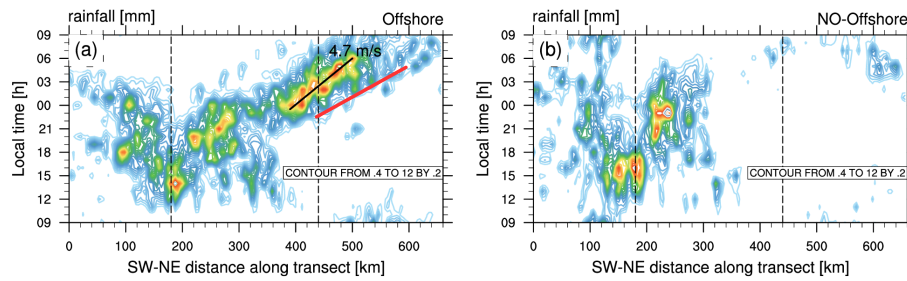
Figure 6. Composite diurnal cycle in local time (LT) in simulated (a) Offshore and (b) NO-Offshore days, as averaged across the line sections seen in Fig. 1a. The black line represents the estimated phase speed of the peak rain signal across the northern coast, while the red line denotes the estimated phase speed of the broader rain envelope ( \sim 8 \text{ m s}^{-1} ).
