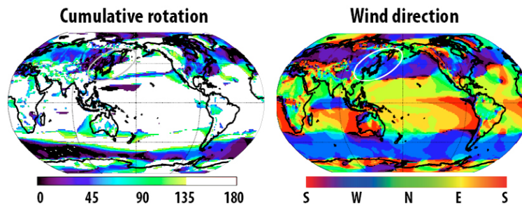
Figure 8. Cumulative rotation of wind from 975 hPa to 30 hPa (left) and prevailing wind direction at 975 hPa (right). Computed from JRA-55 for November 2008.
