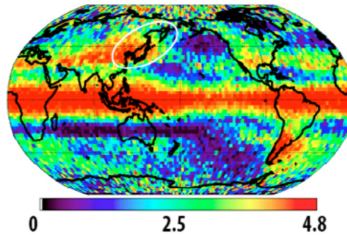
Figure 3. Annual mean of the potential energy in J/kg averaged across the whole vertical profile for 2007–2010 (non-linear color scale used).
