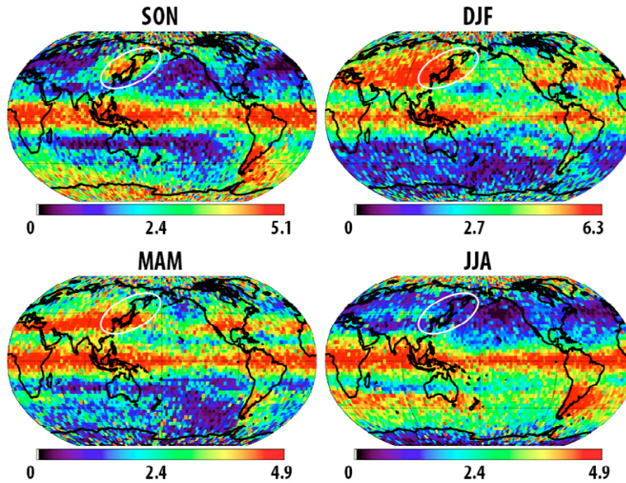
Figure 4. Seasonal means of the potential energy in J/kg averaged across the whole vertical profile for 2007–2010 (non-linear color scale used).
