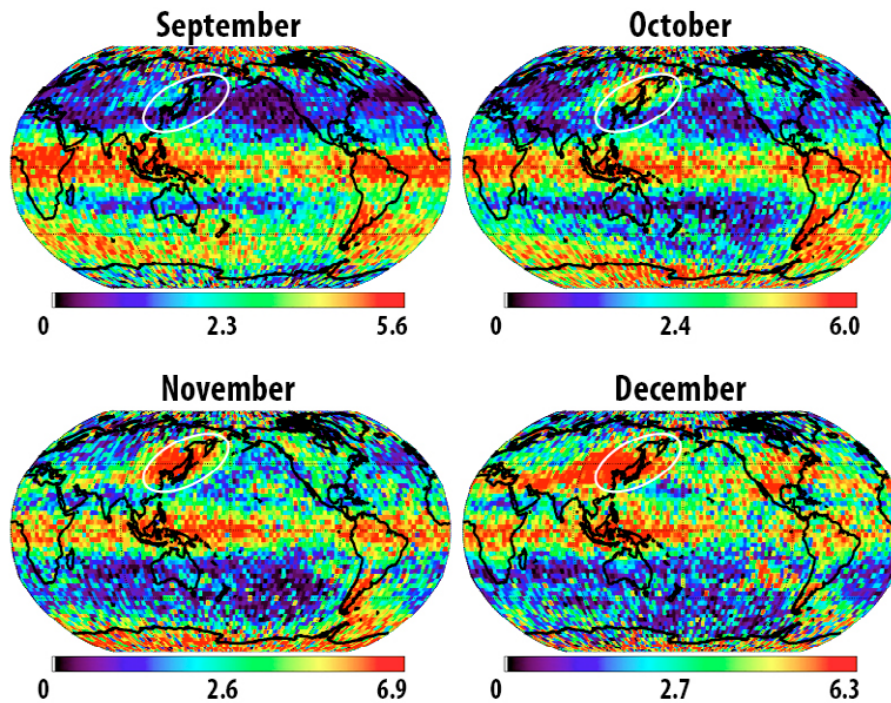
Figure 5. Selected monthly means of the potential energy in J/kg averaged across the whole vertical profile for 2007–2010 (non-linear color scale used).
