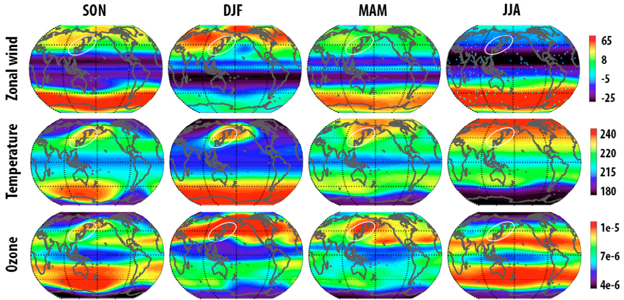
Figure 2. Seasonal averages of zonal wind in m/s, temperature in K and ozone mass mixing ratio in mg/kg for 1979-2013 using MERRA reanalysis (non-linear color scale used).
