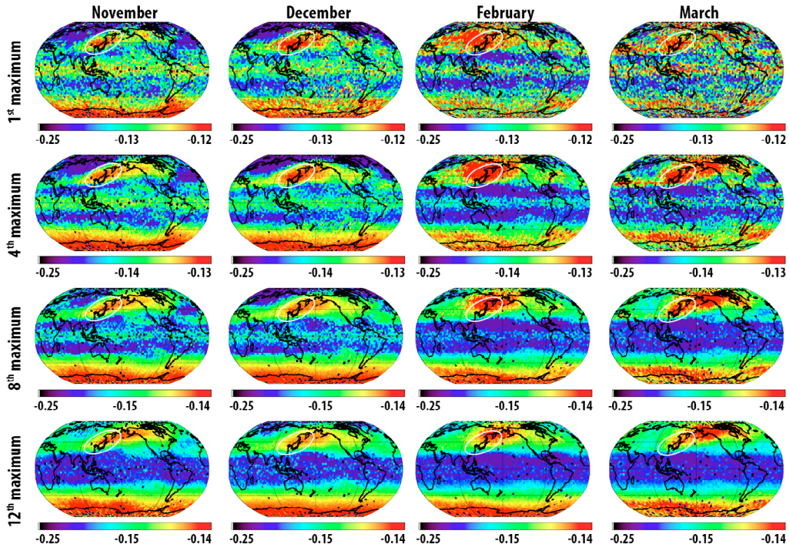
Figure 7. Selected monthly means of primary and selected secondary (i.e., higher order) sigma squared maxima in s^{-2} for 2007–2010 (non-linear color scale used).
