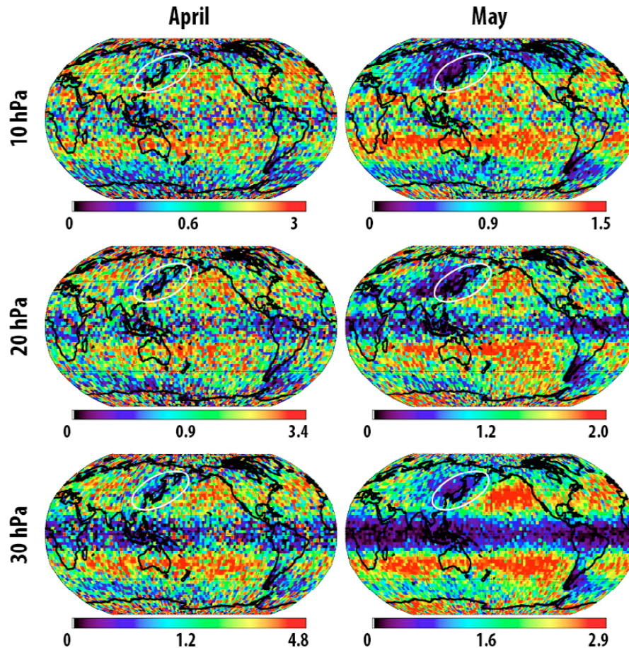
Figure 6. Selected monthly means of the gradient Richardson number at 10, 20 and 30 hPa for 2007–2010 (non-linear color scale used).
