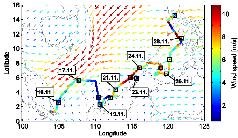
Figure 1: ERA-Interim mean wind field November 15-30, 2011 (arrows) and 10 minute running mean of wind speed observed on R/V SONNE as the cruise track. The black squares show the ships position at 00 UTC each day.
