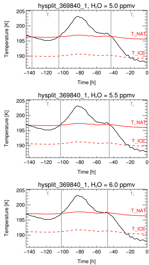
Figure 6. Same as Fig. 5 but with an additional temperature decrease along the back trajectory of 1 K.
