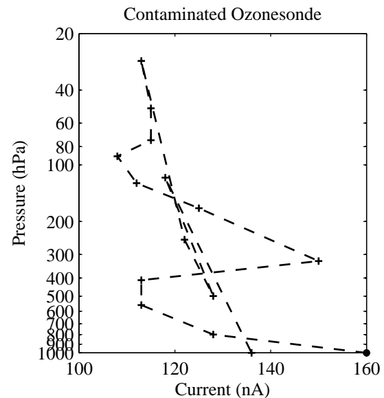
Fig. A1. Current measured at each pressure for the contaminated ozonesonde. The dashed line shows the order in which the measurements were taken, starting from (1000 hPa, 160 nA) (the ● data-point).
