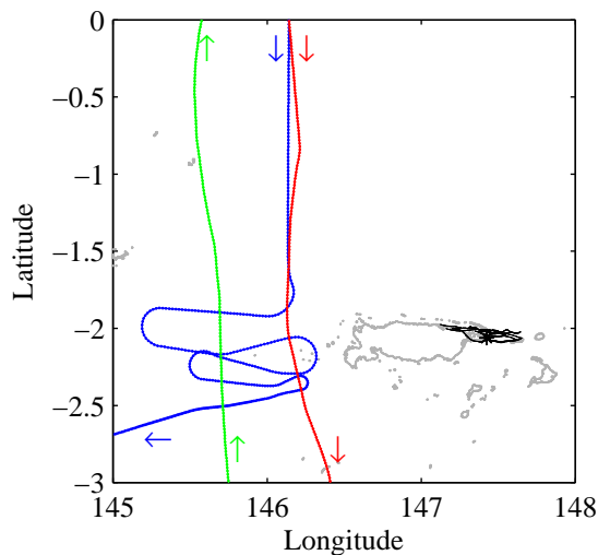
Fig. 3. Map of the co-located measurements of Gulfstream V flights RF09 and RF14, and CAST ozonesondes 6, 34 and 35. The blue flightpath is RF09, the red is the outbound leg of RF14 and green is the return leg of RF14. The black lines are the flightpaths of ozonesondes 6, 34 and 35, which all remained in the east of Manus Island at all times. The arrows show the direction of travel of the Gulfstream V.
