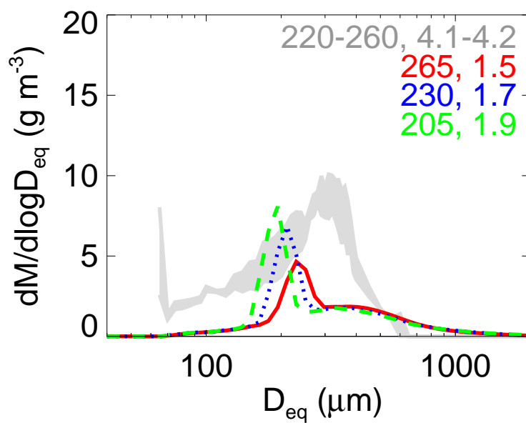
Figure 17. Particle size distributions of fluffy ice at -40\text{ }^{\circ}\text{C} for simulations as in Fig. 16 with baseline updraft and pseudo-Hallett–Mossop sources of 1 (red solid line), 2 (blue dotted line), and 3 \text{std cm}^{-3} (green dashed line).
