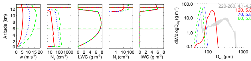
Figure 4. For simulations with droplet activation, diffusional growth, and homogeneous drop freezing only, and baseline updraft strength scaled by factors of 0.5 (red solid line), 1.0 (blue dotted line), and 1.5 (green dashed line), profiles of parcel updraft speed ( w ), water drop concentration ( N_d ), liquid water content (LWC), ice particle concentration ( N_i ), and ice water content (IWC), and ice particle size distribution (PSD) at output level nearest -40\text{ }^\circ\text{C} for simulations with droplet activation, diffusional growth, and homogeneous drop freezing only, and baseline updraft strength scaled by factors of 0.5 (red solid line), 1.0 (blue dotted line), and 1.5 (green dashed line). Shaded area in PSD panel is envelope of median Airbus PSDs from Cayenne and Darwin for \text{IWC} > 4\text{ g m}^{-3} (see Fig. 6 of Part 1). Horizontal lines in profiles correspond to 0 and -40\text{ }^\circ\text{C} . PSD is plotted in terms of ice particle mass ( M ) and area-equivalent diameter D_{\text{eq}} . The numbers in the upper right of the PSD panel are \text{MMD}_{\text{eq}} in units of \mu\text{m} and IWC in units of \text{g m}^{-3} for the IWC-filtered measurements (in gray) and correspond to simulation results with same line color. \text{MMD}_{\text{eq}} from simulations are rounded to nearest 5\text{ }\mu\text{m} to reduce attention to smaller differences attributable to variations in height resulting from 10 s output frequency.
