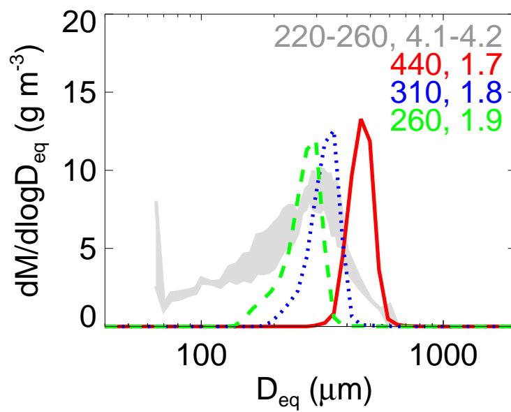
Figure 11. Particle size distributions of fluffy ice at -40^{\circ}\text{C} for simulations as in Fig. 10 with parcel depth \Delta z = 1 \text{ km} and pseudo-Hallett–Mossop sources of 1 (red solid line), 2 (blue dotted line), and 3 \text{ std cm}^{-3} (green dashed line).
