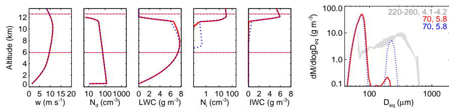
Figure 5. As in Fig. 4 for simulations that also include 1 std cm -3 of immersion-mode IFN (red solid line) or pseudo-Hallett–Mossop embryos (blue dotted line), both with baseline updraft. Details provided in text.
