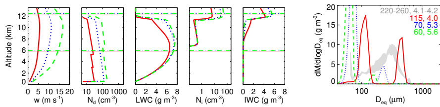
Figure 9. As in Fig. 6 for simulations that also allow sedimentation with parcel depth \Delta z = 1 km.
