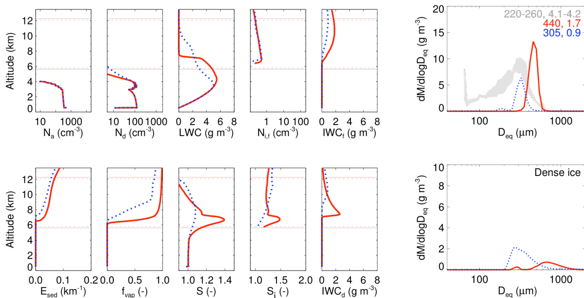
Figure caption: Panels as in fig. 10 for simulations including gravitational collection for parcel depth of 1 km with (red solid line) and without (blue dotted line) raindrop breakup.
