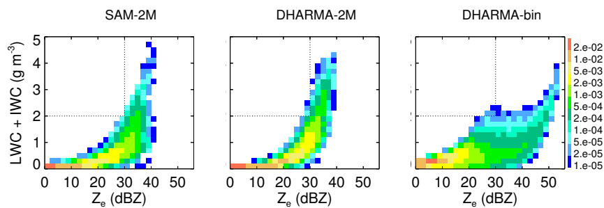
Figure 2. Joint histograms of Rayleigh-regime equivalent radar reflectivity Z_e vs. total hydrometeor condensed water content LWC + IWC from the last twelve hours of 23 January TWP-ICE simulations using the System for Atmospheric Modeling (SAM) with two-moment microphysics (left panel) and the Distributed Hydrodynamic Aerosol and Radiative Modeling for Atmospheres (DHARMA) using two-moment and bin microphysics (center and left-right panels, respectively) at an altitude where the mean air temperature is -40^\circ\text{C} . Simulations with two-moment microphysics are reported by Fridlind et al. (2012) and sampled every three hours, while the DHARMA-bin microphysics simulation uses the same TWP-ICE setup but on a domain with a quarter of the horizontal area and is restarted from a run with two-moment microphysics at 03:00 on 23 January, using microphysics as described by van Diedenhoven et al. (2012).
