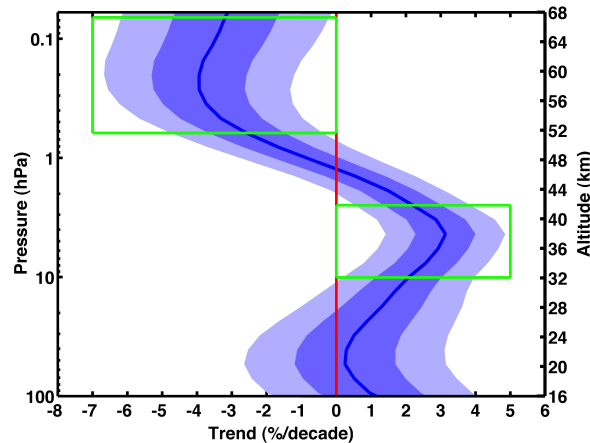
Figure 9. Estimated ozone trend profile (in % decade -1 ) for the period of January 1997 - January 2015 recorded by GROMOS above Bern, Switzerland. The dark blue line represents the trend profile, the darkest blue area and the lightest blue area are the 1 \sigma and 2 \sigma areas, respectively. Being \sigma the uncertainty of the trend estimate. The green boxes are the two regions where the trend is statistically significant at 95% of confidence level.
