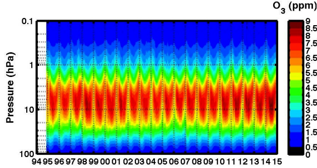
Figure 5. Harmonised 20 years (Nov.1994 - Nov.2014) time series of stratospheric ozone VMR profiles recorded by GROMOS above Bern, Switzerland
