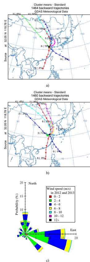
Figure 8. Clusters of 96 h back trajectories arriving at the study site at 100 m in 2012 (a) and 2013 (b) simulated by HYPIT model and the probability distributions of 6 h interval near surface wind speed in different wind directions in Nanjing (c).
