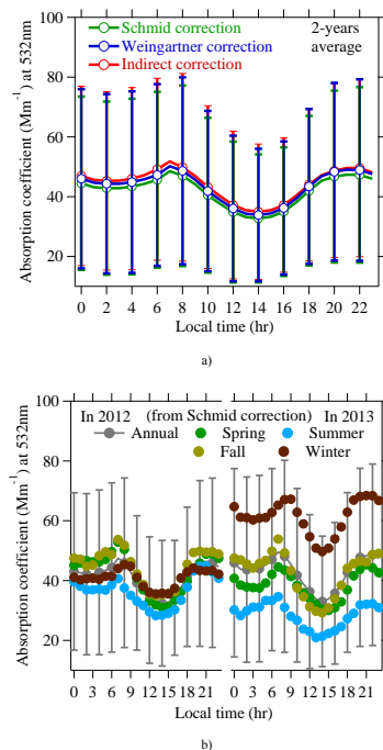
Figure 4. Diurnal variations of the aerosol absorption coefficients at 532 nm in urban Nanjing. (a) The two-year (2012–2013) coefficients corrected by indirect way (red), WC2003 (blue) and SC2006 (light green) and (b) the coefficients corrected by SC2006 in separate seasons of 2012 and 2013. March, April and May represent the spring, June, July and August represent the summer, September, October and November represent the fall, and January, February and December in 2012 (2013) represent the winter in 2012 (2013).
