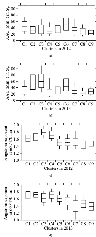
Figure 9. The 10, 25, 50, 75 and 90 % percentile values of the aerosol absorption coefficient ( a, b ) and absorption angstrom exponent ( c, d ) in each cluster of back trajectories in 2012 (Fig. 8a) and 2013 (Fig. 8b).
