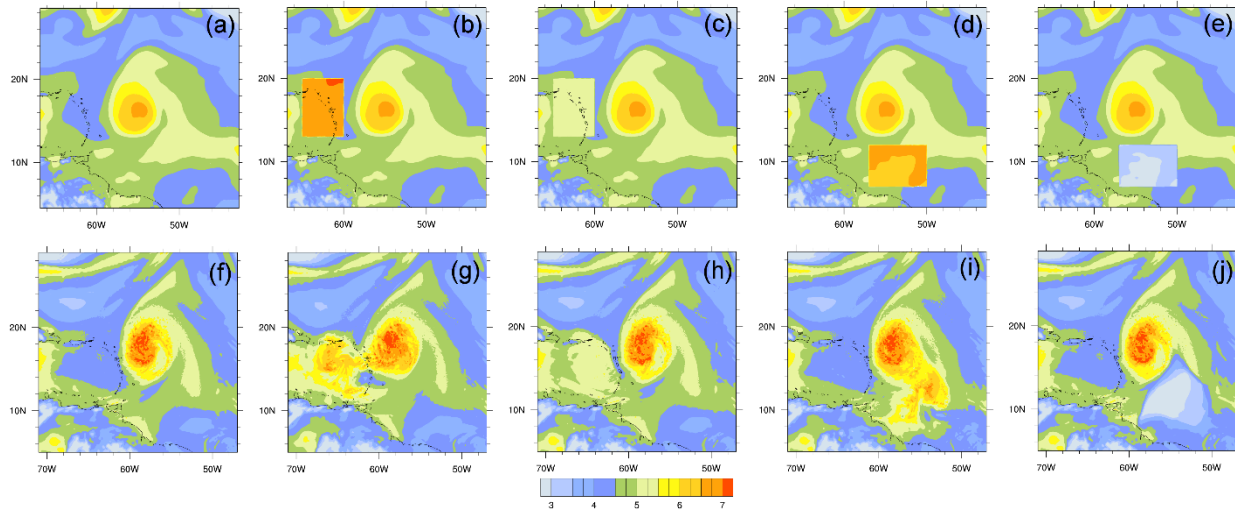
Figure 1. Column-integrated PWV (cm) at the initialization of the WRF simulations: (a) CTRL, (b) MF, (c) MFI, (d) MR, (e) DR; and 12-hour forecast for (f) CTRL, (g) MF, (h) MFI, (i) MR, (j) DR.
