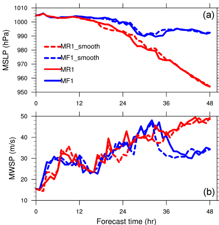
Figure 3 Time series of model simulated (a) MSLP (hPa); (b) MWSP (m/s). MF1 and MR1 are one of the MF and MR ensemble simulations, respectively. MF1_smooth and MR1_smooth are same as MF1 and MR1, respectively, but with smoothed moisture perturbation on the edges.
