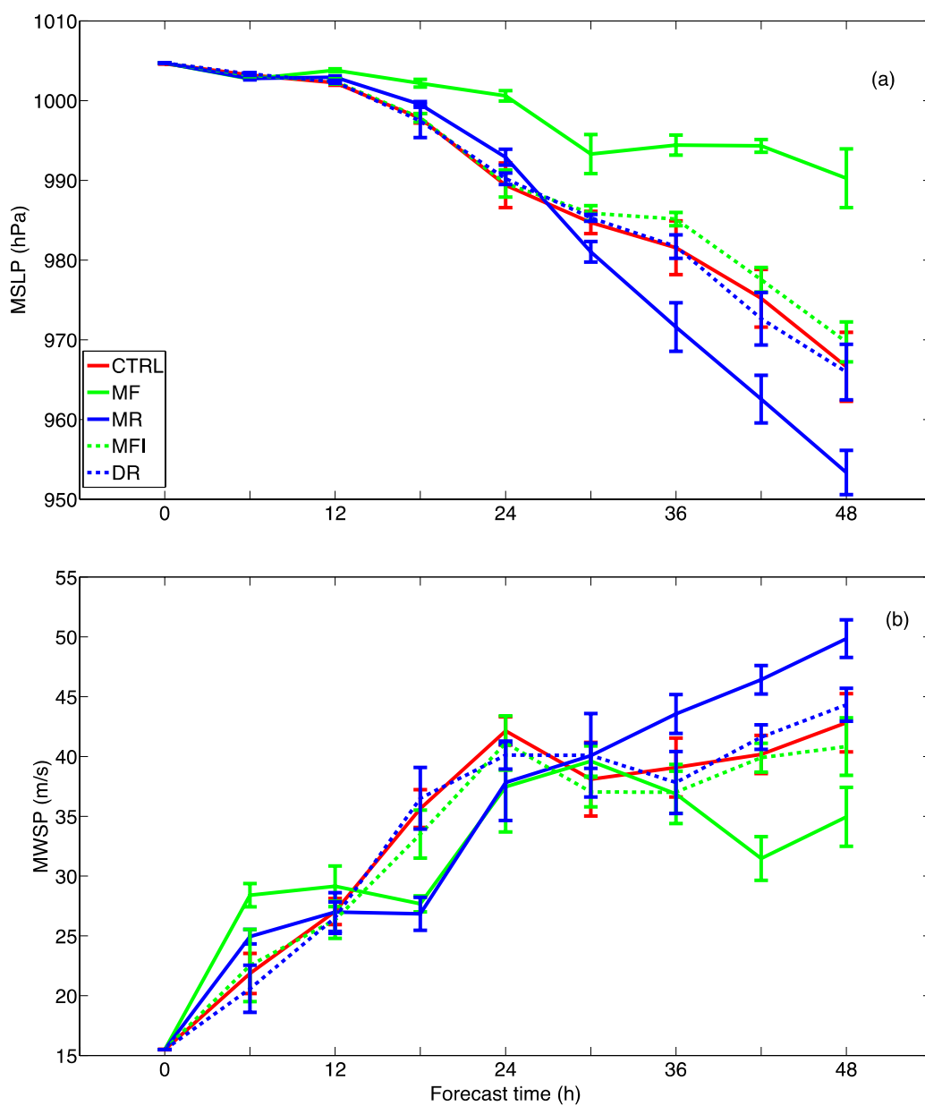
502 503 Figure 2. Time series of the model simulated ensemble mean and standard deviation of (a) MSLP 504 (hPa) and (b) MWSP ( \text{m s}^{-1} ).
