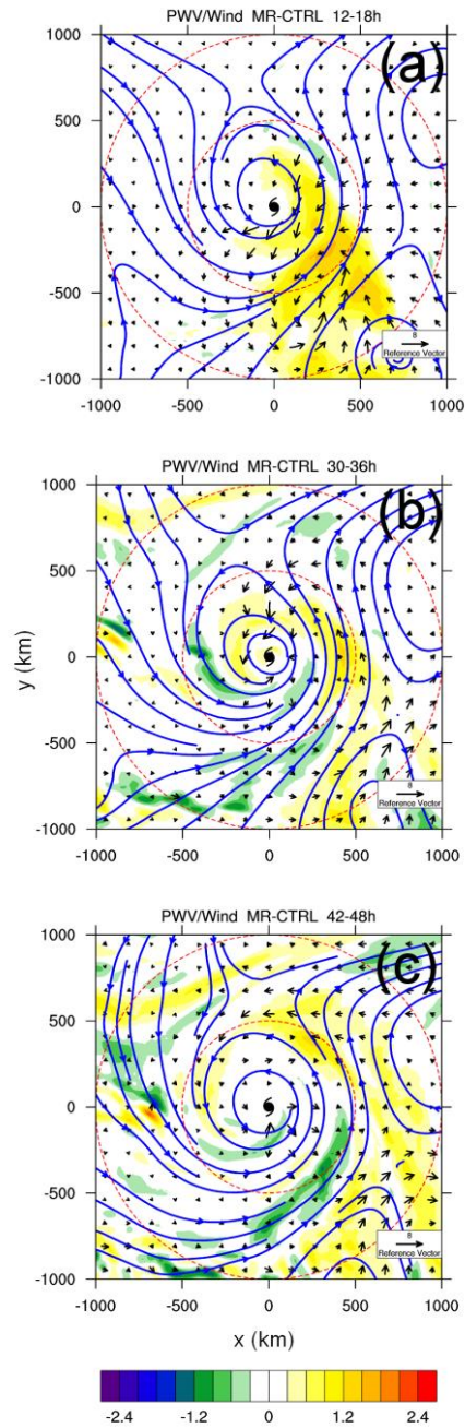
539 Figure 8. Same as Fig. 5, but for differences between the MR and CTRL experiments. Mean 540 wind vectors and column-integrated PWV for CTRL and MR at each time are shown in 541 supplementary Figure 1.
