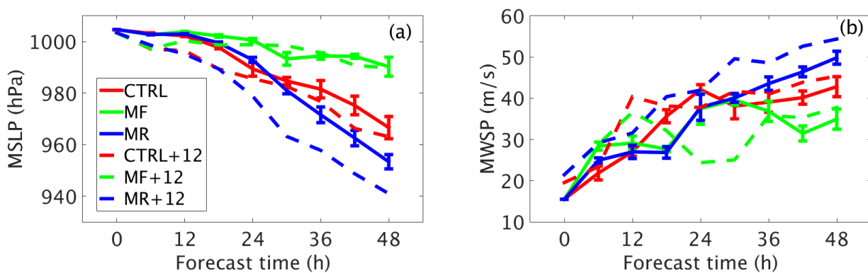
Figure 2 The simulated (a) MSLP (hPa) and (b) MWSP (m/s) for CTRL (solid red), MF (solid green), MR (solid blue), CTRL+12hr (dashed red), MF+12hr (dashed green) and MR+12hr (dashed blue).
