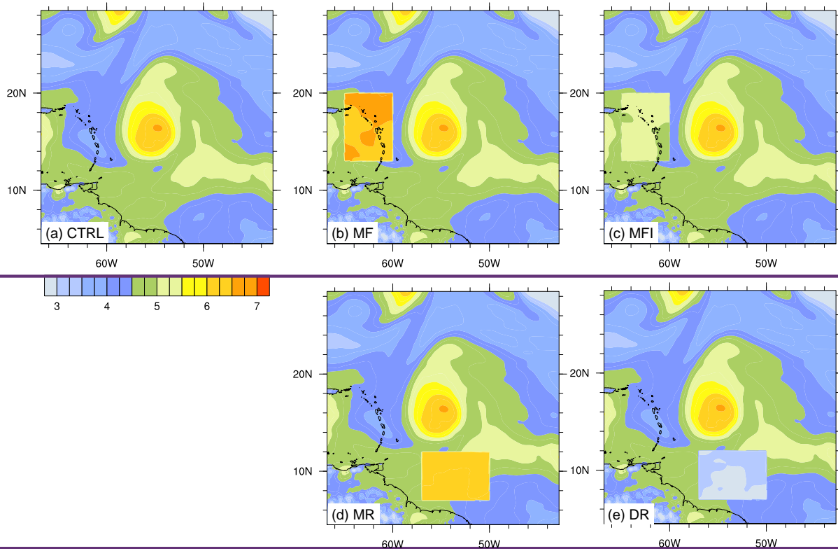
499 Figure 1. Column-integrated PWV (cm) at the initialization of the WRF simulations: (a) CTRL; 500 (b) MF; (c) MFI; (d) MR; (e) DR; and 12-hour forecast for (f) CTRL, (g) MF, (h) MFI, (i) MR, 501 (j) DR.
