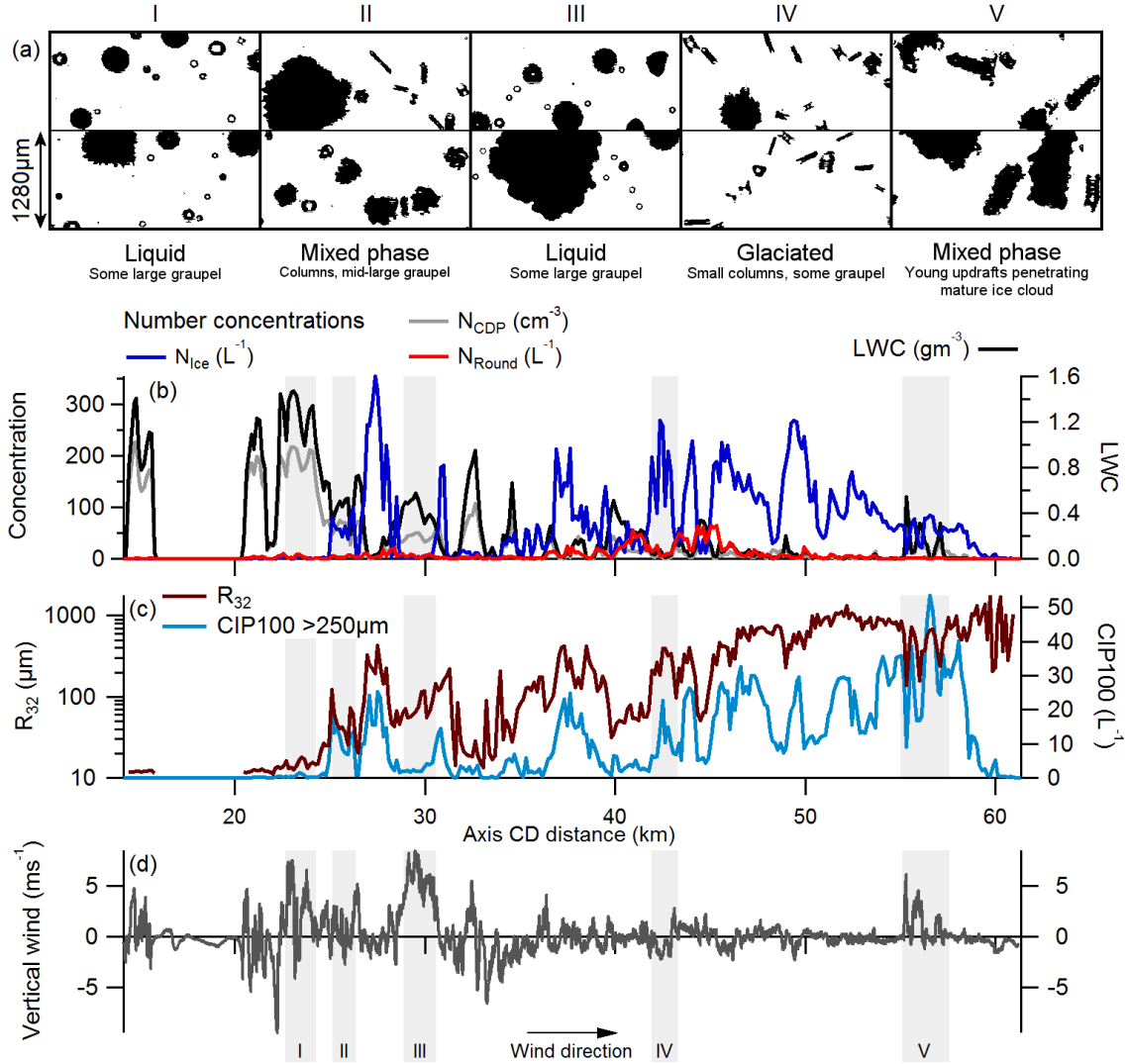
Figure 5. In situ measurements made by the BAe-146 on longitudinal Run 11.2 along axis CD. The run was made at an altitude of 3.5 km ( T \sim -5^{\circ}\text{C} ) between 13:34:55 and 13:40:30 UTC. In panel (b), the number concentrations use the left axis, and the units are defined according to the measurement probe. The 2DS categories are defined in Appendix A. The images shown were recorded by the 2DS and show representative images from the sections marked by grey boxes and labelled with Roman numerals. Only images >50 pixels are shown, and they are not classified by shape.
