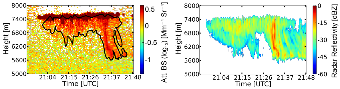
Fig. 4. Lidar and radar observations on 2 August 2012 (case 2). Left: 532 nm attenuated backscatter coefficient, right: radar reflectivity.
