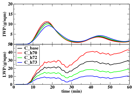
Fig. 14. Liquid (lower panel) and ice water paths (upper panel) for case 2. Comparison of the different values for h_{bot} .
