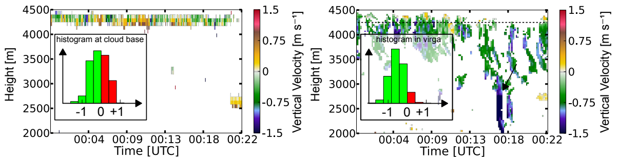
Fig. 3. Vertical velocity for case 1. Left: derived from lidar (valid for more numerous smaller droplets at cloud base), right: derived from radar observations (valid for large particles; virgae).
