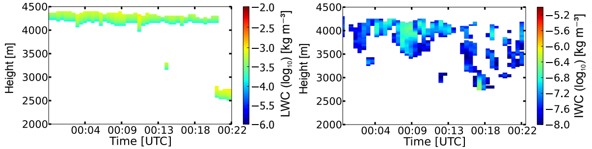
Fig. 2. Cloudnet derived water contents for case 1. Left: Liquid water content, right: ice water content (both in logarithmic scale).
