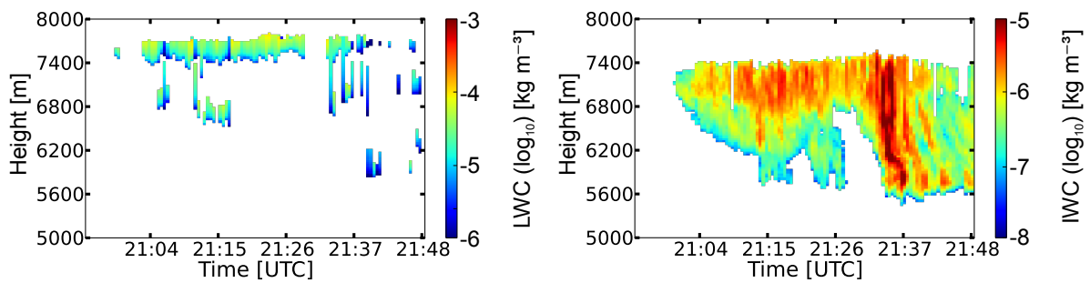
Fig. 5. Cloudnet derived water contents for case 2. Left: Liquid water content, right: ice water content (both in logarithmic scale).
