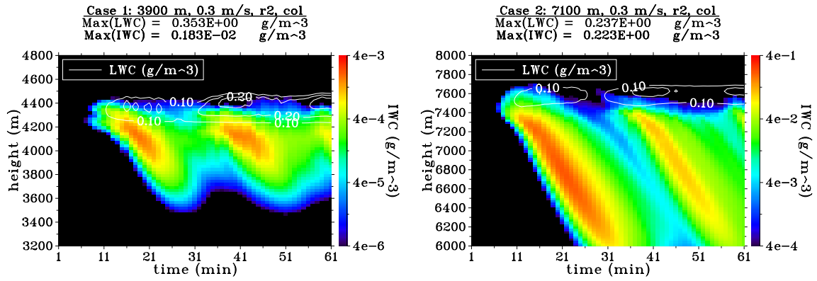
Fig. 20. LWC (contours) and IWC (colors, logarithmic scale). Results for changing ice particle shape to hexagonal columns for case 1 (W.col, left) and case 2 (C.col, right).
