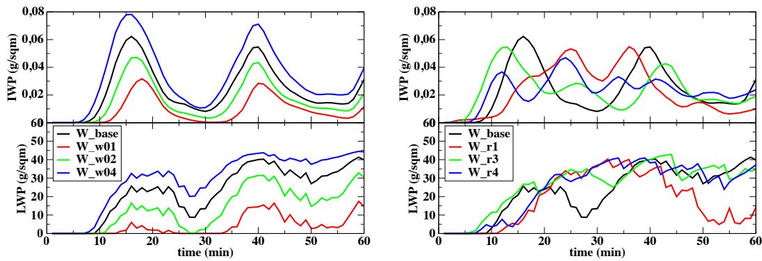
Fig. 12. Liquid (lower panels) and ice water paths (upper panels) for case 1. Comparison of the different values for w_{ave} (left) and the different stochastic realizations (right).
