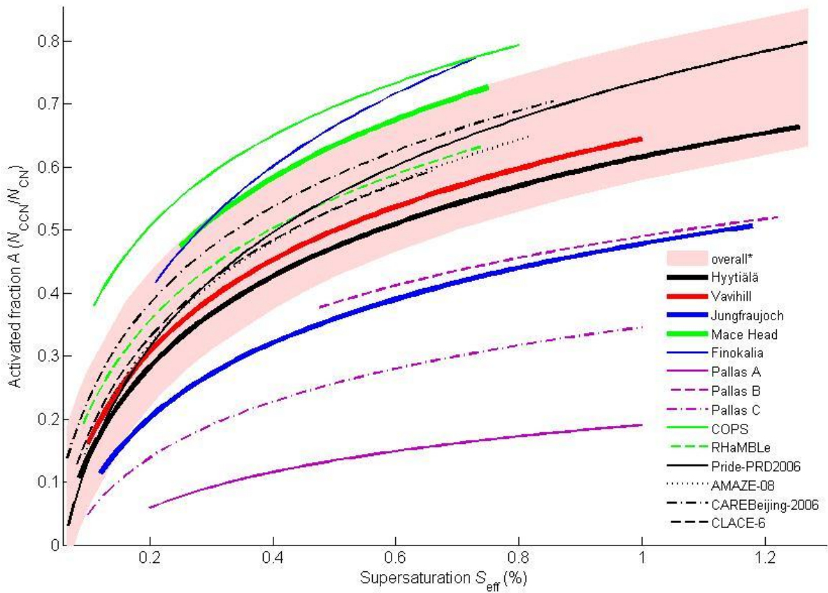
2 Figure 4. Average activated fraction A as a function of supersaturation S_{\text{eff}} for all available 3 datasets. Shown are the linear fits in the form A = a \times \ln(S_{\text{eff}}) + b . Also shown is the overall fit 4 based on most of the data points (*Finokalia, COPS, Jungfraujoch and Pallas A, B and C 5 datasets excluded). The shading of the overall fit represents the prediction bounds of the fit with 6 a confidence level of 95%.
