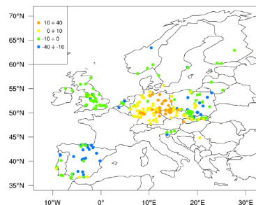
Figure 16. Spring (MAM) 24 h average PM 10 concentrations in \mu\text{g m}^{-3} (a), MBE at rural stations (b), MBE at suburban stations (c) MBE at urban stations (d).
