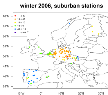
Figure 15. Winter (DJF) 24 h average PM_{10} concentrations in \mu g m^{-3} (a), MBE at rural stations (b), MBE at suburban stations (c) MBE at urban stations (d).
