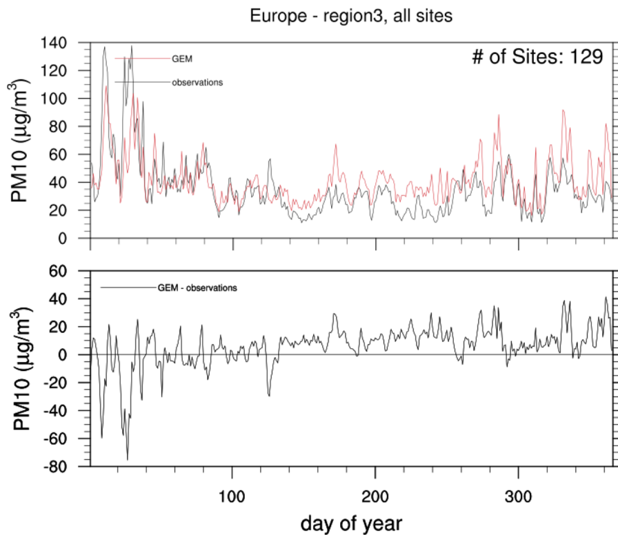
Figure 21. Time series of observed and modelled \text{PM}_{10} 24 h concentration (a) averaged for all stations in Central Europe, (b) MBE.
