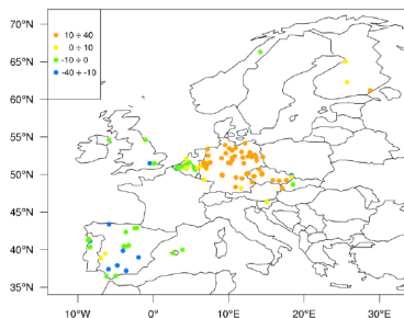
Figure 18. Autumn (SON) 24 h average PM_{10} concentrations in \mu g m^{-3} (a), MBE at rural stations (b), MBE at suburban stations (c) MBE at urban stations (d).
