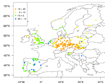
Figure 17. Summer (JJA) 24 h average PM 10 concentrations in \mu\text{g m}^{-3} (a), MBE at rural stations (b), MBE at suburban stations (c) MBE at urban stations (d).
