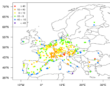
Figure 4. Spring (MAM) maximum 8 h running average ozone concentration in \mu\text{g m}^{-3} (a), MBE at rural stations (b), MBE at suburban stations (c) MBE at urban stations (d).
