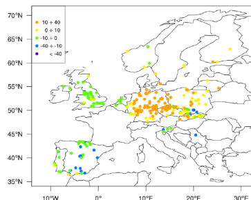
Figure 18. Autumn (SON) 24 h average PM_{10} concentrations in \mu g m^{-3} (a), MBE at rural stations (b), MBE at suburban stations (c) MBE at urban stations (d).
