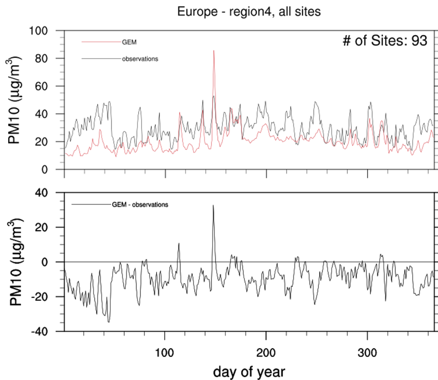
Figure 22. Time series of observed and modelled \text{PM}_{10} 24 h concentration (a) averaged for all stations in Southern Europe, (b) MBE.
