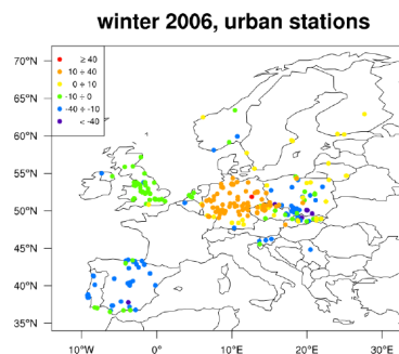
Figure 15. Winter (DJF) 24 h average PM_{10} concentrations in \mu g m^{-3} (a), MBE at rural stations (b), MBE at suburban stations (c) MBE at urban stations (d).
