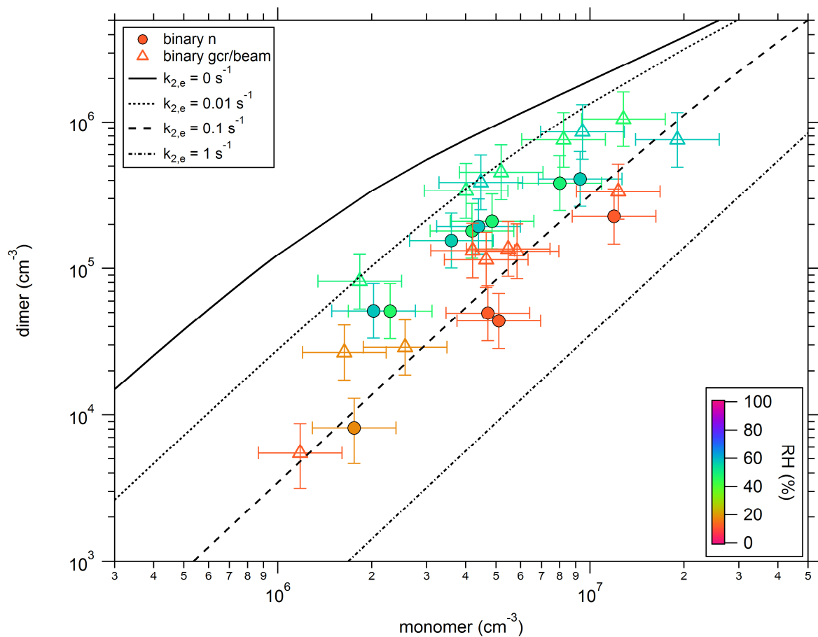
Fig. 4. Sulfuric acid dimer concentration of as a function of the monomer concentration at 208 K for binary conditions. The full circles are from neutral experiments obtained at steady-state and the open triangles from ion-induced experiments. The black lines indicate the modeled dimer concentration for a given dimer evaporation rate with all other cluster evaporation rates set to zero. The color code indicates the relative humidity over supercooled water.
