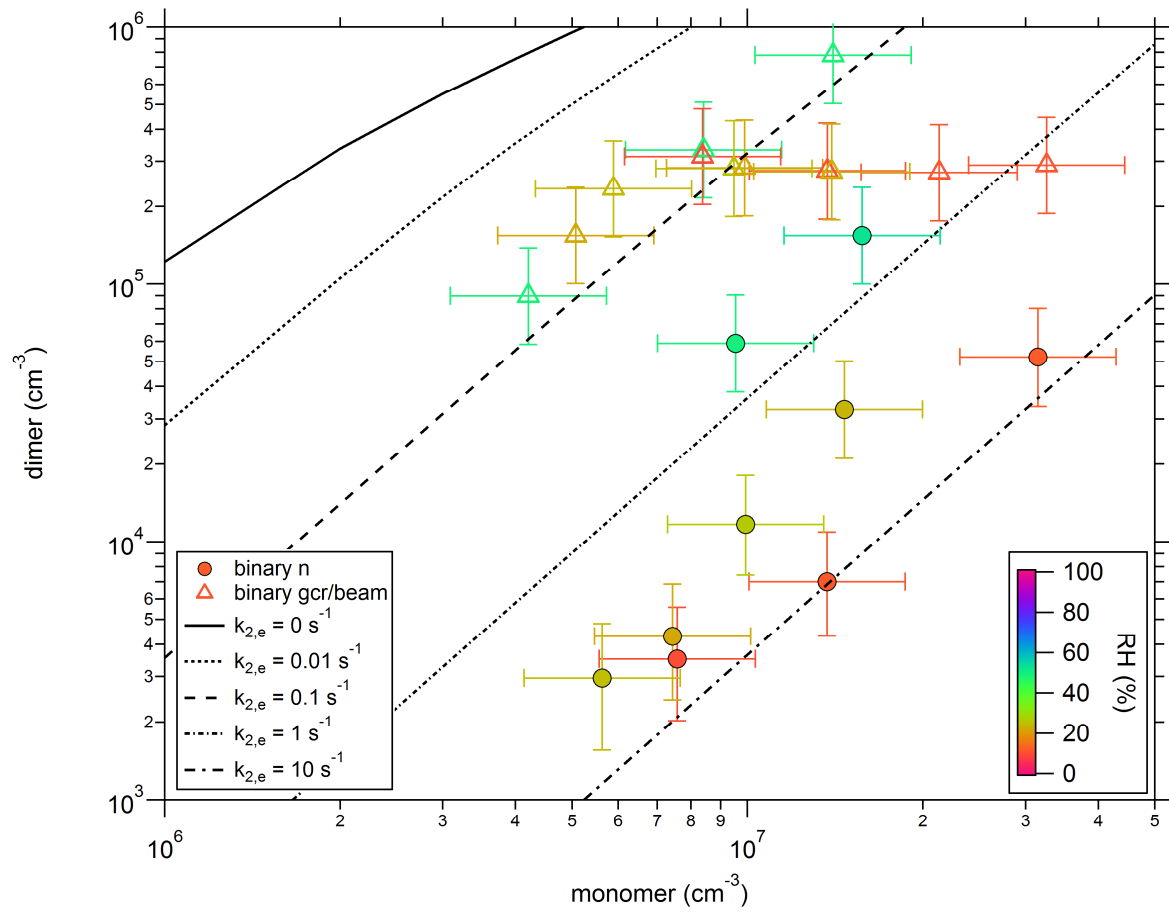
Fig. 5. Same as Fig. 4 but for a temperature of 223 K.
