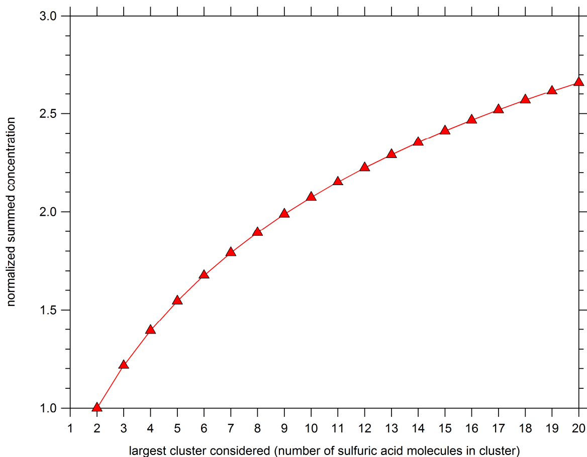
Fig. 3. Simulated summed cluster concentrations at 223 K and 20% RH ( k_{2,e} = 5.8 \text{ s}^{-1} and k_{3,e} = 0.056 \text{ s}^{-1} ; all larger evaporation rates are zero). The cluster concentrations are summed up to a certain number of sulfuric acid molecules in a cluster starting with the dimer concentration. The values on the x -axis indicate the number of sulfuric acid molecules in the largest cluster considered in the summation. All concentrations are normalized by the dimer concentration (at 2.0 \times 10^7 \text{ cm}^{-3} monomer concentration).
