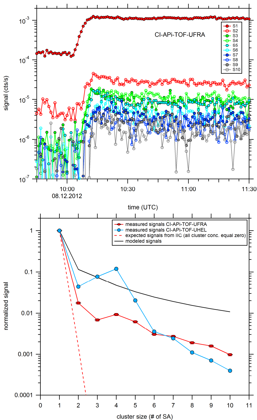
Fig. 8. Cluster measurements for the binary system at 206 K and a RH close to 100% over ice measured with two CI-API-TOFs (UFRA and UHEL instruments). The upper panel shows the monomer (S1) and the cluster signals ( S_i , i \geq 2 ) normalized by the nitrate ion signals as a function of time (1 minute time resolution) for the CI-API-TOF-UFRA. The lower panel shows the measured steady-state signals as well as expected signals using different assumptions as function of the cluster size. See text for details.
