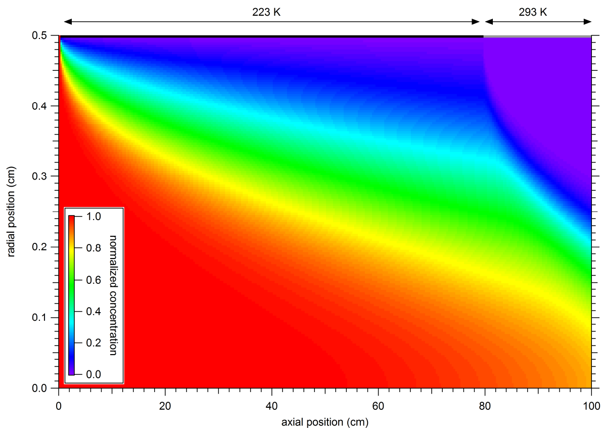
5 Fig. 1. Simulated transmission of dimers through the CIMS sampling line at a temperature of 223 K for the incoming air. The temperature of the sampling line is fixed to 223 K for the first 80 cm (black color at top axis) and to 293 K for the last 20 cm (grey color at top axis). Wall loss is the dominant loss process over the first 80 cm, whereas evaporation is an additional loss process for the last 20 cm. The overall transmission (diffusion loss and evaporation) is 22.8% at a flow rate of 7.6 \text{ liter min}^{-1} , while it is 47.5% 10 when evaporation is neglected (diffusion loss only). See text for details.
