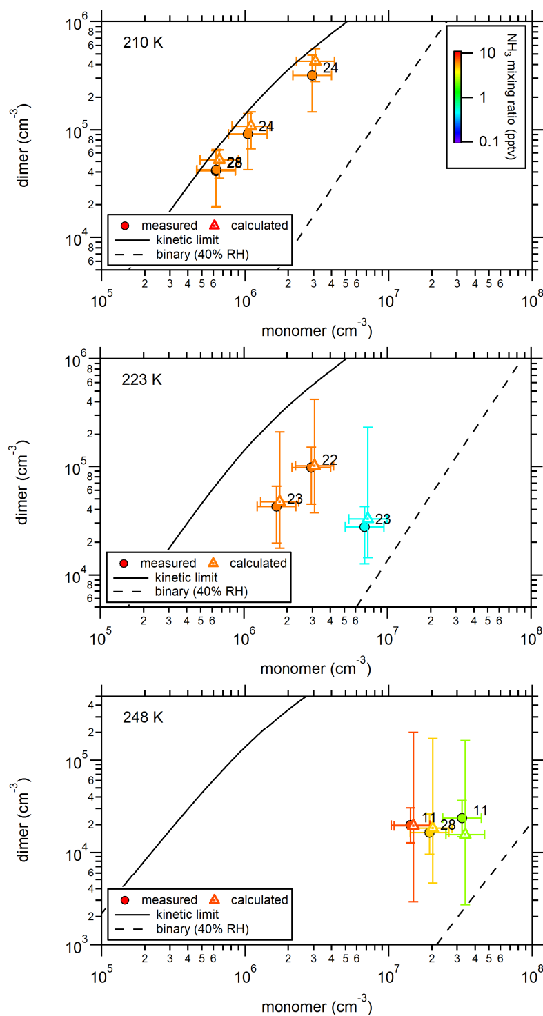
Fig. 9. Sulfuric acid dimer concentrations as a function of the sulfuric acid monomer concentration at three different temperatures for the ternary system involving ammonia (ammonia mixing ratio indicated by the color code). The colored circles are the measured concentrations. Lines are from model calculations indicating the expected concentrations for the binary system (dashed line) and the kinetic limit (solid line). The numbers indicate the RH (in %) during an experiment. Open colored triangles are the simulated dimer concentrations using the reaction scheme from Fig. 10. These are slightly offset to the right in order to improve readability.
