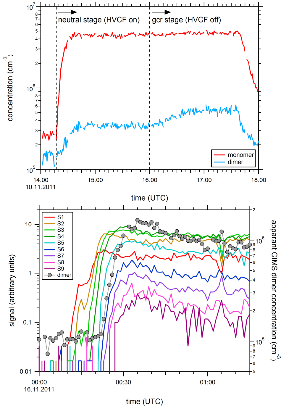
Fig. 2. Upper panel: observed ion effect on CIMS sulfuric acid dimer ( m/z 195) measurements at 223 K. The first part of the experiment is under neutral conditions, the second part is a GCR run with ions present in the chamber. The increase in the dimer signal during the GCR stage is due to ions detected by the CIMS and not due to neutral dimers. Lower panel: comparison between the APi-TOF signals and the CIMS dimer measurements for a different ion-induced experiment at 223 K. The ion clusters (S6, i.e., \text{HSO}_4^-(\text{H}_2\text{SO}_4)_5 and larger) show a clear correlation with the apparent dimer signal, which indicates that fragmented cluster ions contribute to the CIMS dimer measurement (Pearson's correlation coefficient between dimer and S6 is 0.93).
