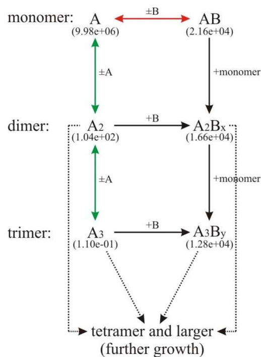
Fig. 10. Reaction scheme for the sulfuric acid dimer formation in the ternary system at a low temperature. ‘A’ denotes a sulfuric acid molecule, and ‘B’ an ammonia molecule. ‘Monomer’ is the sum of the concentration of the pure sulfuric acid (A) and the sulfuric acid bound to an ammonia (AB). ‘Dimer’ is the sum of all clusters containing two sulfuric acid molecules ( A_2 + A_2B + A_2B_2 ) and the same applies for the ‘trimer’ with three sulfuric acid molecules. The arrows indicate the relevant reactions and whether only collisional growth (single-ended arrow) or growth as well as evaporation (double-ended arrow) are important. Losses due to walls, dilution and coagulation are included in the model but not indicated. Small numbers represent concentrations for an example calculation at a temperature of 248 K, a [monomer] of 1 \times 10^7 \text{ cm}^{-3} and a [\text{NH}_3] of 2 \times 10^8 \text{ cm}^{-3} . See text for details.
