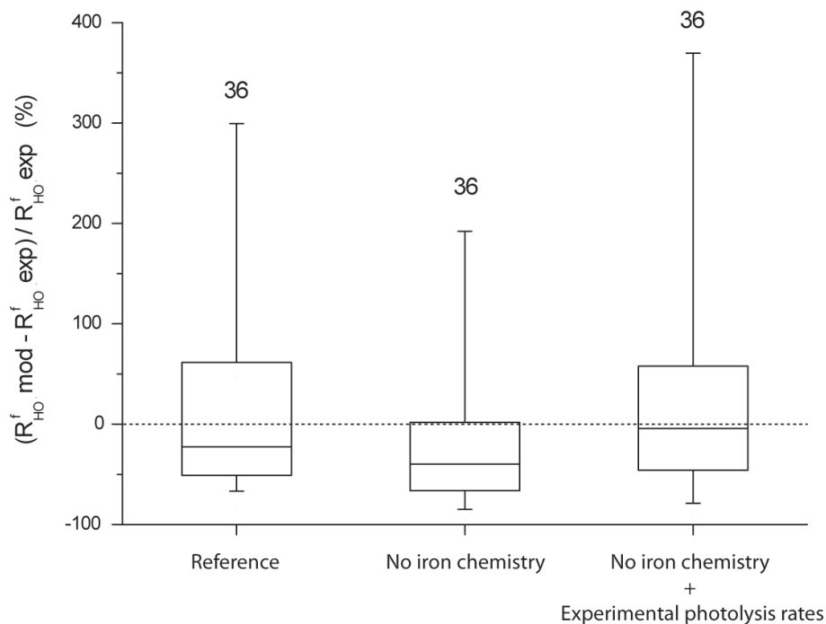
Figure 5. Distribution of the bias error for the whole cloud water samples for the reference case and for two sensitivity tests performed with the model: (i) the iron chemistry (photolysis of Fe(III) and the Fenton reaction) is neglected in the model; (ii) the iron chemistry is neglected, and the new photolysis rate constants obtained from experimental measurements are implemented in the model. The bias error is defined by the ratio (R_{HO}^f \text{ mod} - R_{HO}^f \text{ exp}) / R_{HO}^f \text{ exp} in (%). The number of samples analyzed is indicated above each box plot. The bottom and top lines correspond to the 25 and 75 %, respectively. The full line represents the median values. The ends of the whiskers are the 10 and 90 %.
