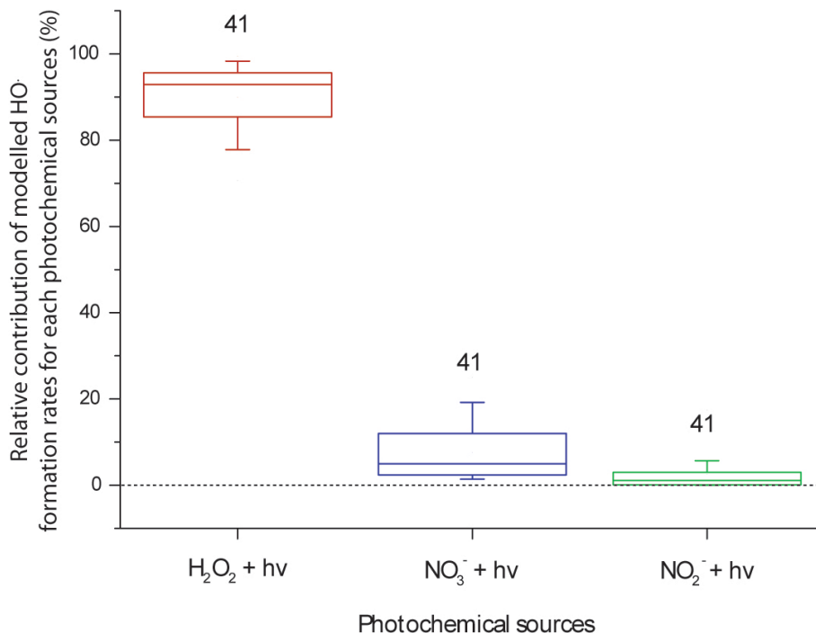
Figure 6. Distribution of relative contributions of modeled \text{HO}^\bullet formations rates for each photochemical source ( \text{H}_2\text{O}_2 , \text{NO}_3^- and \text{NO}_2^- photolysis) for the whole cloud water samples. Model outputs are obtained from the sensitivity test in which the iron chemistry is not considered, and new photolysis rate constants from experimental measurements are implemented in the model. The number of samples analyzed is indicated above each box plot. The bottom and top lines correspond to the 25 and 75 %, respectively. The full line represents the median values. The ends of the whiskers are the 10 and 90 %.
