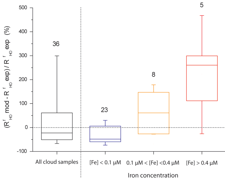
Figure 4. Distribution of the bias error for the whole cloud water samples (black) and for cloud samples discretized as a function of different iron concentration ranges (in color). The bias error is defined by the ratio (R_{\text{HO}}^f \text{ mod} - R_{\text{HO}}^f \text{ exp}) / R_{\text{HO}}^f \text{ exp} in (%). The number of samples analyzed is indicated above each box plot. The bottom and top lines correspond to the 25 and 75%, respectively. The full line represents the median values. The ends of the whiskers are the 10 and 90%.
