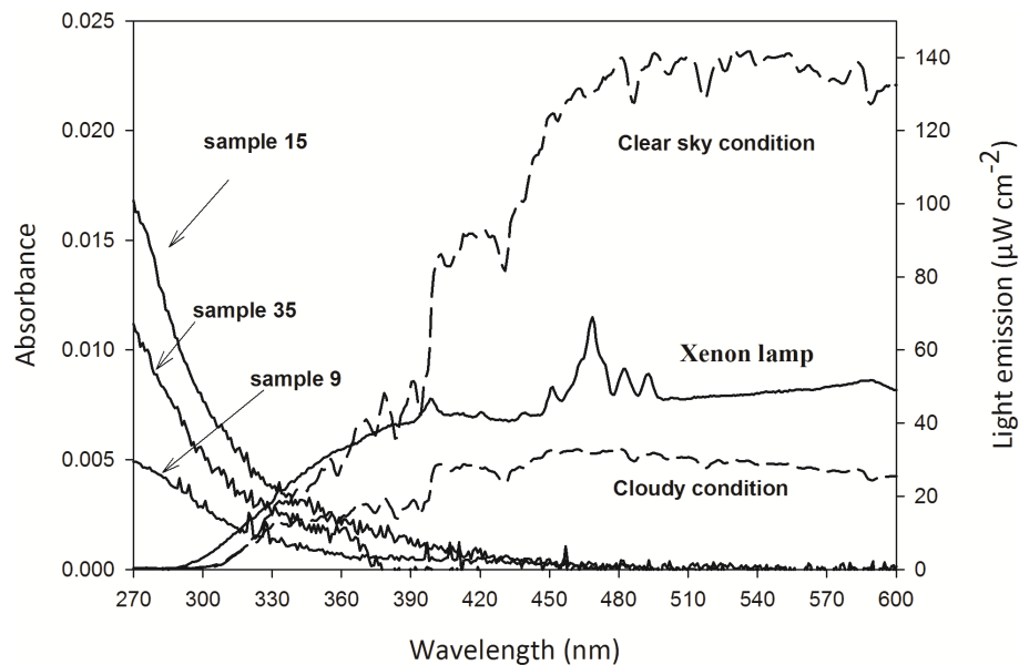
Figure 1. Absorption spectra of different cloud water samples (left axis) and the right-hand axis shows the emission spectrum of the adopted Xenon lamp reaching solutions over the range of 290 to 600 nm (total flux intensity = 157 \text{ W m}^{-2} ) compared with the sun emission spectrum (dashed line) for a sunny ( 353 \text{ W m}^{-2} ) and a cloudy day ( 90 \text{ W m}^{-2} ) in October 2013.
