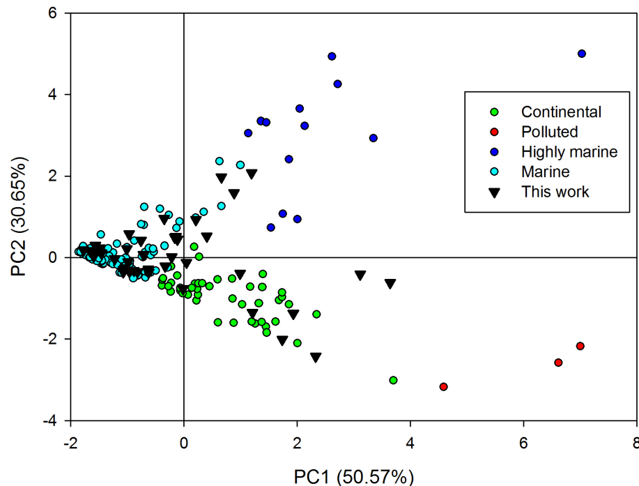
Figure 2. Scores plot obtained by PCA analysis of 137 samples collected before 2013 and grouped in four classes as a function of the previously described classification (Deguillaume et al., 2014) and 41 samples collected during 2013 and 2014. These new data correspond to 15 cloud events and are indicated in black triangles. Statistical analysis is performed using 6 selected variables (pH, [\text{Na}^+] , [\text{Cl}^-] , [\text{SO}_4^{2-}] , [\text{NO}_3^-] , and [\text{NH}_4^+] ). The scree plot obtained from autoscaled data shows that two selected principal components (PC) containing a total variance of about 81 %.
