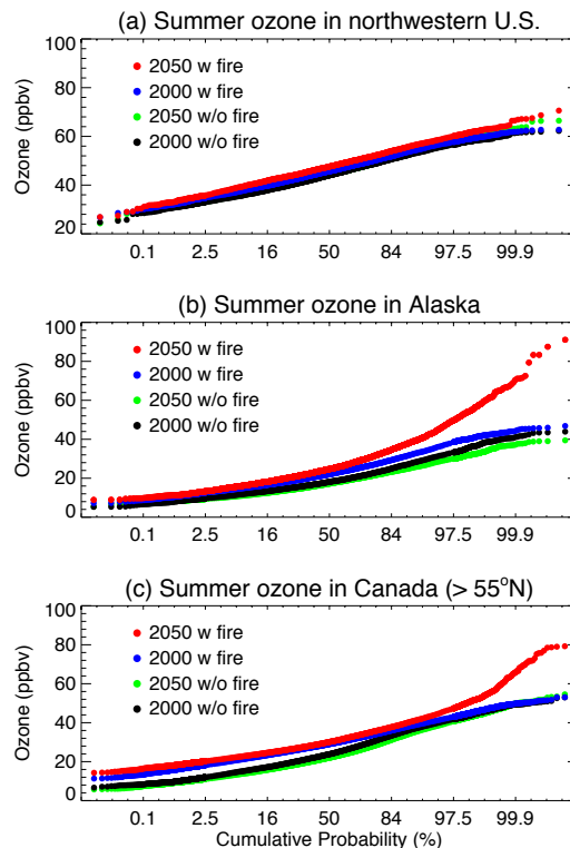
Figure 11. Simulated cumulative probability distributions of MDA8 ozone at the surface in summer (June–August) over (a) northwestern US (> 40° N), (b) Alaska, and (c) Canada (> 55° N) for different scenarios. Black shows the present-day (1997–2001) climate without wildfire emissions; green shows future (2047–2051) climate without wildfire emissions; blue indicates present-day climate including the associated wildfire emissions; and red indicates future climate including the associated wildfire emissions. Each point represents the value in one grid square within each region for each day during the five model summers (1997–2001 or 2047–2051).
