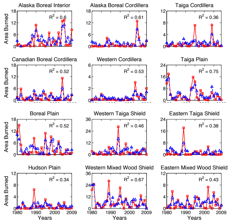
Figure 4. Observed (red solid lines) and predicted (blue dashed lines) area burned ( 10^5 ha) for 1980–2009 in boreal ecoregions. The area burned is calculated using the regressions for the fire season (May–October) for each ecoregion. Site-based observations from GSOD are used in the prediction. The fraction of the variance in observed area burned explained by the regression ( R^2 ) is shown on each panel.
