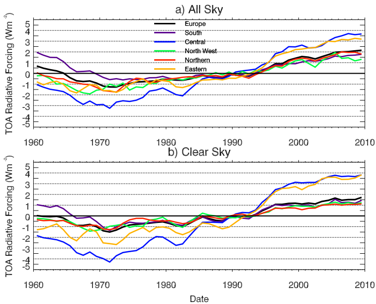
Figure 16. European and sub-regional top of atmosphere aerosol radiative forcing ( \text{Wm}^{-2} ), relative to a 1980 to 2000 average, under a) all-sky and b) clear-sky conditions. European regions are as defined in Fig. 1
