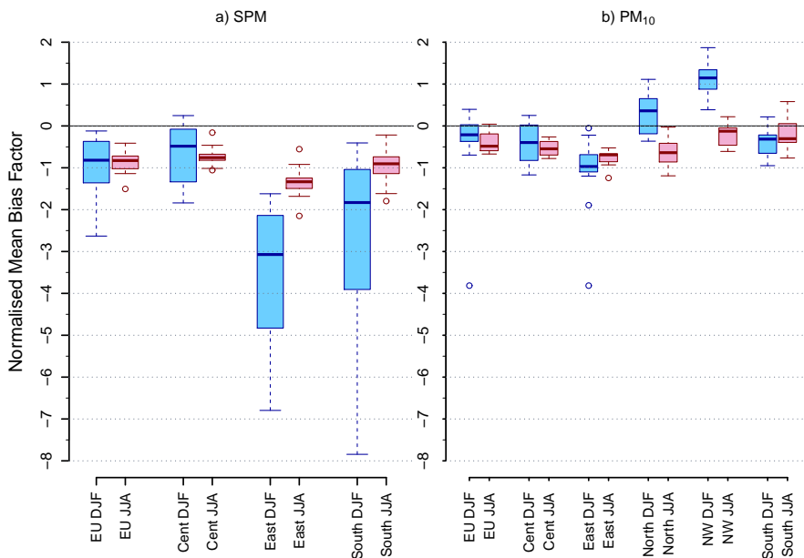
Figure 9. European and sub-regional Normalised Mean Bias Factors for summertime (red) and wintertime (blue) a) suspended particulate matter (SPM) and b) PM 10 mass concentrations across all the years that data was available. The solid line shows the median value, the boxes show the 25 th and 75 th percentile values with the error bars showing the maximum and minimum values and the circles representing outliers (values > 1.5 * inter quartile range).
