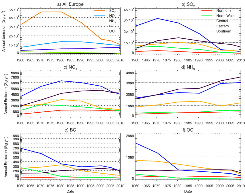
Figure 2. Annual European emissions (Gg yr -1 ) of aerosols and aerosol precursors from the MACC inventory over the period 1960-2009. a) Total European emissions of sulfur dioxide (SO 2 , orange), organic carbon (OC, light green), black carbon (BC, black), ammonia (NH 3 , light purple) and oxides of nitrogen (NO x , blue). b) to f) shows European regional emissions for b) SO 2 , c) NO x , d) NH 3 , e) BC and f) OC. Regions are as defined in Fig. 1: northern (red), north west (green), central (blue), eastern (orange), southern (purple).
