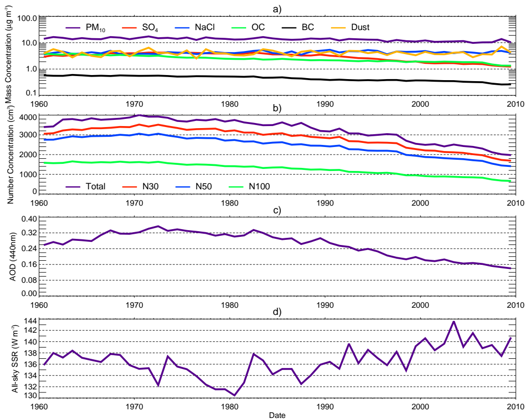
Figure 4. Simulated European annual mean a) \text{PM}_{10} and composition resolved surface mass concentration, b) aerosol number concentration for particles with dry diameter >3 nm (total), >30 nm (N30), >50 nm (N50) and >100 nm (N100), c) aerosol optical depth (AOD) at 440 nm and d) surface solar radiation (SSR) between 1960 and 2009. Mean values are calculated over the European land domain shown in Fig. 1
