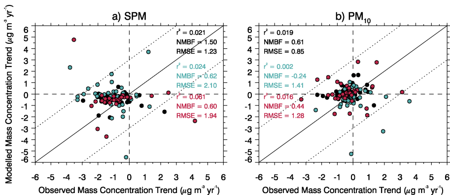
Figure 10. Annual (black), summertime (red) and wintertime (blue) calculated linear trends in modelled and observed a) suspended particulate matter (SPM) and b) \text{PM}_{10} mass concentrations ( \mu\text{g S m}^{-3} \text{yr}^{-1} ) at each individual monitoring location over their operational period between 1978 to 2002 for SPM and 1996 to 2009 for \text{PM}_{10} .
