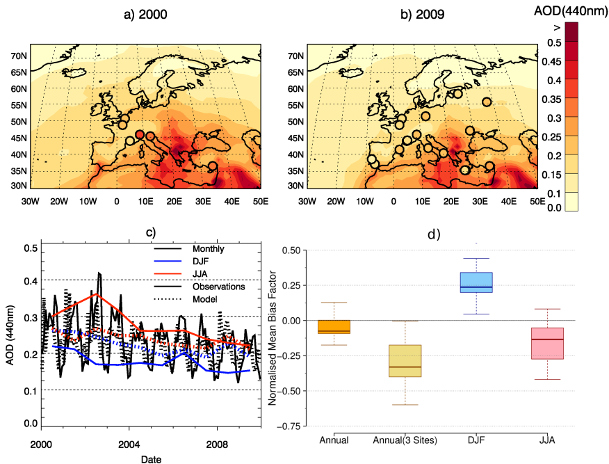
Figure 12. Annual mean aerosol optical depth (AOD) at 440 nm with observations from the AERONET sites overplotted for a) 2000 and b) 2009. c) Time series of monthly and seasonal mean observed (solid lines) and modelled (dashed lines) AOD at 440 nm averaged across all measurement locations. d) European Normalised Mean Bias Factors (NMBF) of AOD for annual (orange), summertime (red) and wintertime (blue) across all the years and sites that data was available. The annual NMBF for the 3 sites with the longest continuous record (> 9 years) is shown in yellow.
