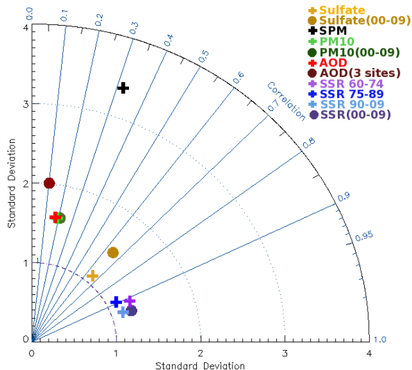
Figure 15. Taylor diagram comparing simulated and observed European sulfate mass concentrations, suspended particulate matter (SPM), PM_{10} , aerosol optical depth (AOD) and surface solar radiation (SSR). Comparisons are made across all the years observations are available. We additionally show results for the period 2000-2009, where sulfate, PM_{10} , AOD and SSR are consistently available. For AOD, we separately plot the 3 locations with the longest observational record. For SSR we also across three different time periods (1960-1974, 1975-1989, 1990-2009). Correlation coefficients are plotted against the observed standard deviations normalised relative to the simulated standard deviation.
