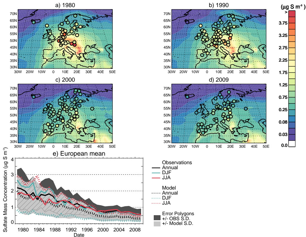
Figure 5. Annual mean sulfate aerosol mass concentrations ( \mu\text{g S m}^{-3} ) from the lowest model level with observations overplotted in circles for a) 1980, b) 1990, c) 2000 and d) 2009. e) Time series of annual and seasonal mean observed (solid lines) and modelled (dashed lines) sulfate concentrations averaged across all measurement locations for each particular year. Shaded areas show \pm 1 standard deviation of the modelled (light grey) and observed (dark grey) annual mean values, with the hatching identifying areas of overlap.
