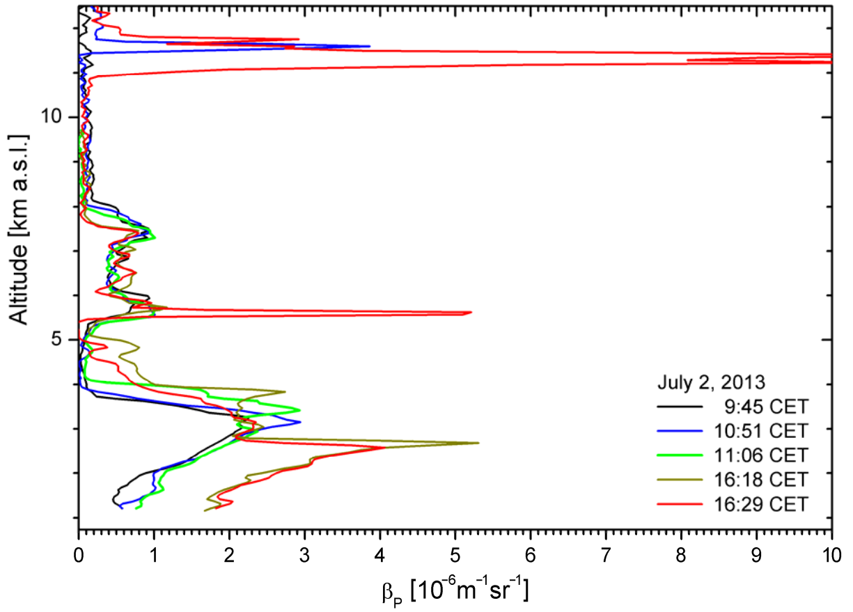
Fig. 5. 313-nm particle backscatter coefficients for July 2, 2013; the spikes between 11 and 12 km are due to faint cirrus clouds.
