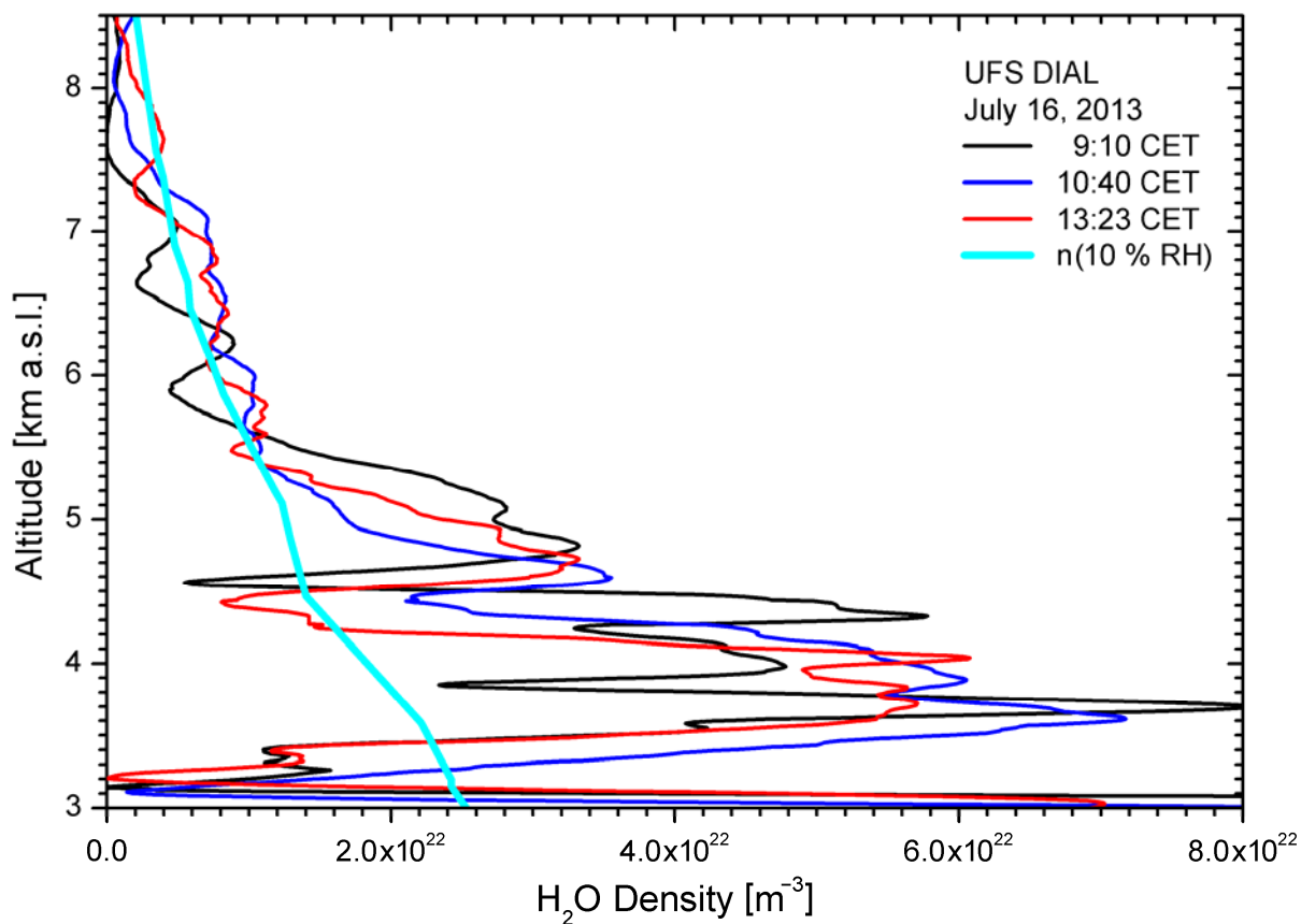
Fig. 17. Water-vapour profiles obtained with the UFS DIAL on July 16, 2013 together with the 10 % RH curve from the Stuttgart radiosonde (Munich data not being available); the layer with most aerosol is extremely dry suggesting the presence of stratospheric air. Also in the aerosol layer around 4.5 km relative humidity values of the order of just 5 % are seen indicating a strong stratospheric component.
