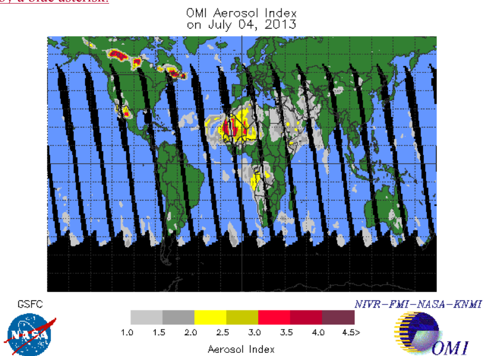
Fig. 2. OMI aerosol index for July 4, 2013
