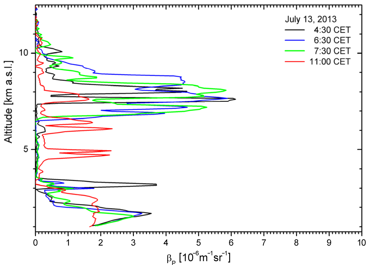
Fig. 10. 313-nm particle backscatter coefficients for July 13, 2013; on this day almost the entire troposphere was filled with aerosol layers from the Canadian fires.
