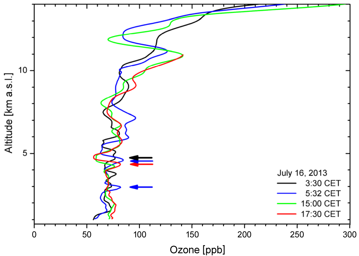
Fig. 16. Ozone profiles for July 16, 2013, in the layers of strongly enhanced aerosol below 5 km the ozone mixing ratio is several times slightly elevated (see arrows, colour chosen as in corresponding curves). Elevated ozone is seen also in other layers.
