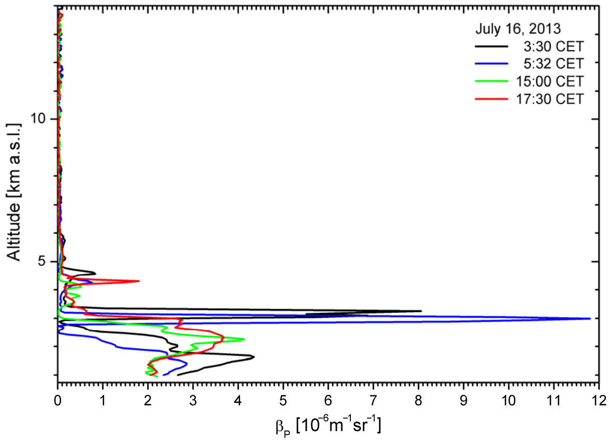
Fig. 15. 313-nm particle backscatter coefficients for July 16, 2013; the peak backscatter coefficient at 5:32 CET, 1.2 \times 10^{-5} , corresponds to a horizontal standard visual range of the order of 6.5 km.
