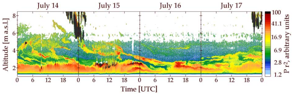
Fig. 14: Range-corrected backscatter signal ( P(r) r^2 ; logarithmic colour code), measured by ceilometer over Hohenpeißenberg (South Germany) from July 14 to 17, 2013. Areas with low signal/noise ratio are masked white. The smoke layer descends across the Zugspitze summit on July 16 and even seems to penetrate into the boundary layer.
