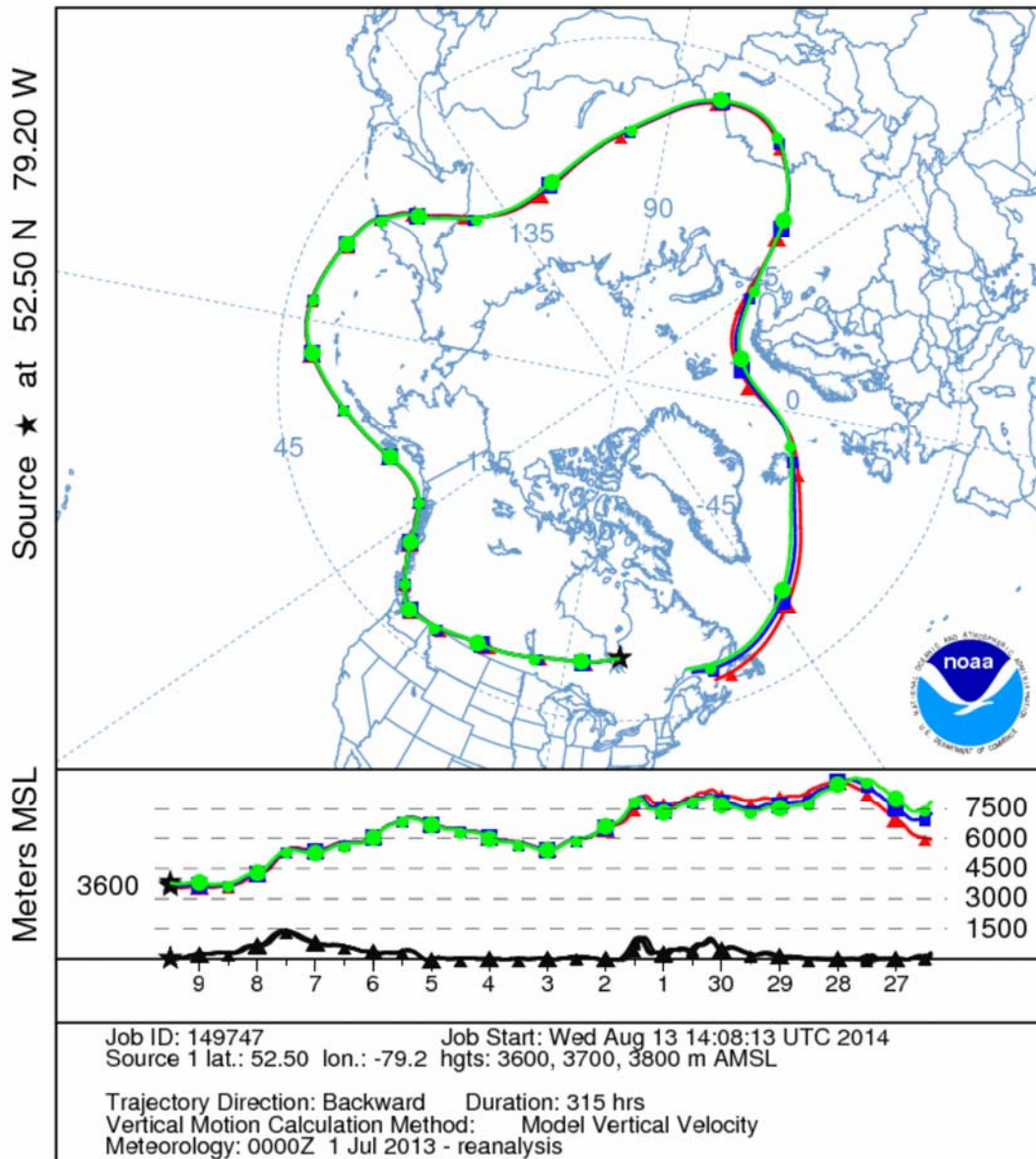
Fig. 19. Extension backward trajectories for those in Fig. 18 initiated on July 9, 2013 (12:00 UTC) at altitudes of 3600 m, 3700 m and 3800 m a.s.l. above James Bay where the three trajectories in Fig. 18 almost coincide. The coherence of the trajectory bundle is exceptional. The maximum altitude reached is about 9 km.
