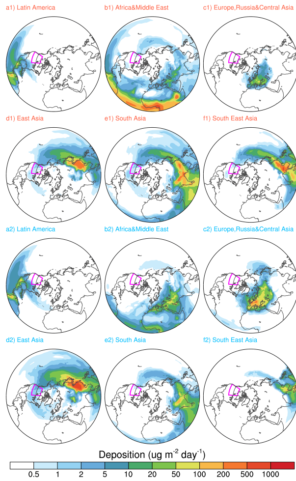
Fig. S10. Same as Fig. S6 but for BC deposition.
