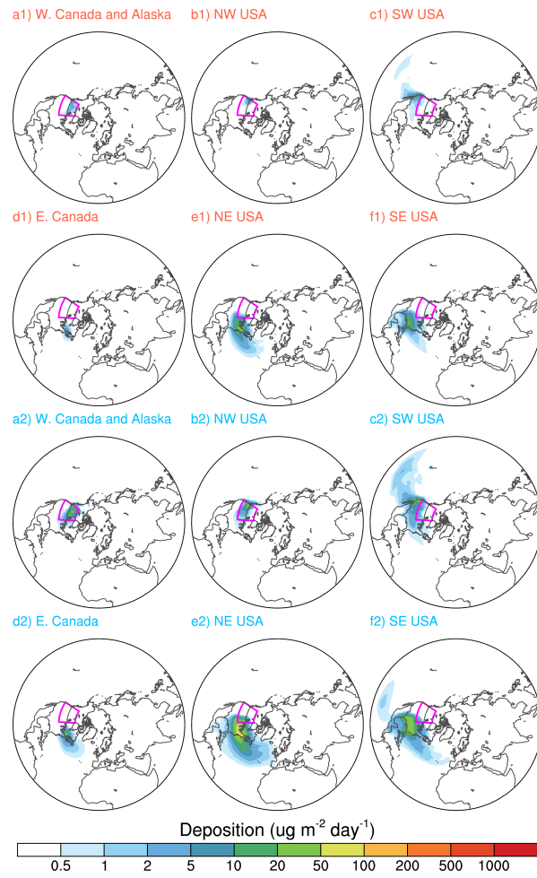
Fig. S11. Same as Fig. S7 but for BC deposition.
