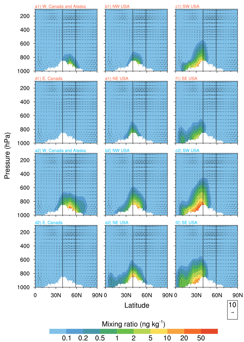
Fig. S9. Latitude-height cross-section of JFM mean BC mass mixing ratios (in \text{ng kg}^{-1} , colors) over the longitude band 93.75\text{--}123.75^\circ \text{W} , originating from the BB (a1–f1) and the FF (a2–f2) sectors in six tagged local source regions. The latitudinal boundaries of Western North America ( 39.8\text{--}58.8^\circ \text{N} ) are marked with black vertical lines.
