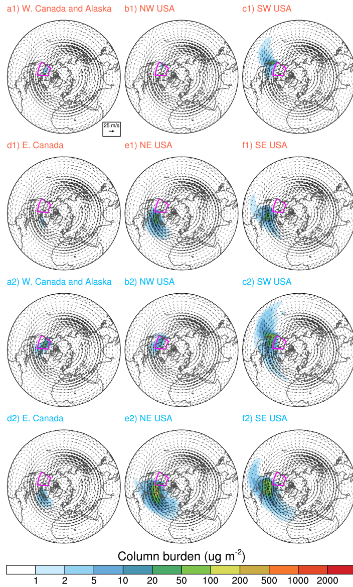
Fig. S7. Same as Fig. S6 but for six local source regions within North America.
