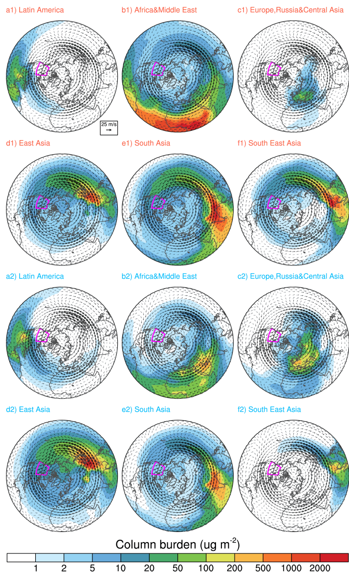
Fig. S6. Spatial distributions of the JFM mean BC total column burden (in \mu\text{g m}^{-2} , colors), originating from the BB (a1–f1) and the FF (a2–f2) sectors in six tagged source regions that are distant from the receptor region of interest, Western North America ( 39.8\text{--}58.8^\circ\text{ N} , 93.75\text{--}123.75^\circ\text{ W} ), which is marked with magenta outline.
