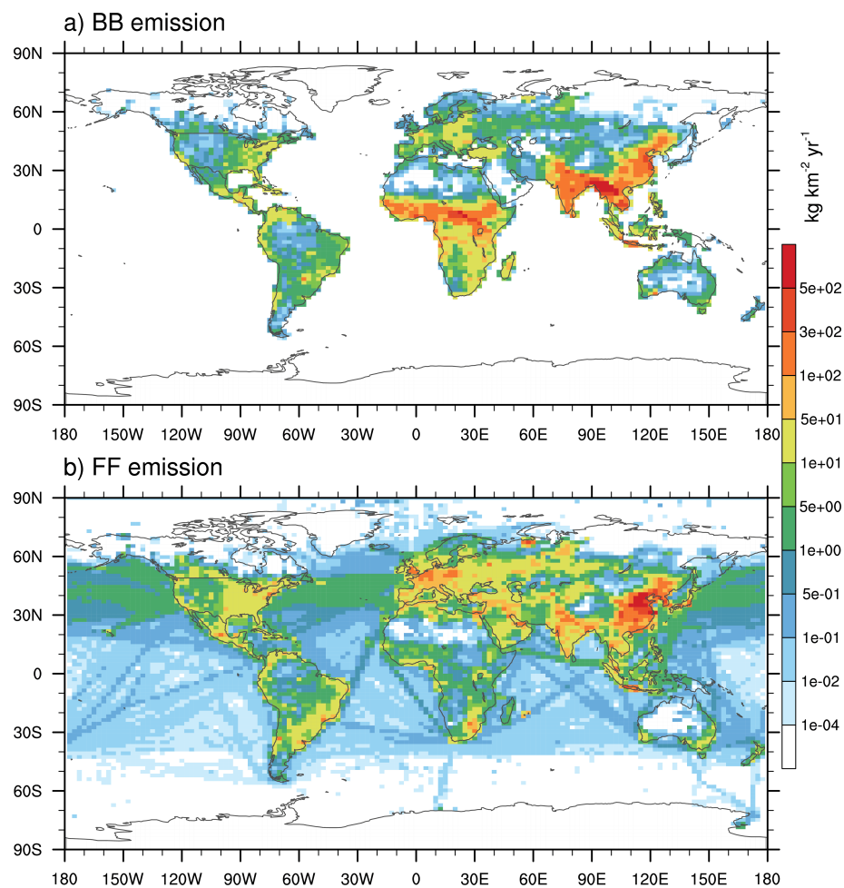
Fig. S2. Global distribution of JFM mean BC emissions ( \text{kg km}^{-2} \text{yr}^{-1} ) from the (a) BB and (b) FF sectors for the emission inventory of year 2010 used in this study.
