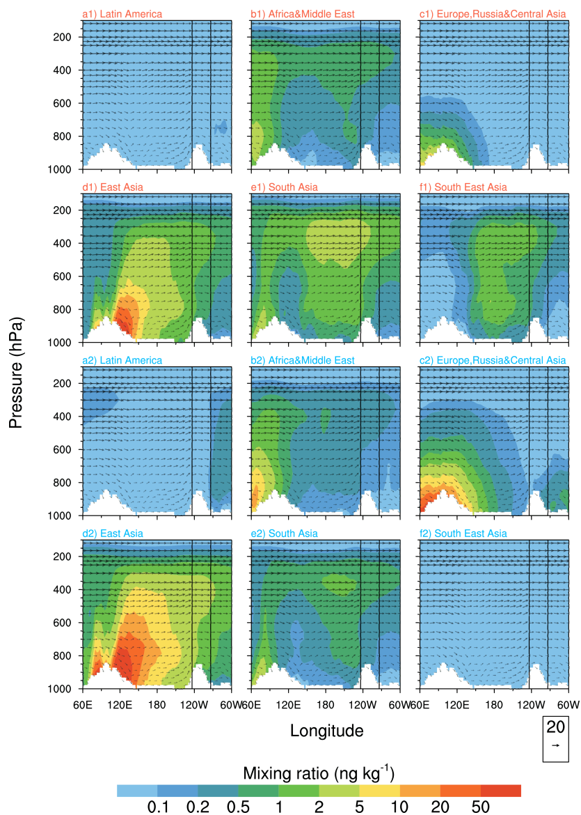
Fig. S8. Longitude-height cross-section of JFM mean BC mass mixing ratios (in \text{ng kg}^{-1} , colors) over the latitude band 39.8\text{--}58.8^\circ \text{N} , originating from the BB (a1–f1) and the FF (a2–f2) sectors in six tagged source regions that are distant from the receptor region. The longitudinal boundaries of Western North America ( 93.75\text{--}123.75^\circ \text{W} ) are marked with black vertical lines.
