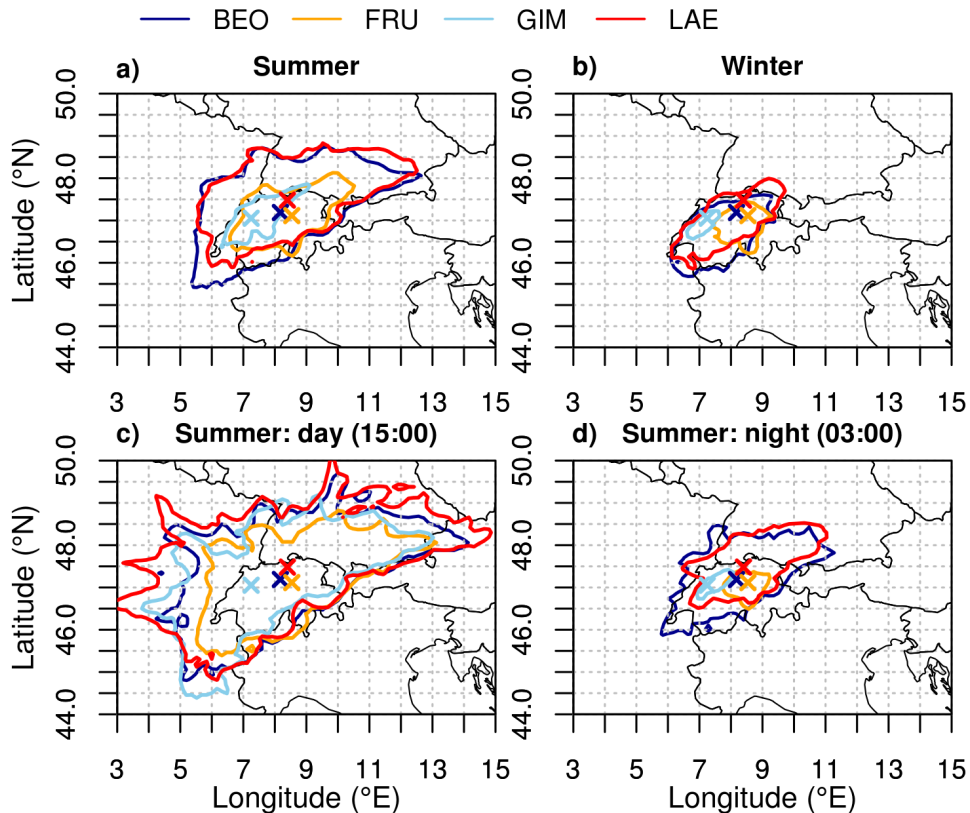
Figure 12. Area of surface influence (Eq. 5) defined as the isoline at the site-dependent value \tau_{s50} encompassing 50 % percent of the total mean surface sensitivities. Lines are color-coded according to measurement site—Beromünster: dark blue, Frübüel: orange, Gimmiz: light blue, Läger-Hochwacht: red. (a) Summer (June–August, 2013), (b) winter (December 2013–February 2014), and (c) and (d) summer (June–August, 2013) in the afternoon (15:00 UTC) and at nighttime (03:00 UTC), respectively. Local time is Central European Time (CET or UTC+1).
