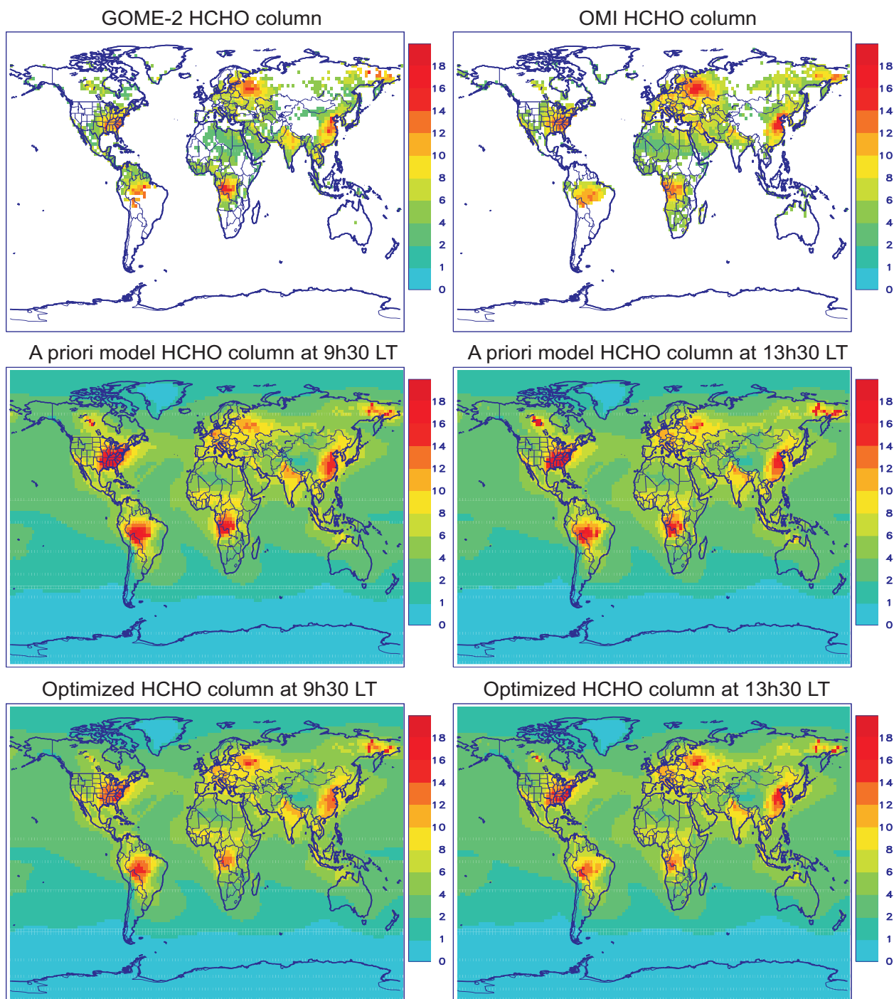
Fig. 6. Observed (upper panels) HCHO columns by GOME-2 and OMI instruments in July 2010. Simulated HCHO columns using IM-AGESv2 CTM at the overpass times of GOME-2 and OMI (middle panels), and optimized modelled columns derived from the inversions using GOME-2 data (left) and OMI columns (right). The columns are expressed in 10^{15} molec. cm^{-2} .
