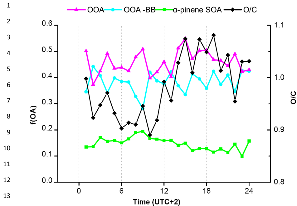
Fig. 9. Diurnal variability of the three major classes of organic aerosol obtained from the PMF analysis, along with the O/C ratio, during the period 28 August to 2 September. The quantity f(OA) represents the fractions of individual organic compounds of the total organic mass, where OA refers to OOA, OOA-BB or \alpha -pinene SOA.
