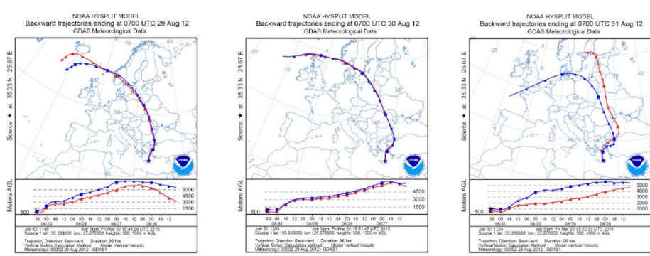
Fig. 3. Four-day back trajectories for air masses arriving at Finokalia on 29, 30 and 31 August, 2012.
